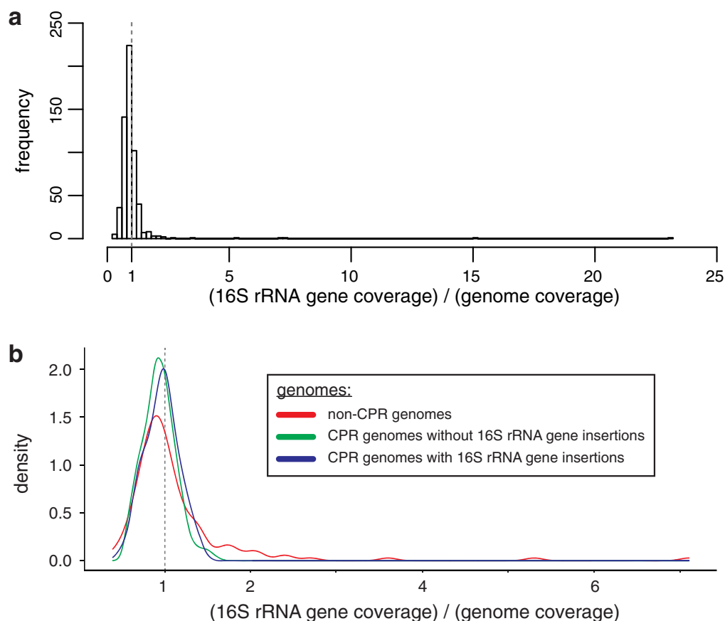
Extended Data Figure 5 | 16S rRNA gene copy number estimations for genomes reconstructed from groundwater metagenomics. a, b, 16S rRNA gene copy number was estimated for all draft CPR genomes and genome bins for organisms outside the CPR. This was achieved by comparing the coverage of 16S rRNA gene regions to the coverage of the rest of the genome.
