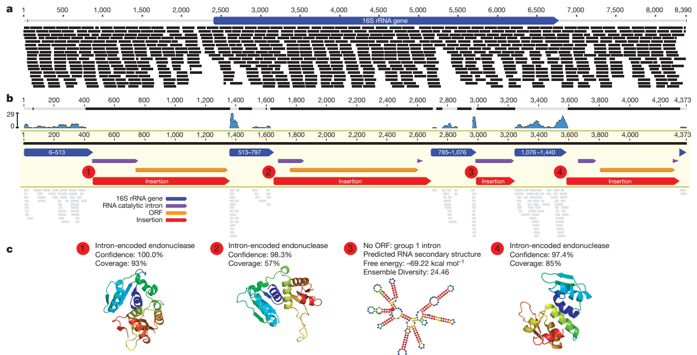
Figure 3 | Intron-encoding 16S rRNA gene from complete Microgenomates genome. a , Stringent mapping of paired-read metagenome sequences confirms the assembly. b , 16S rRNA encoding regions, but not insertions, are covered by perfectly matched metatranscriptome sequences. The absence of RNA sequences for insertions indicates that they are introns. Shown are regions corresponding to Escherichia coli K12 gene positions, RNA catalytic introns,
