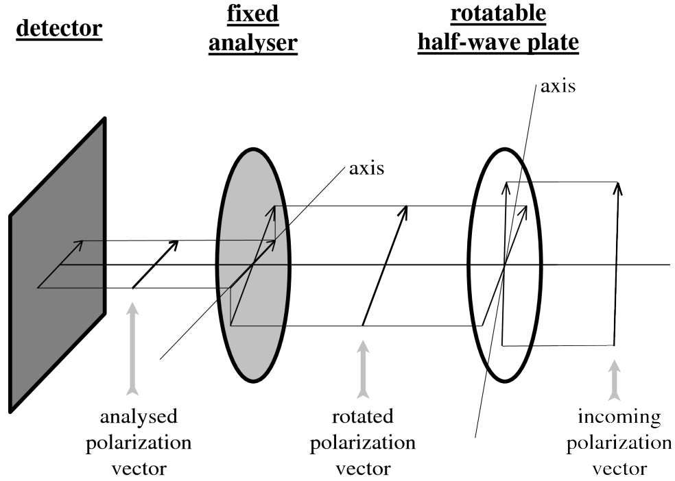
Figure 2.2: The main optical components in a typical single-beam imaging polarimeter such as POL-2 (taken from SUN/223).
