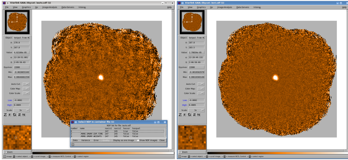
Figure 4.2: Left: I map, i: auto.sdf , as produced by the automask on the first pass of pol2map . Right: Final I map, i: ext.sdf , as viewed with GAIA. The flatter background is due to the increase in pca.pcathresh .
