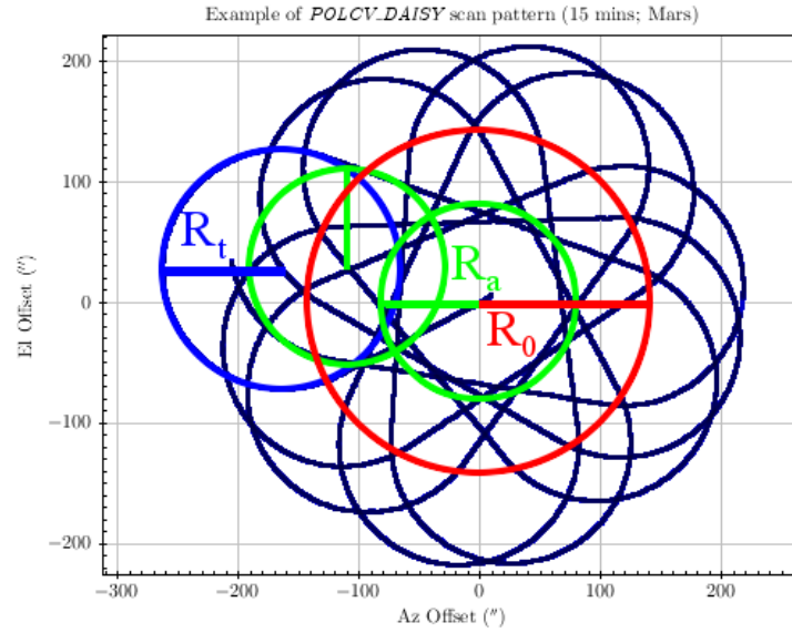
Figure 2.7: Detail of POLCV_Daisy. R_0 is the map pattern radius, R_t the turn radius, and R_a is the nominal avoidance radius. For more details see Table 2.1.
