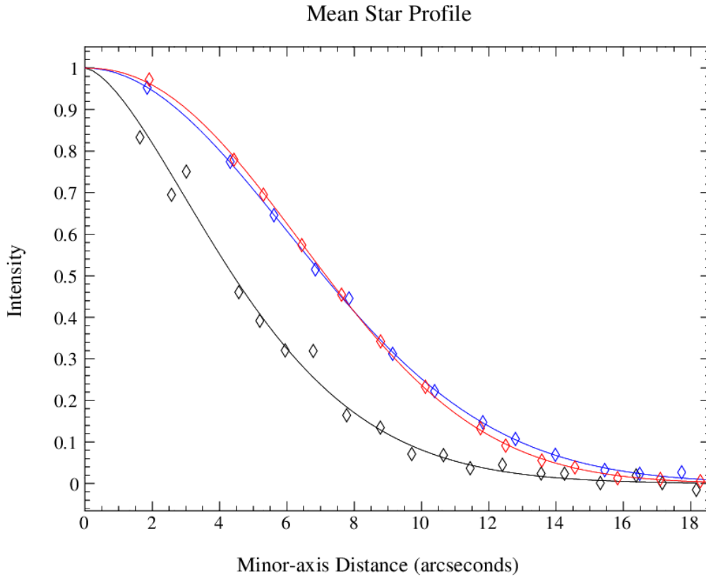
Figure 6.5: The mean radial total-intensity profile of 3C 279 determined from 25 POL-2 observations. The black curve shows the 450 \mu\text{m} profile produced using SM00TH450 = NO (the default), the red curve shows the 450 \mu\text{m} profile produced using SM00TH450 = YES and the blue curve shows the 850 \mu\text{m} profile.
