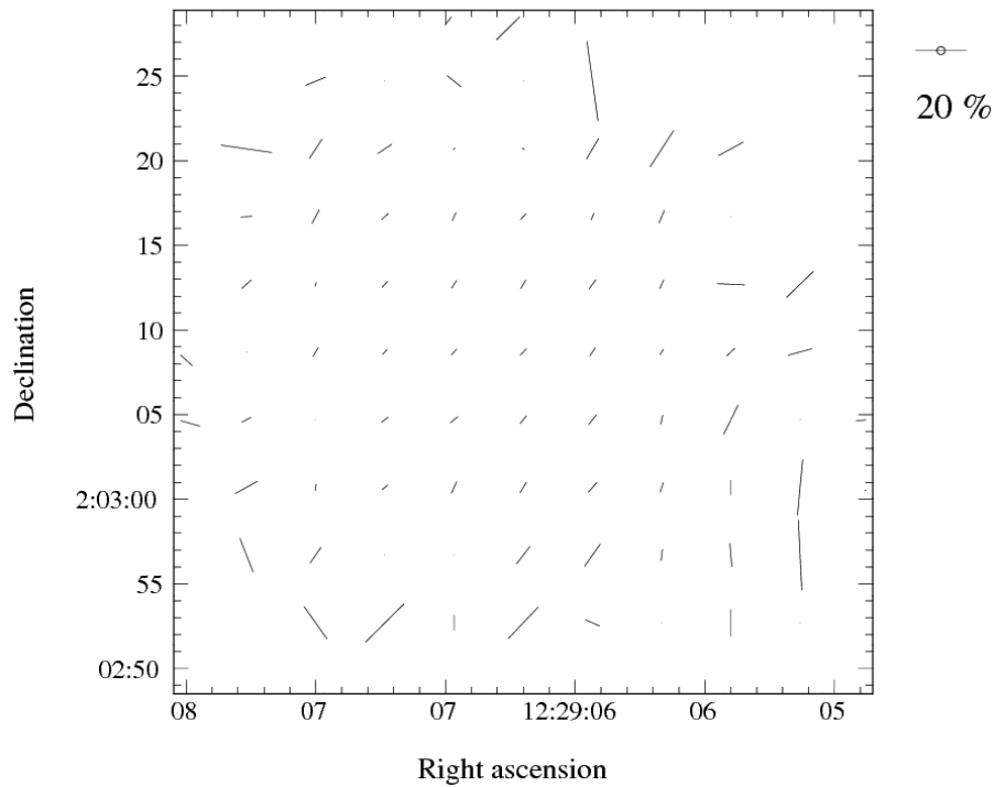
Figure 5.4: Results of Example 1: Producing a vector map with no background using polplot.
