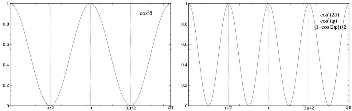
Figure 2.3: Left: If there was a single rotating analyser this would be the resulting curve of the power transmitted of the linearly polarised component. Right: With the HWP, the linearly polarised component is rotated at twice the speed. It may be useful to remind the reader of the trigonometric identity: \cos^2 x = 0.5(1 + \cos(2x))
