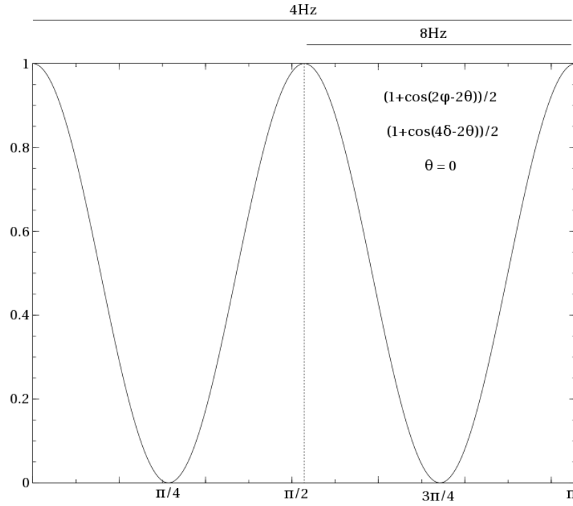
Figure 2.4: The incoming polarised radiation (with a polarised angle, \theta , of zero) is attenuated by the HWP. The HWP rotates at 2Hz (through 2\pi ) so we see the signal is modulated at 8Hz as the instrument scans at 8''/\text{s} .
