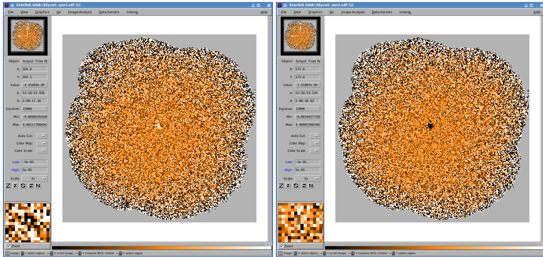
Figure 4.3: Left: Q map, q: ext.sdf . Right: U map u: ext.sdf , as viewed with GAIA.
