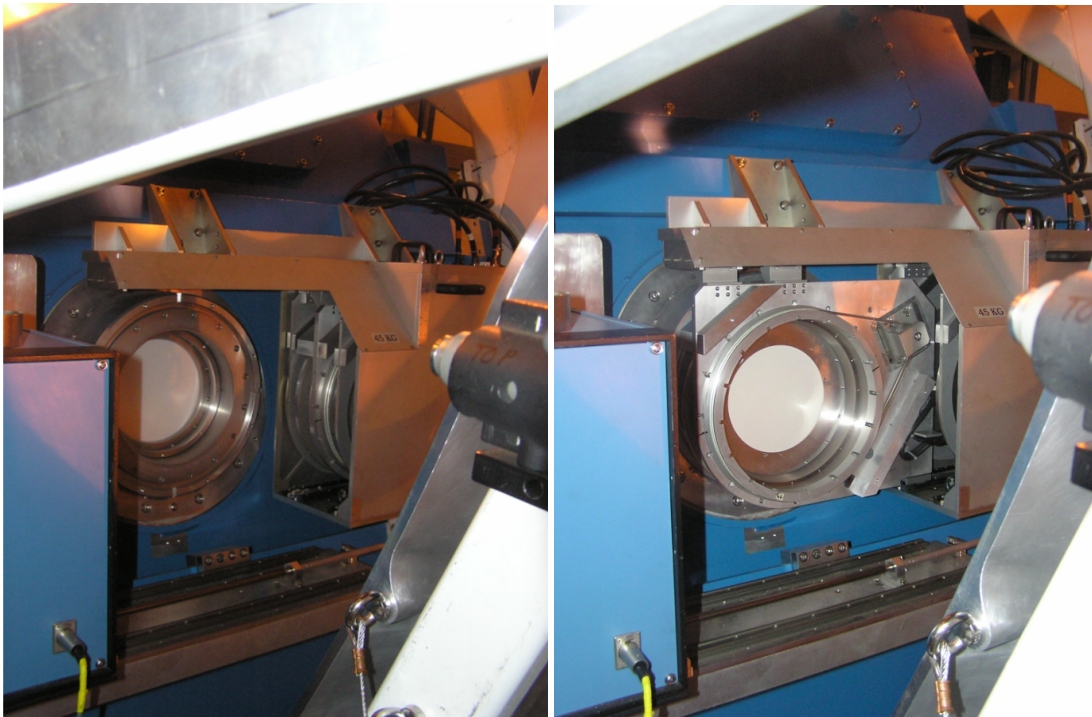
Figure 2.1: POL-2 mounted on the front of SCUBA-2. The left image shows the SCUBA-2 window. The right image shows the components of POL-2 inserted in front of the SCUBA-2 window: the calibrator grid, rotating half-wave-plate (HWP) and the analyser grid. The calibrator grid is only inserted for test purposes.
