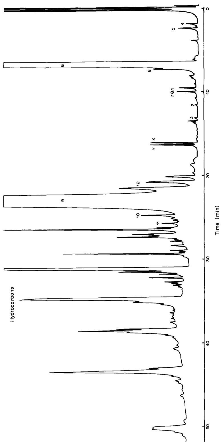
Fig. 1. GC trace of the volatiles from I. purpureus run on FFAP (column c) 90°, programmed at 3°C/min to 230°C. The numbers refer to Table 1.
