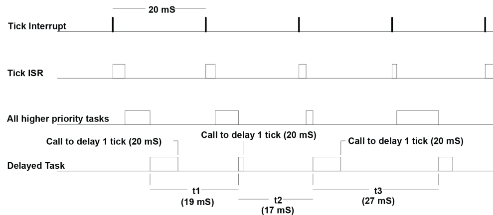
Figure - Figure 2.25 Delaying a task for one tick (Case 1)
