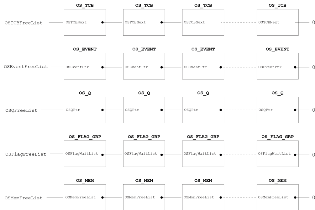
Figure - Figure 3.12 Free Pools
