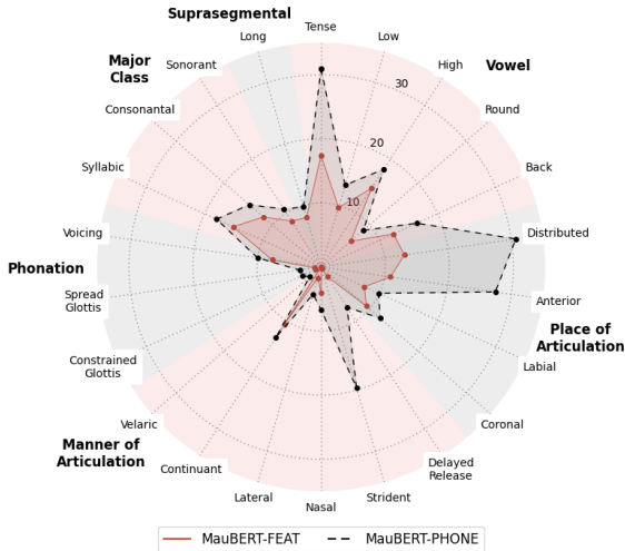
Figure 2: Classification errors across articulatory features ( \downarrow ) for both MAUBERT variants on the 5 development languages. All values are in %.
