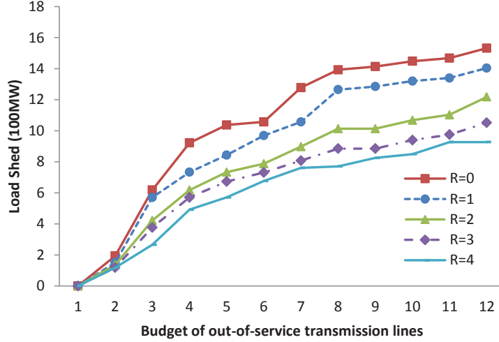
Figure 3: Load shed with different protection budgets
