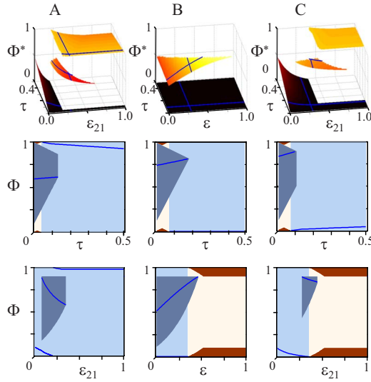
FIG. 2. (Color online) (Un-)stable states for two inhibitory pulse-coupled oscillators with delay. (A) Asymmetric case with \varepsilon_{12}=0.2 . (B) Symmetric case: \varepsilon_{21}=\varepsilon_{12}=\varepsilon . (C) Asymmetric coupling with \varepsilon_{12}=0.4 . Asymptotically stable fixed points \Phi^* of the return map as a function of \tau and \varepsilon_{21} [cf. Fig. 1 now with \varepsilon_{21}=0.3 (middle row) and \tau=0.1 (bottom row)].
