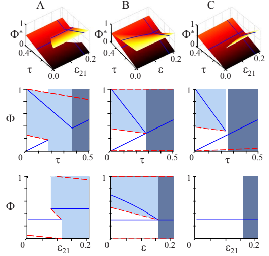
FIG. 1. (Color online) (Un-)stable states for two excitatory pulse-coupled oscillators with delay. (A) Asymmetric coupling with \varepsilon_{12}=0.1 . (B) Symmetric coupling with \varepsilon_{21}=\varepsilon_{12}=\varepsilon . (C) Asymmetric coupling with \varepsilon_{12}=0.2 . Top: asymptotically stable fixed points of the return map as a function of \tau and \varepsilon_{21} . Solid lines represent the cross sections shown in middle and bottom rows. Middle: stable (blue, solid line) and unstable (red, dashed line) fixed points and their attraction domains as a function of \tau for \varepsilon_{21}=0.18 . Bottom: same as the middle row as a function of coupling strength for \tau=0.3 .
