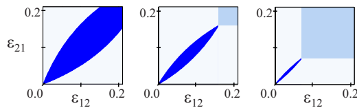
FIG. 3. (Color online) Number of stable states for two asymmetric pulse-coupled oscillators as function of excitatory coupling strengths \tau=\{0.2, 0.3, 0.4\} (from left to right). The darkest areas correspond to bistability contrasting monostability outside this area. The square in the right upper corner of the middle and right panels represents the region where the two oscillators are in antiphase.
