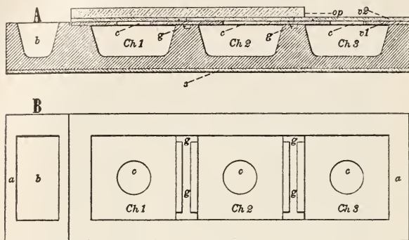
FIG. 282. Janet nest of porous material such as plaster, terra cotta, soft stone, etc. (Janet.) B, Seen from above with covers removed; A, in vertical section: a, block with three chambers; b, water chamber which is filled once or twice a week; Ch. 1, dark and very moist chamber; Ch. 2, dark and somewhat humid chamber inhabited by the ants; Ch. 3, dry chamber, exposed to light and containing the manger; g, communicating galleries in the walls separating the chambers. v 1 , large plate of glass covering all the chambers, pierced with a hole (c) over the center of each chamber; v 2 , three separate pieces of glass which close the openings in the large plate; op, opaque cover (felt, cardboard or plaster) serving to darken chambers 1 and 2; s, plate of glass placed under the nest to prevent the moisture of the nest from reaching the table on which it stands.
