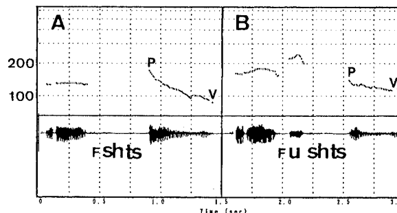
Figure 2 F0 contours of test word F'ST with and without the devoicing of accented syllable. Panel A and B correspond to the same panels in figure 1. Frequency scaling is logarithmic.
