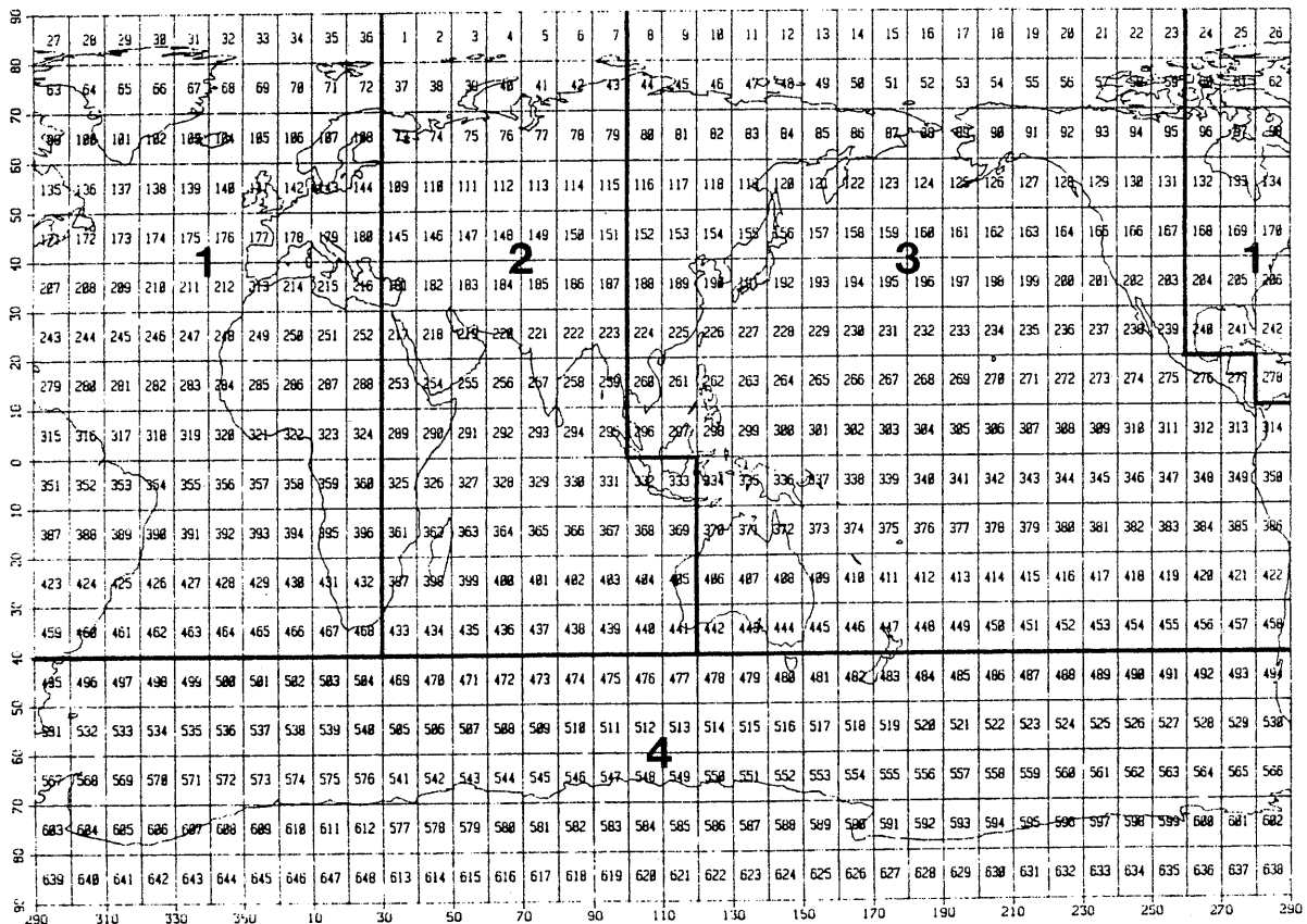
Figure 3-2. Basins and 10° boxes.
