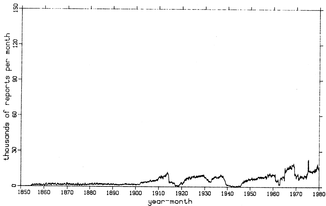
Figure 3-4. Basin 2 INDIAN reports after duplicate elimination.
