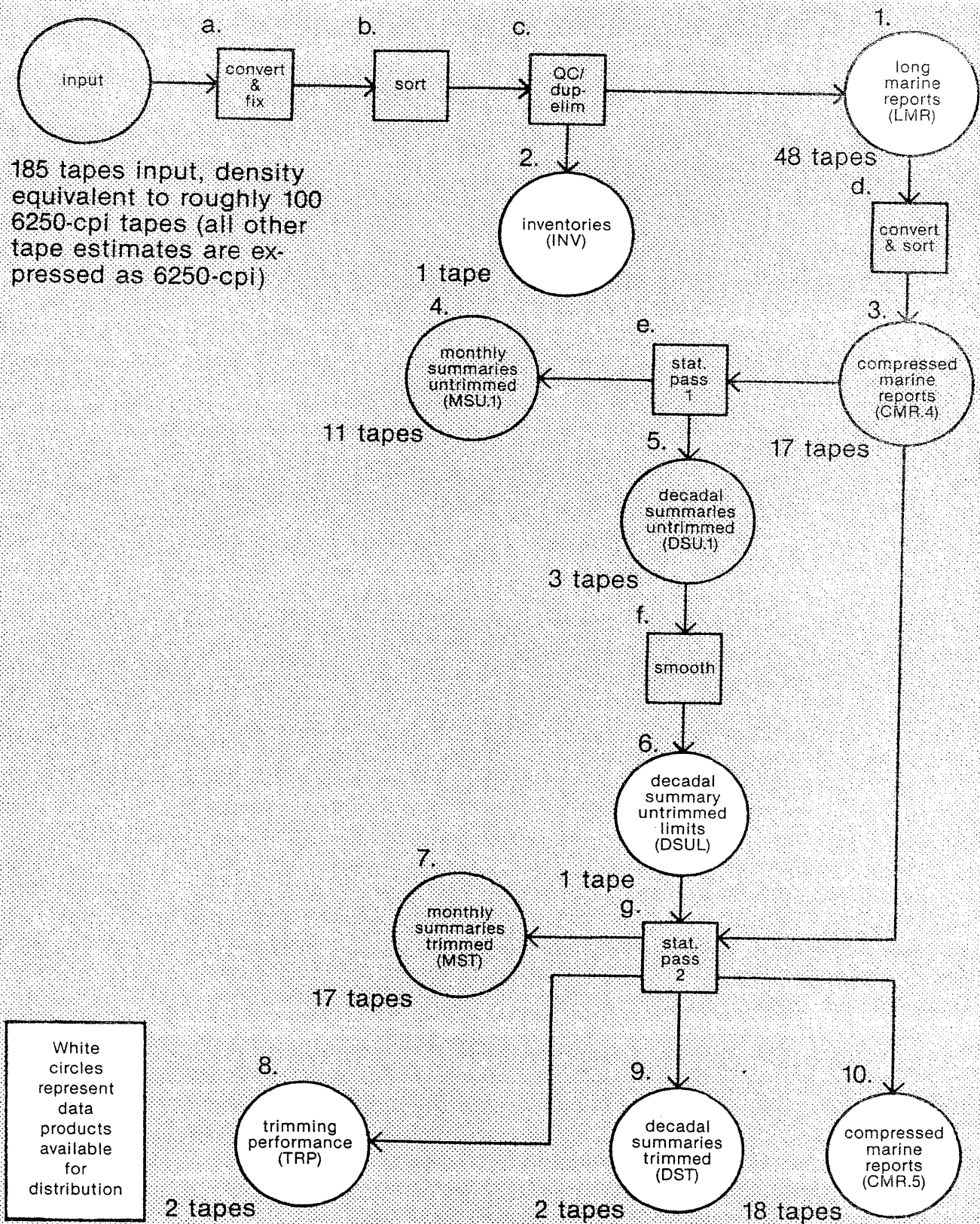
Flowchart 1. Primary Processing. Data products are shown as circles and processes are shown as squares. (Note: product 3 has been superseded by product 10, and products 4, 5, and 7 have been superseded by secondary products 12-18 shown on Flowchart 2.)
