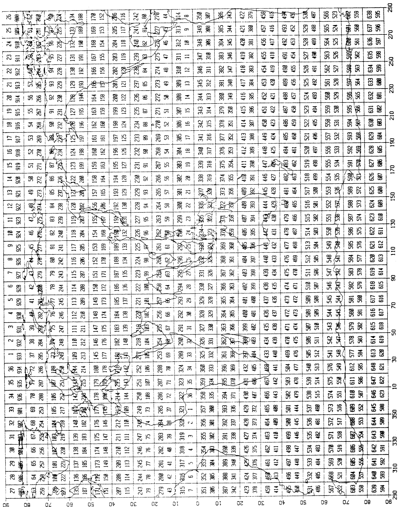
Figure G1-1. 10° boxes (larger numerals) over Marsden Squares (smaller numerals).
