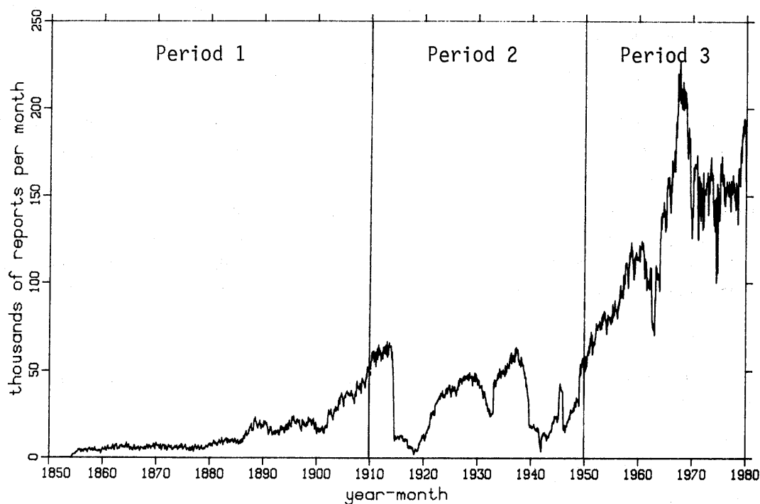
Figure C1-1. Global reports after duplicate elimination, divided into periods that separate limits were established for using untrimmed data.
