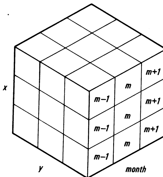
Figure C2-2. Decadal cube example.
