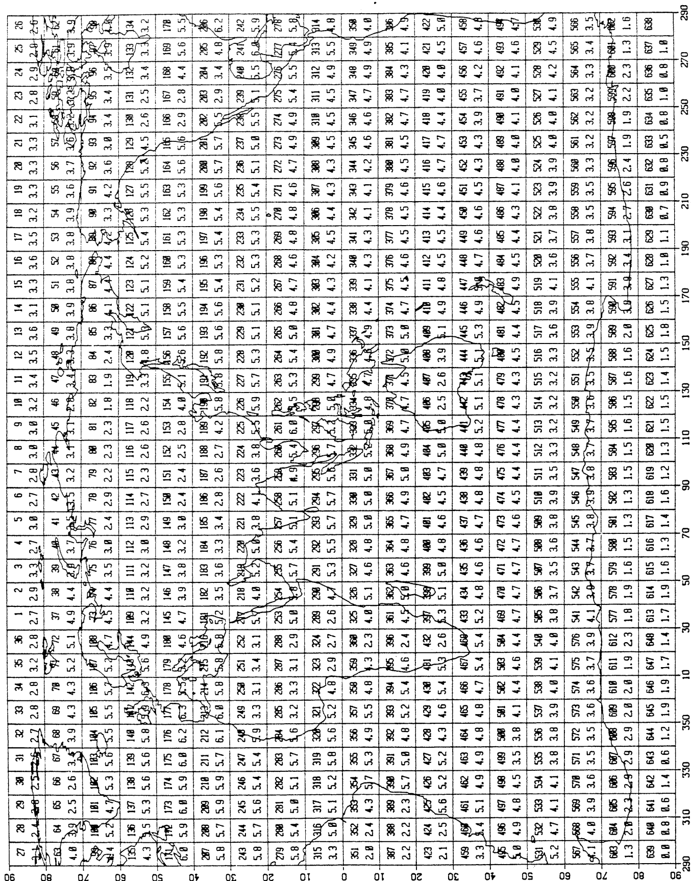
Figure 3-8. 10° boxes (smaller numerals) over log 10 of reports 1854-1979 (larger numerals).
