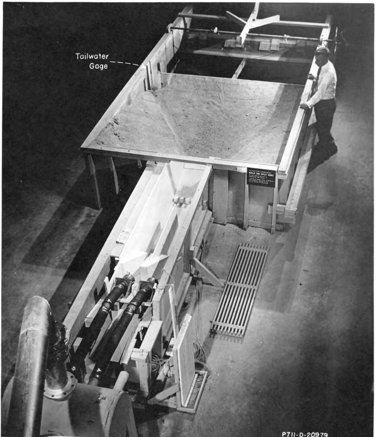
Recommended Permanent Outlet Works Basin
