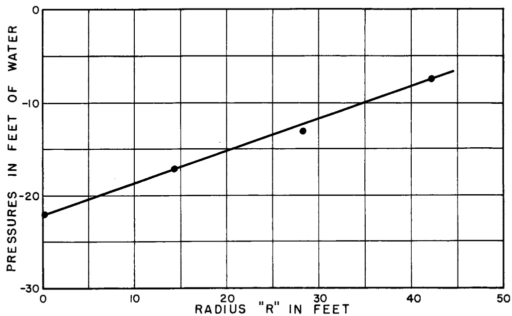
SECTION ON C OF SCHEME #2
