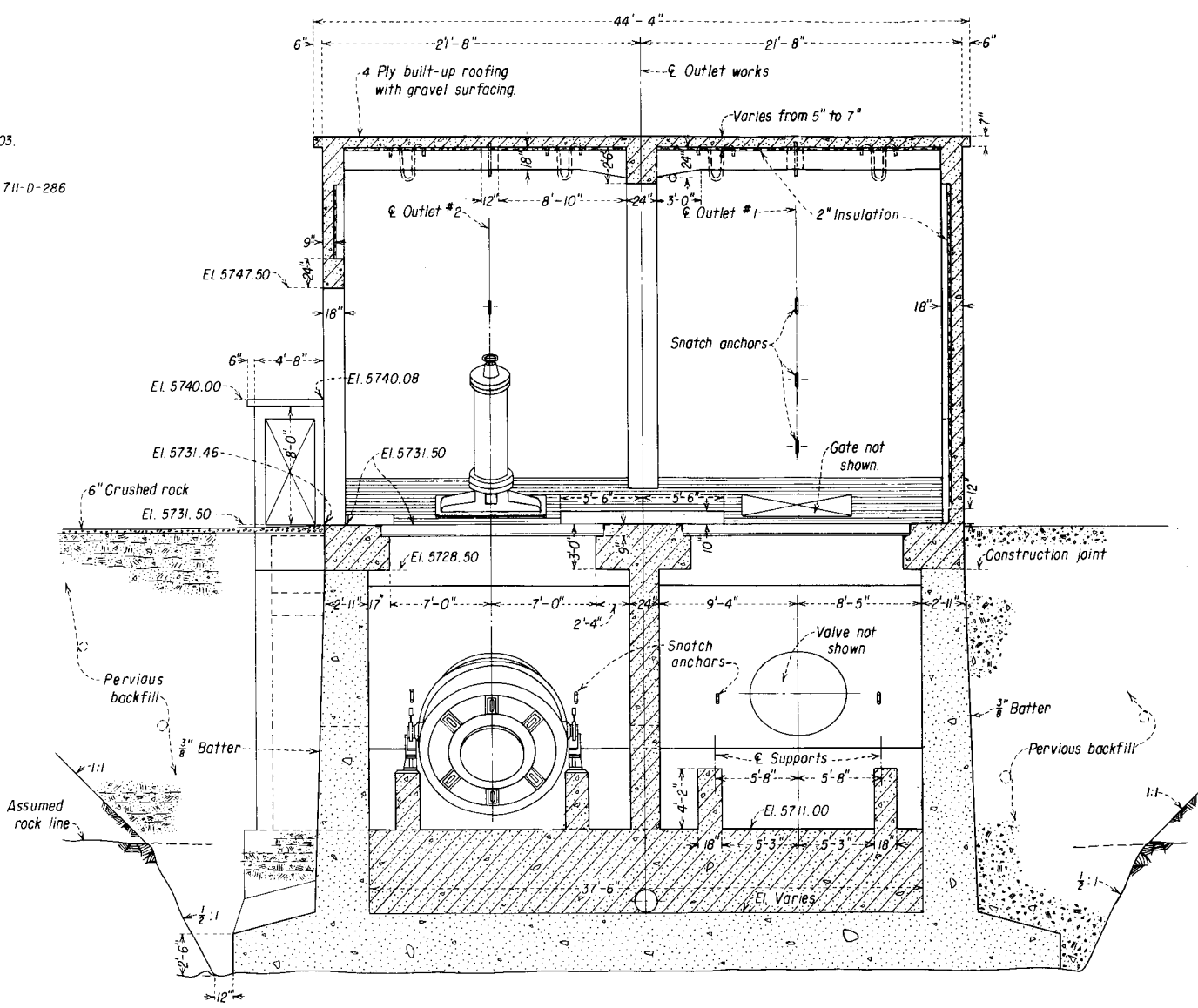
SECTION F-F
