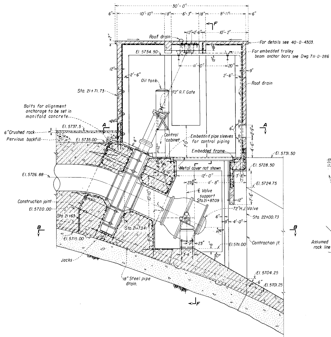
SECTION E-E
