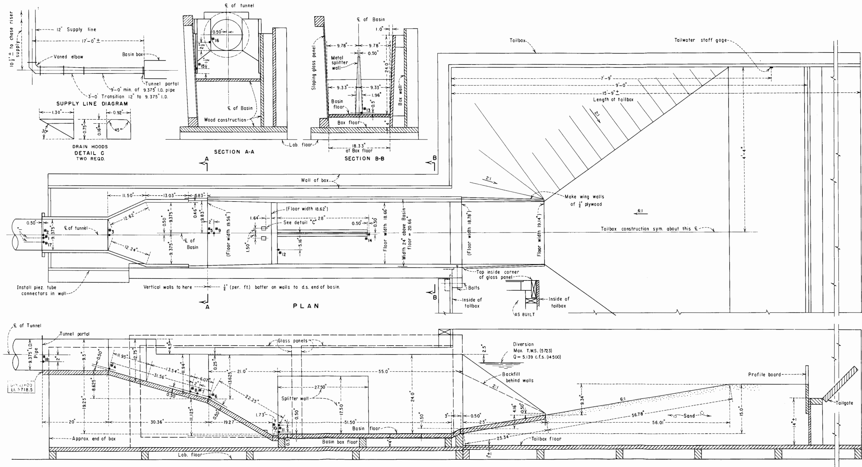
NAVAJO DAM STILLING BASIN LAYOUT FOR DIVERSION STUDY 1:24 SCALE MODEL
