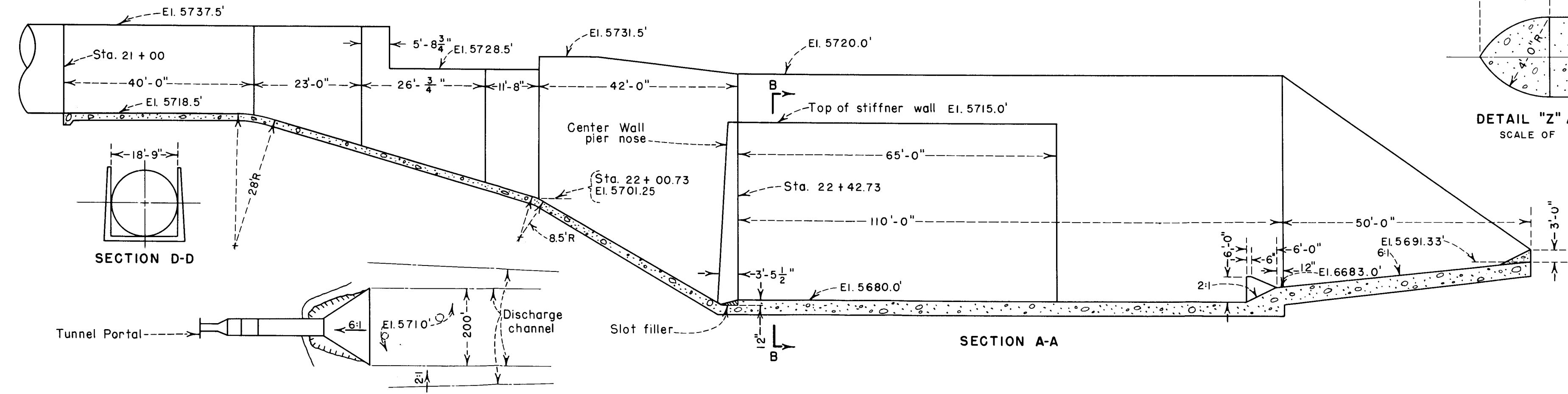
NAVAJO DAM DIVERSION STILLING BASIN SCHEME 2 1:24 SCALE MODEL
