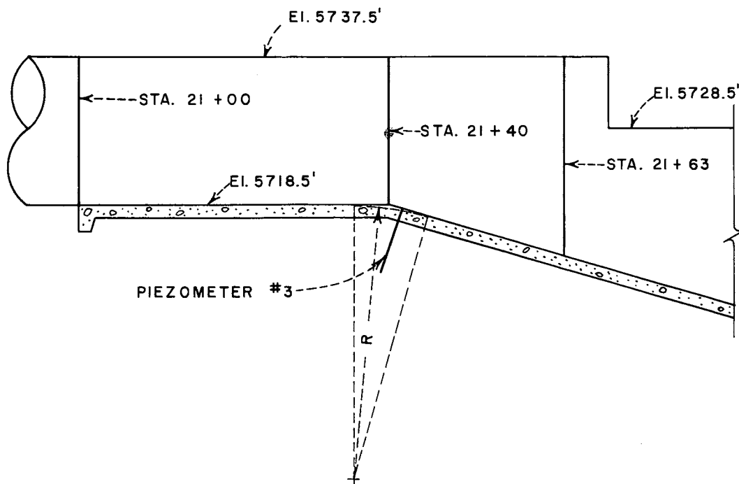
SECTION ON C OF SCHEME #2
