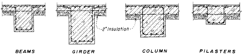
TYPICAL REINFORCEMENT DETAILS
