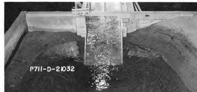
C. Valves 100% open, Head 54 feet, T.W. El. 5711
