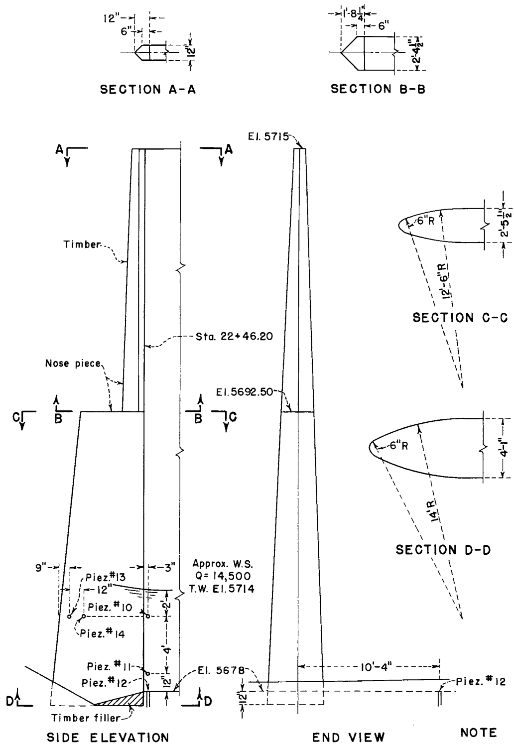
NAVAJO DAM RECOMMENDED CENTER WALL PIER NOSE DIVERSION 1:24 SCALE MODEL
