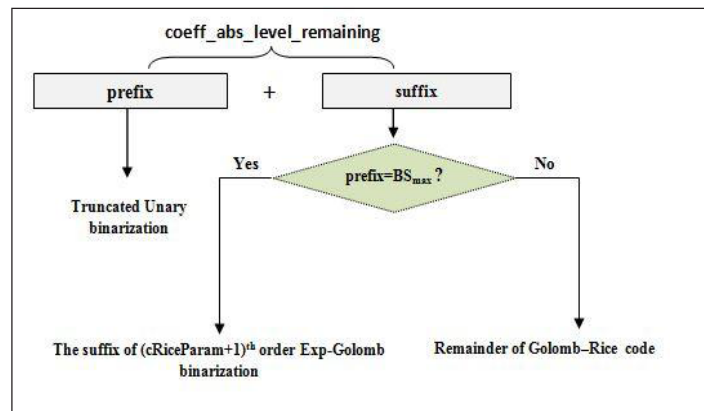
Figure 2. Binarization of coeff_abs_level_remaining : prefix is binarized with truncated unary code, and suffix is binarized either by Golomb–Rice code or by Exp-Golomb code
