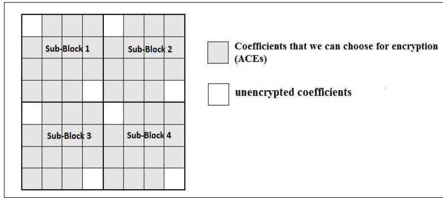
Figure 3. A transform unit TU_{8 \times 8} with 4 sub-block: gray cases mean selected coefficients for encryption
