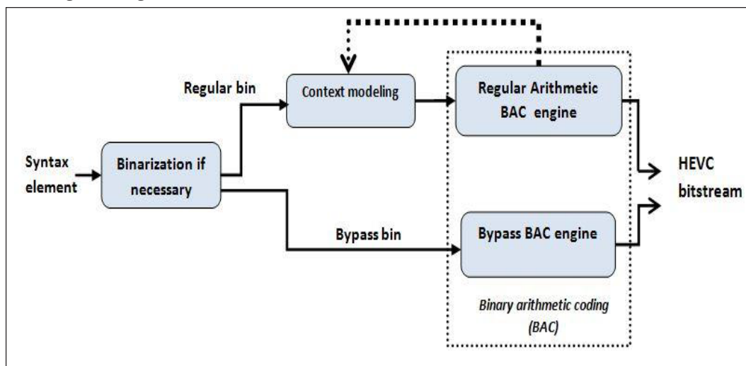
Figure 1. Bloc diagram of CABAC engine with three key operations: binarization, context modeling and binary arithmetic coding (BAC).
