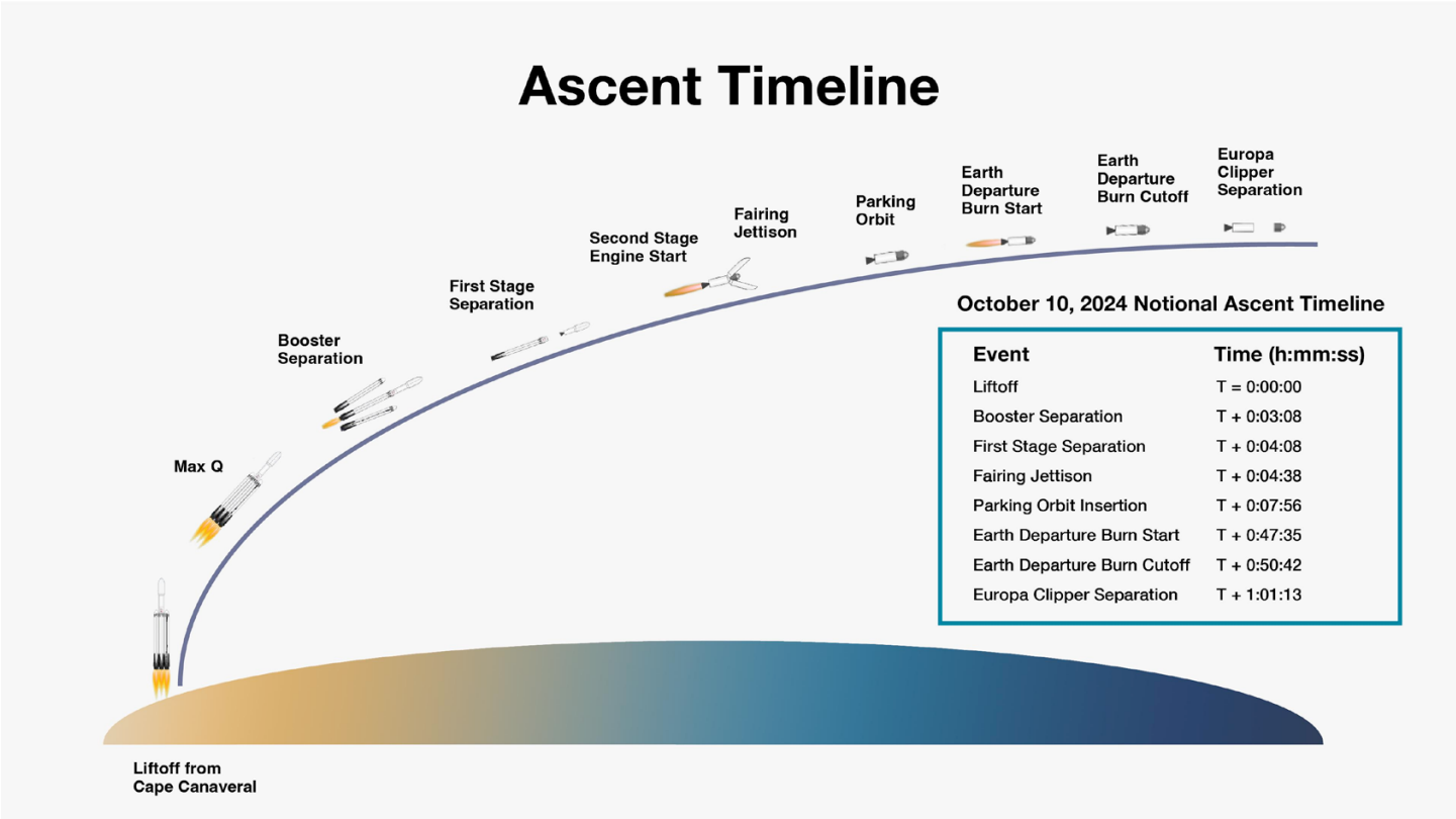
This is a sample ascent timeline for Oct. 10, 2024, the first day of Europa Clipper’s launch period. The actual times of milestones will differ slightly depending on the launch day. Credit: NASA/JPL-Caltech | Full Image
