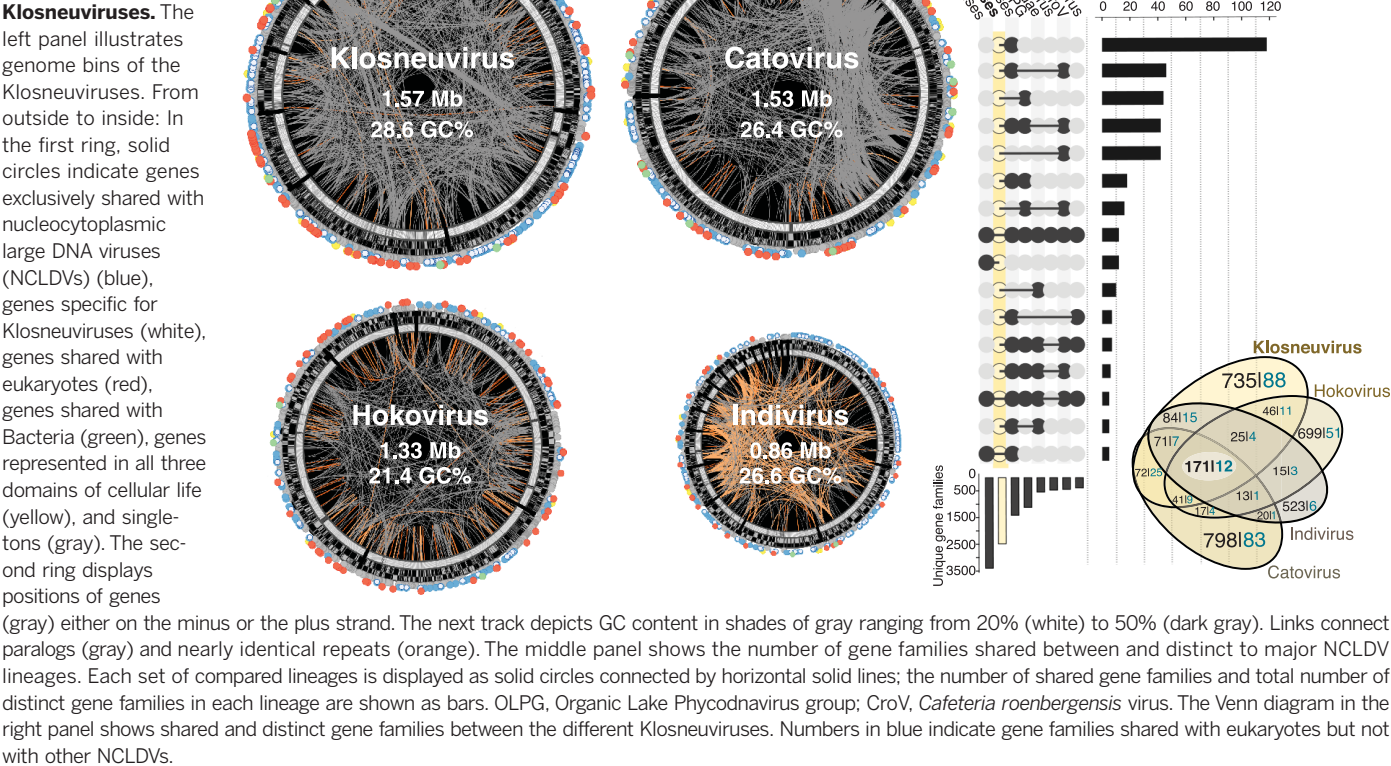
Fig. 1. Genome architecture and gene content of the Klosneuviruses.
