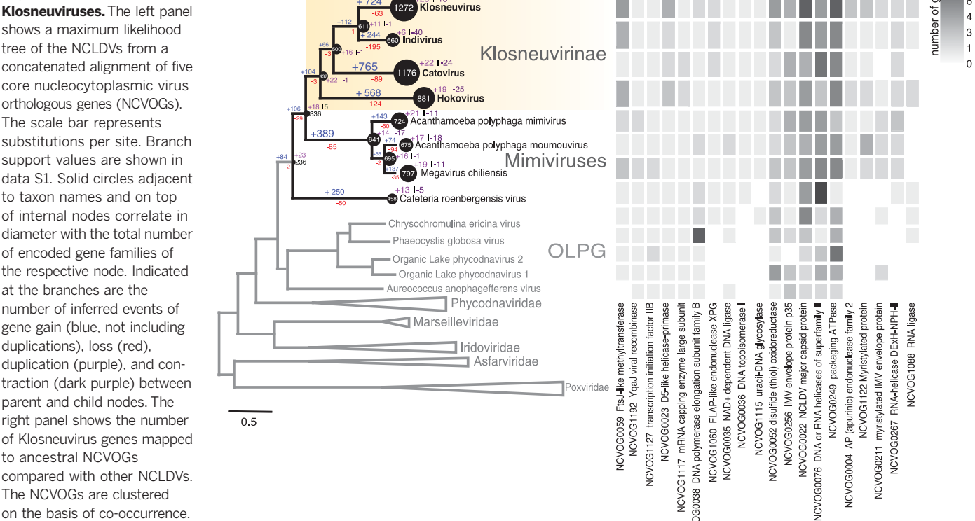
Fig. 2. Genome evolution and phylogenetic position of Klosneuviruses.
