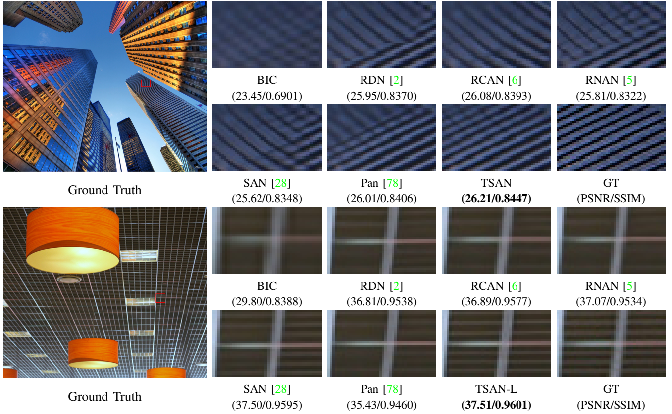
Fig. 11. Visual comparison between our TSAN-L and several heavy-weighted methods on img012 from Urban100 [7] and img044 from Urban100 [7] with scale \times 3 .
