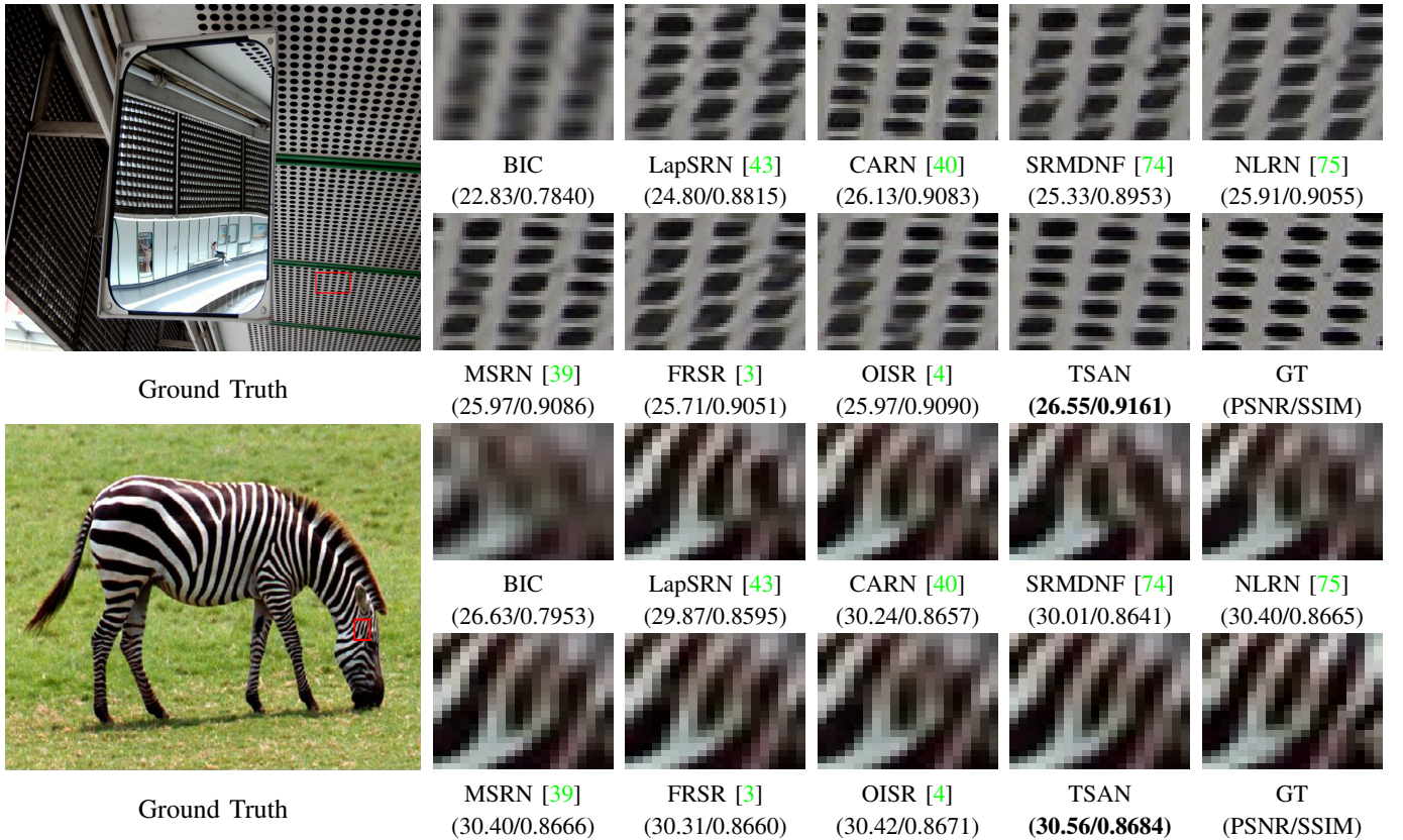
Fig. 8. Visual comparison between our TSAN and other light-weighted methods on img004 from Urban100 [7] and zebra from Set14 [72] with scale \times 3 .
