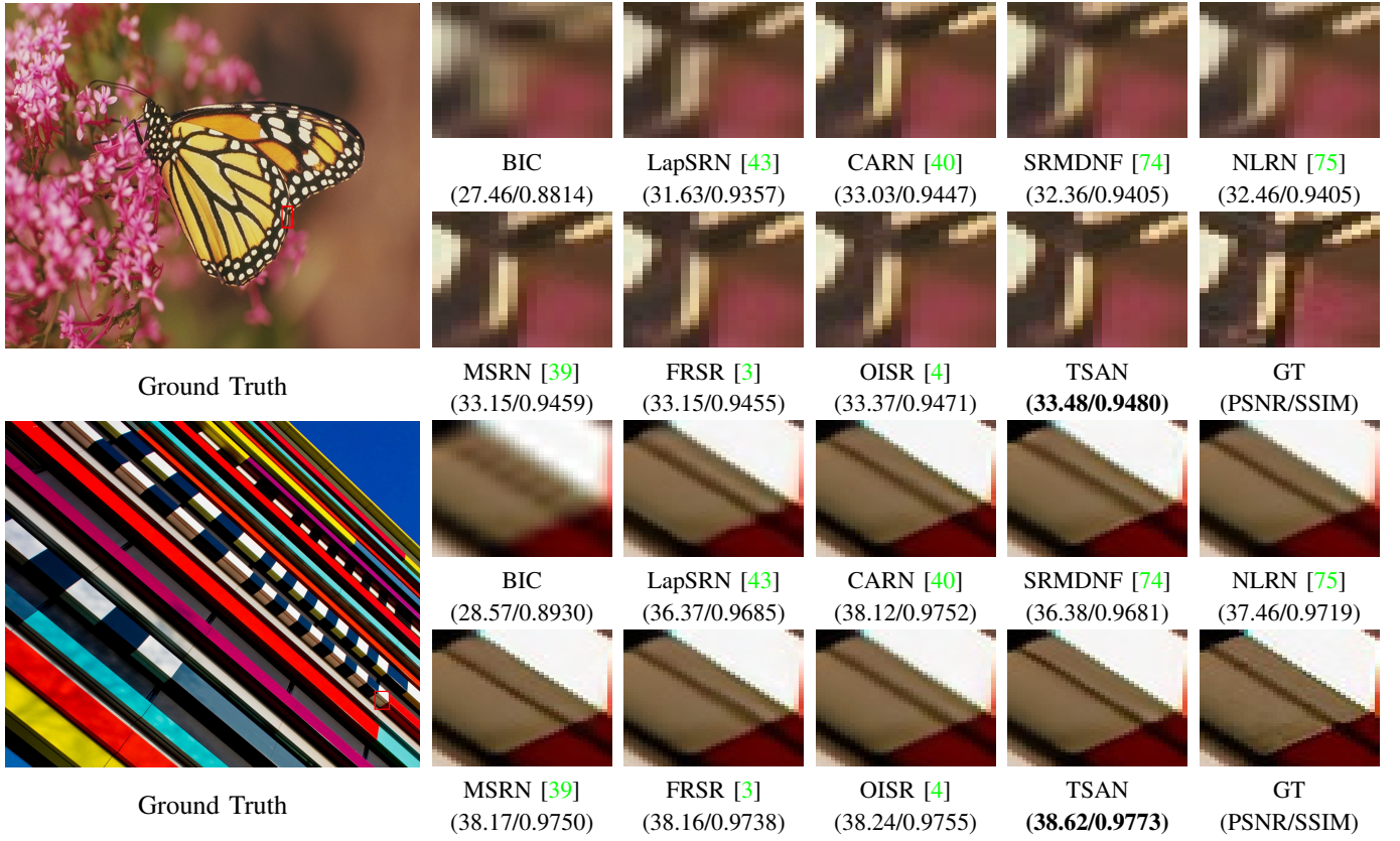
Fig. 9. Visual comparison between our TSAN and other light-weighted methods on monarch from Set14 [72] and img081 from Urban100 [7] with scale \times 4 .
