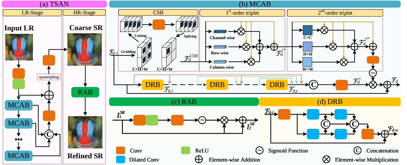
Fig. 2. (a) The overview of our proposed TSAN. TSAN is a two-stage network which reconstructs SR image in a coarse-to-fine manner. In LR-stage, MCABs are leveraged to extract attentive contextual features used for reconstructing an initial SR result. In HR-stage, RAB refines the initial SR result to a more fine-detailed one by exploring useful cues in HR space. (b) Our proposed Multi-Context Attentive Block (MCAB). (c) Our proposed Refined Attention Block (RAB). (d) the Dilated Residual Block (DRB).
