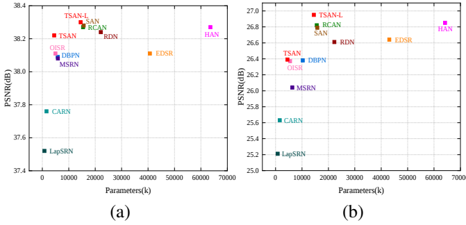
Fig. 6. PSNR performance versus number of parameters. (a) The results are evaluated on Set5 for a scale factor of \times 2 . (b) The results are evaluated on Urban100 for a scale factor of \times 4 . Our TSAN and TSAN-L has a better tradeoff between performance and model size.
