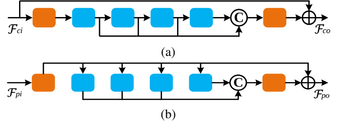
Fig. 3. (a) the cascaded structure; (b) the parallel structure.
