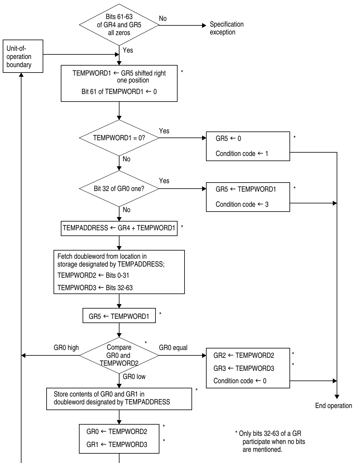
Figure 7-369. Execution of UPDATE TREE in the 24-Bit or 31-Bit Addressing Mode
