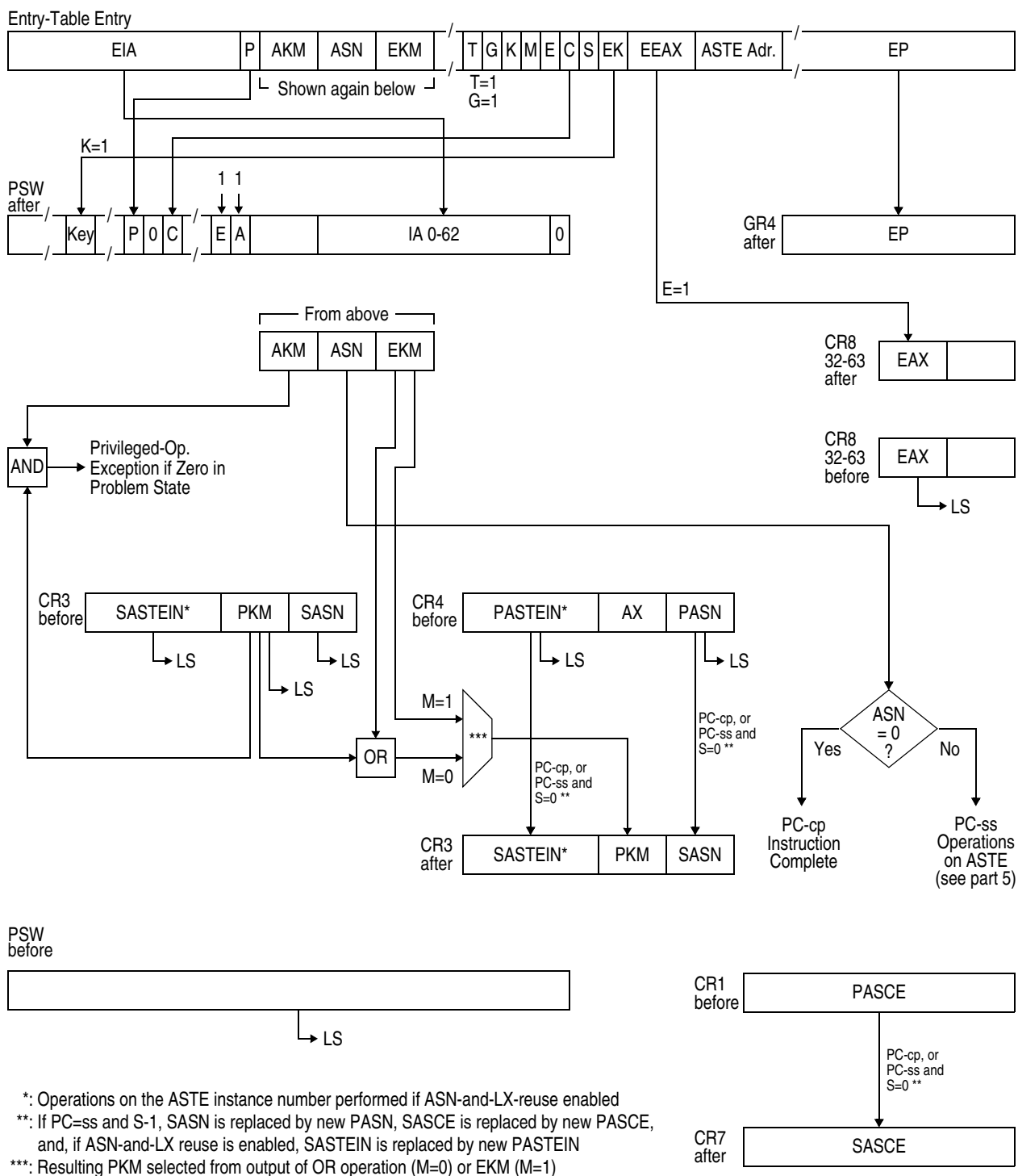
Figure 10-74. Execution of PROGRAM CALL (Part 3 of 5).
