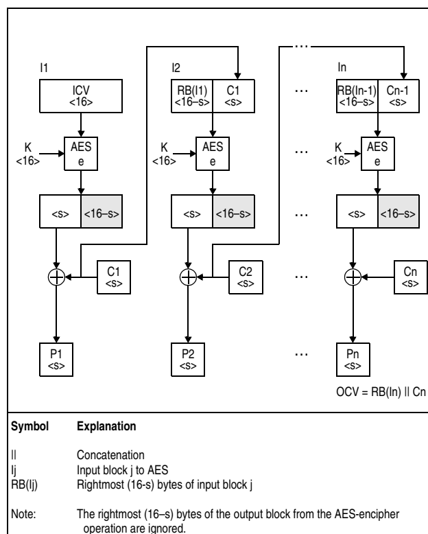
Figure 7-115. KMF-AES-128 Decipher Operation
