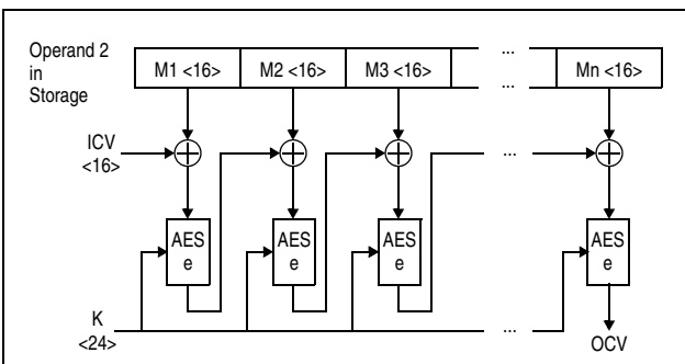
Figure 7-287. KMAC-AES-192
