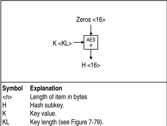
Figure 7-83. Encrypting the Hash Subkey
