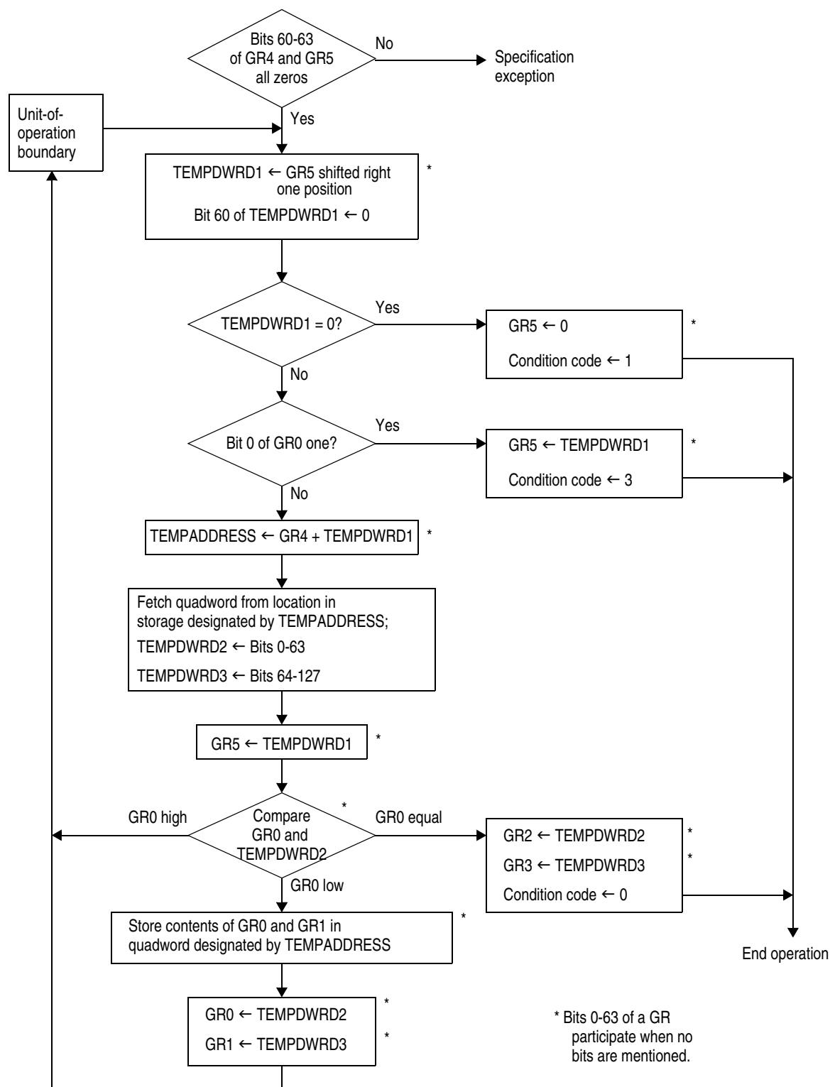
Figure 7-370. Execution of UPDATE TREE in the 64-Bit Addressing Mode
