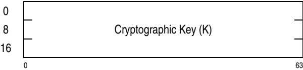
Figure 7-149. Parameter Block for KMCTR-AES-192
