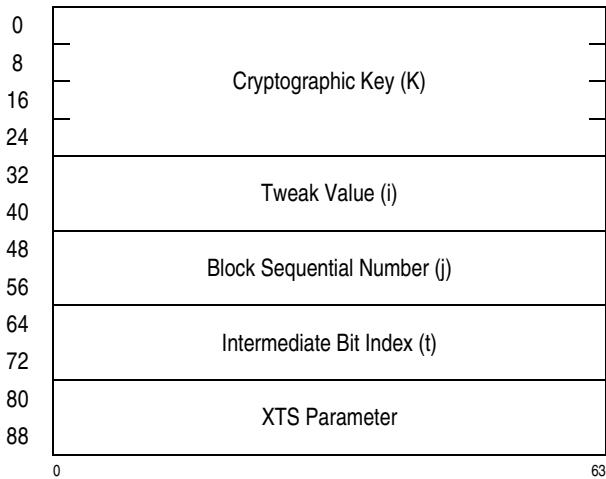
Figure 7-334. Parameter Block for PCC-Compute-XTS-Parameter-Using-AES-256
