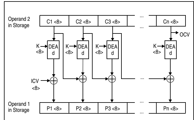
Figure 7-51. KMC DEA Decipher Operation Using 64-Bit Key
