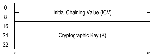
Figure 7-285. Parameter Block for KMAC-AES-192
