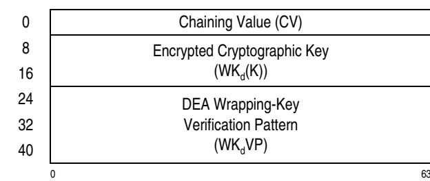
Figure 7-105. Parameter Block for KMF-Encrypted-TDEA-128
