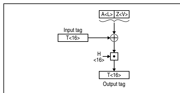
Figure 7-85. GHASH Processing of Last (Short) Block
