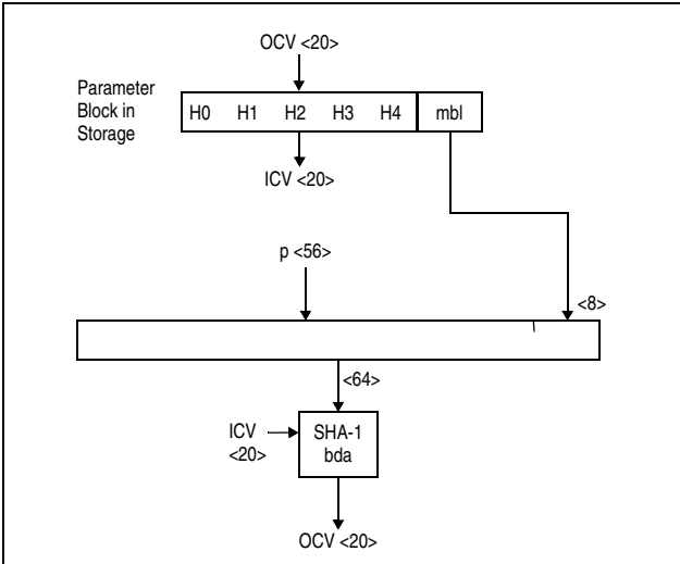
Figure 7-238. KLMD-SHA-1 Empty Block (L = 0)
