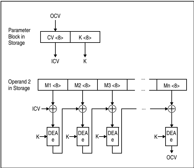
Figure 7-275. MAC Computation Using 64-bit DEA Key
