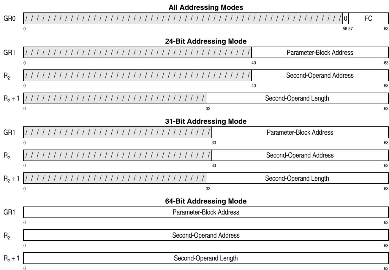
Figure 7-266. General Register Assignment for KMAC
