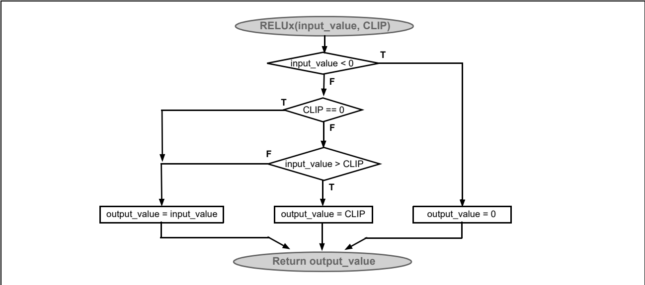
Figure 26-58. RELUx() operation
