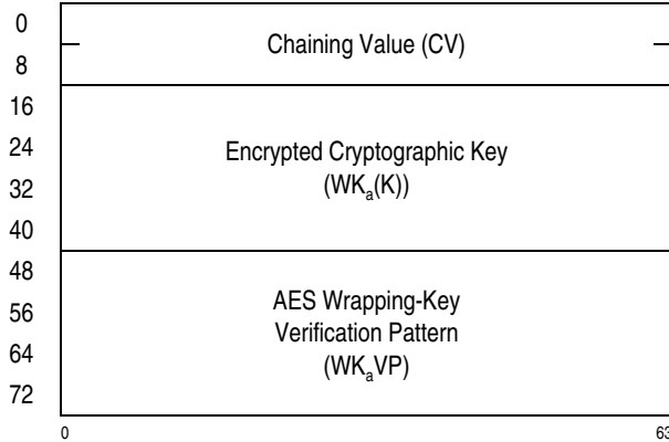
Figure 7-69. Parameter Block for KMC-Encrypted-AES-256
