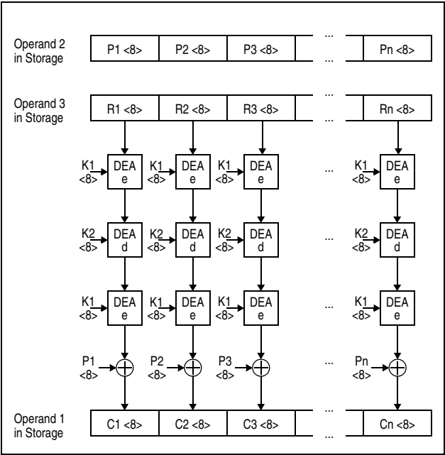
Figure 7-139. KMCTR TDEA Encipher Operation Using 128-Bit Key
