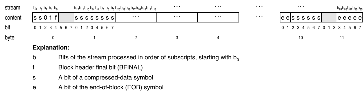
Figure 26-31. Block Type 01 (compressed data using FHT) Example
