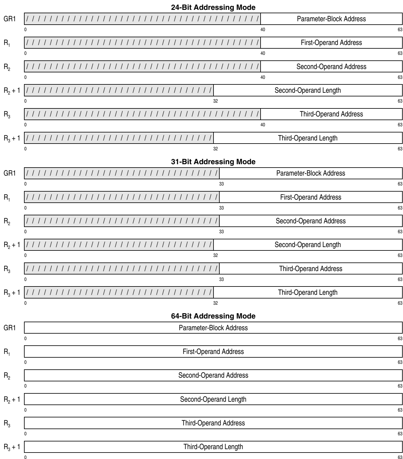
Figure 7-76. General Register Assignment for CIPHER MESSAGE WITH AUTHENTICATION (Part 2 of 2)
