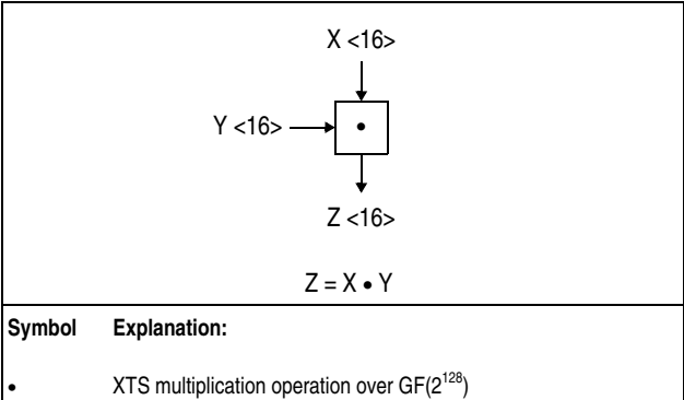
Figure 7-306. Symbol For XTS Multiplication Operation Over GF(2^{128})
