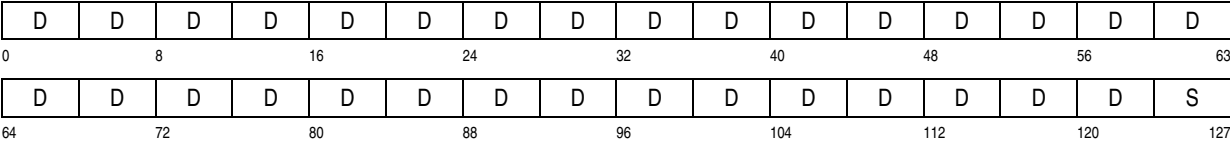
Figure 25-1. Signed-Packed-Decimal Format Number in Vector Registers
