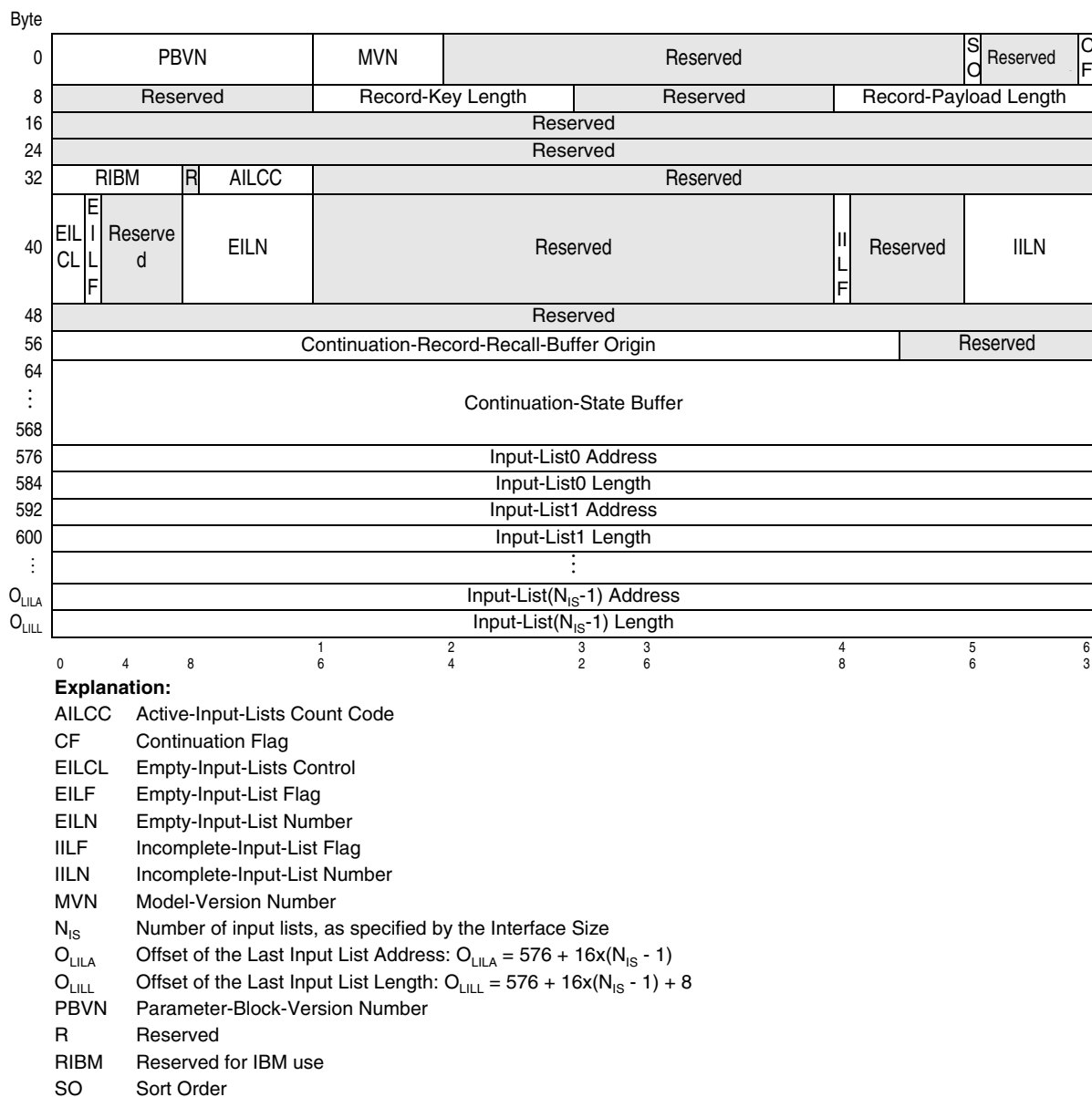
Figure 26-80. Parameter Block (format 0 hex) for SORTL-SFLR and SORTL-SVLR
