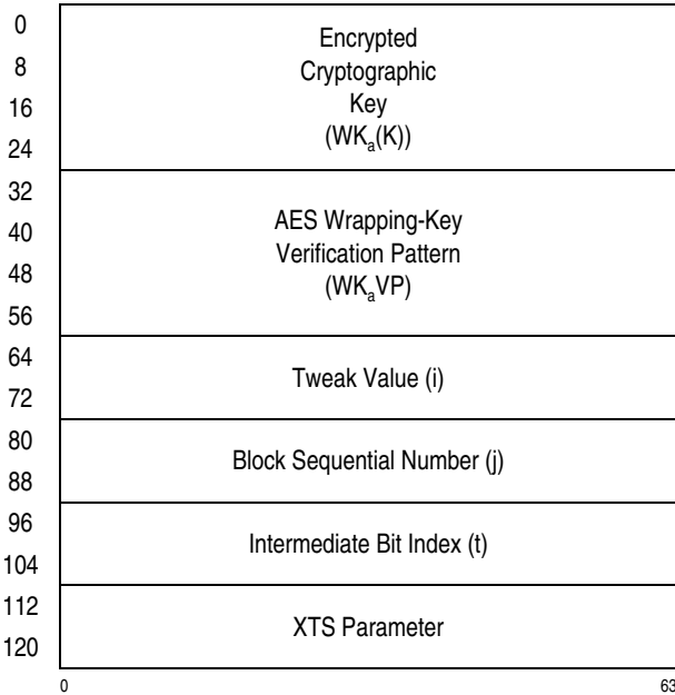
Figure 7-335. Parameter Block for PCC-Compute-XTS-Parameter-Using-Encrypted-AES-256
