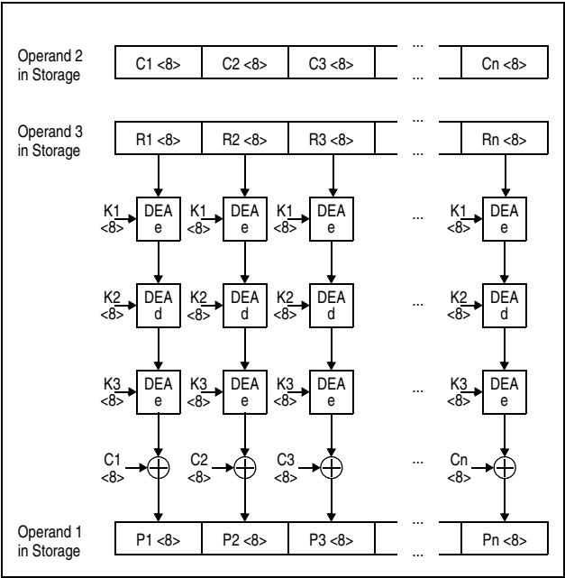
Figure 7-144. KMCTR TDEA Decipher Operation Using 192-Bit Key
