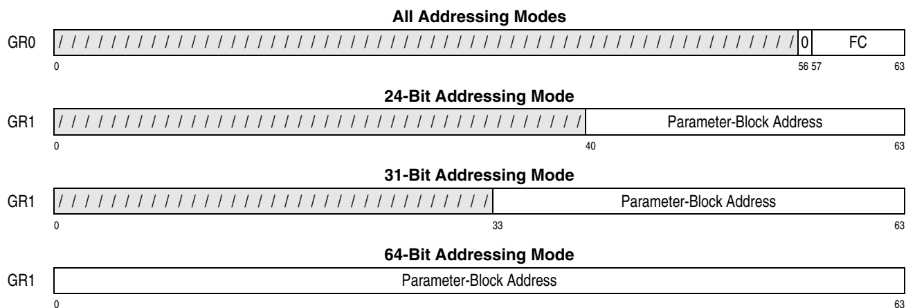
Figure 7-304. General Register Assignment for PCC
