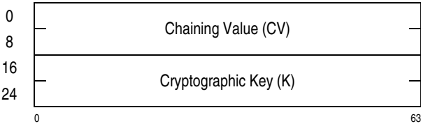
Figure 7-60. Parameter Block for KMC-AES-128
