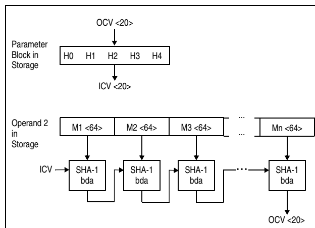
Figure 7-215. KIMD-SHA-1
