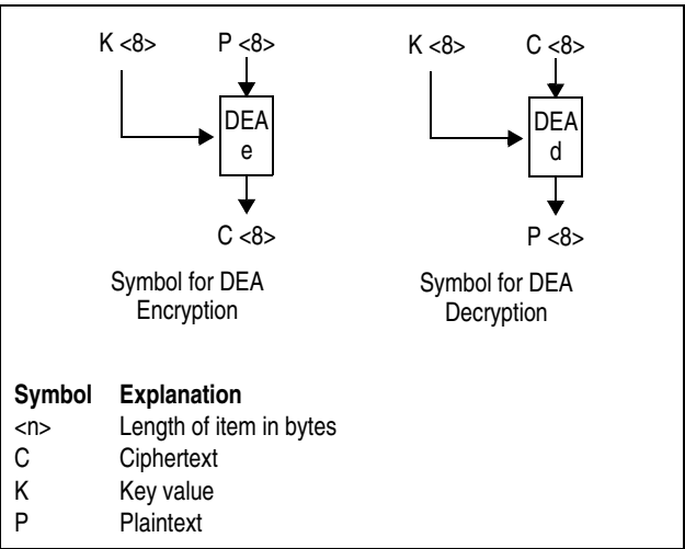
Figure 7-308. Symbols for DEA Encryption and Decryption
