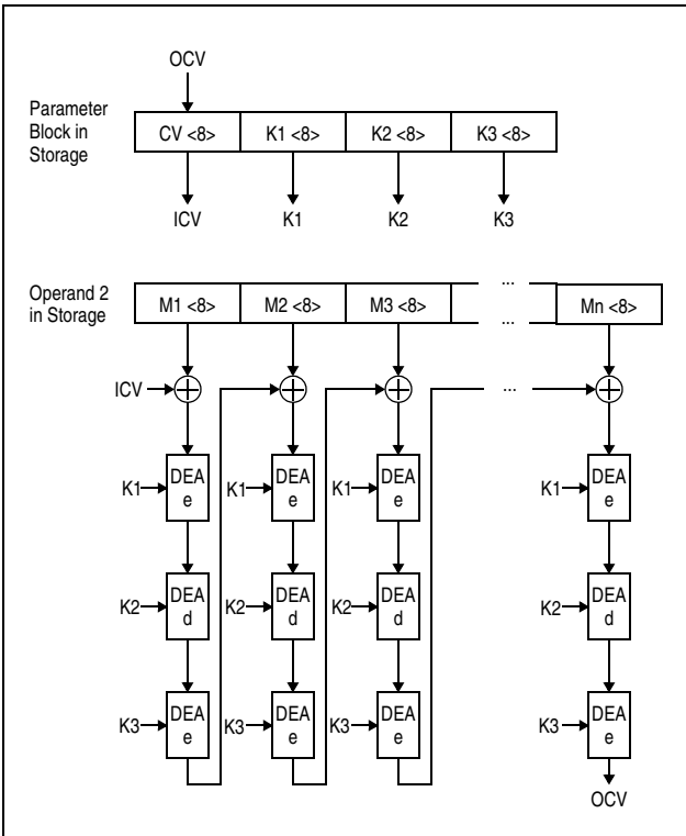
Figure 7-281. MAC Computation Using 192-bit TDEA Key
