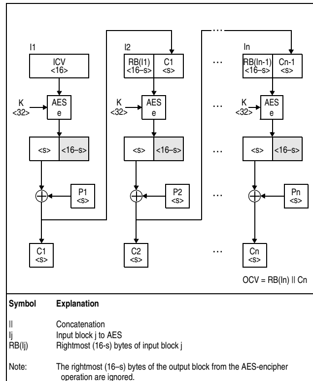
Figure 7-122. KMF-AES-256 Encipher Operation
