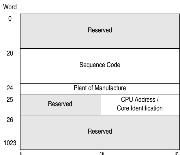
Figure 10-90. Format of the SYSIB 1.2.1
