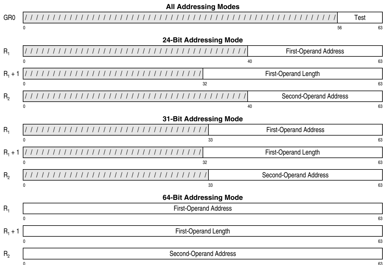
Figure 7-367. Register Contents for TRANSLATE EXTENDED
