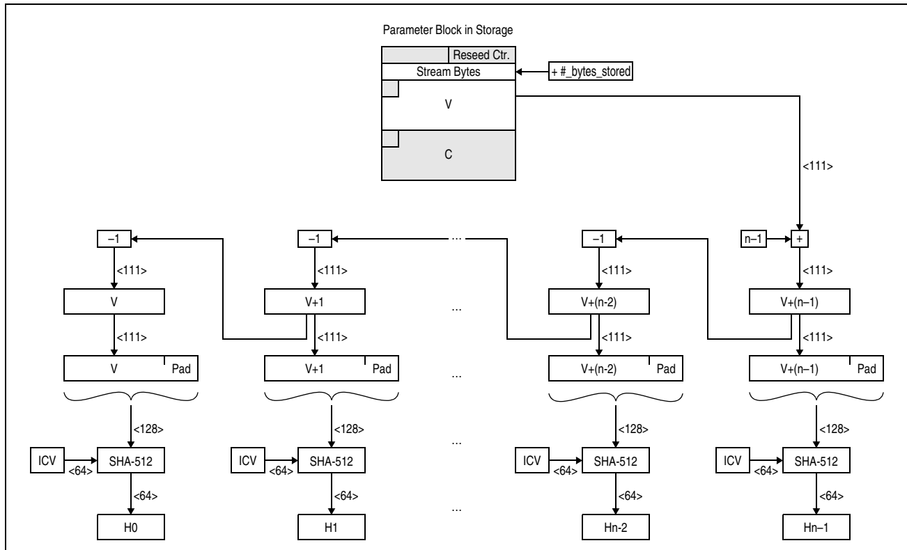
Figure 7-357. PRNO-SHA-512-DRNG Function's Generate Operation Generation of Deterministic Pseudorandom Numbers (Part 1 of 2)
