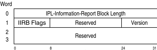
Figure 17-5. IPL-Information-Report BlockHeader
