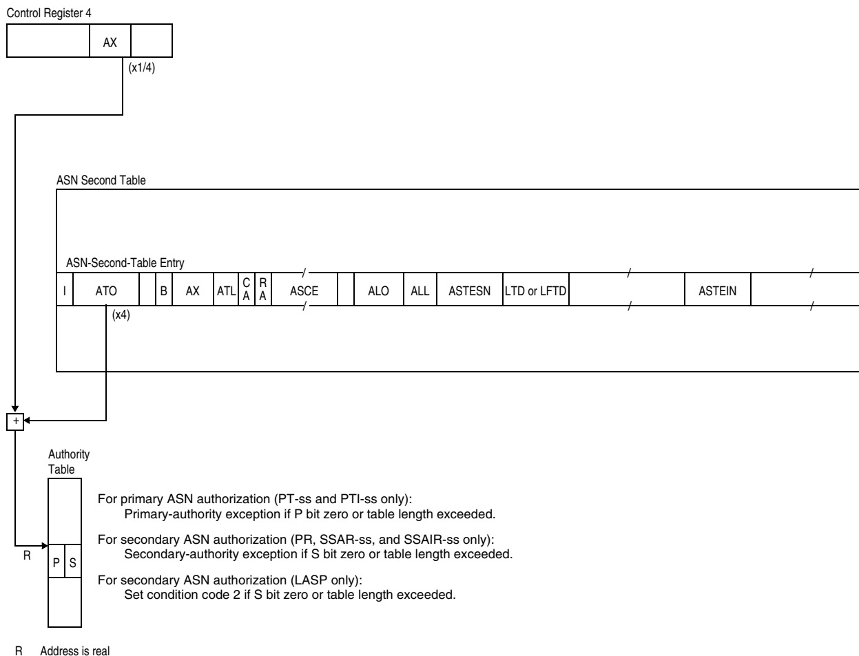
Figure 3-14. ASN Authorization
