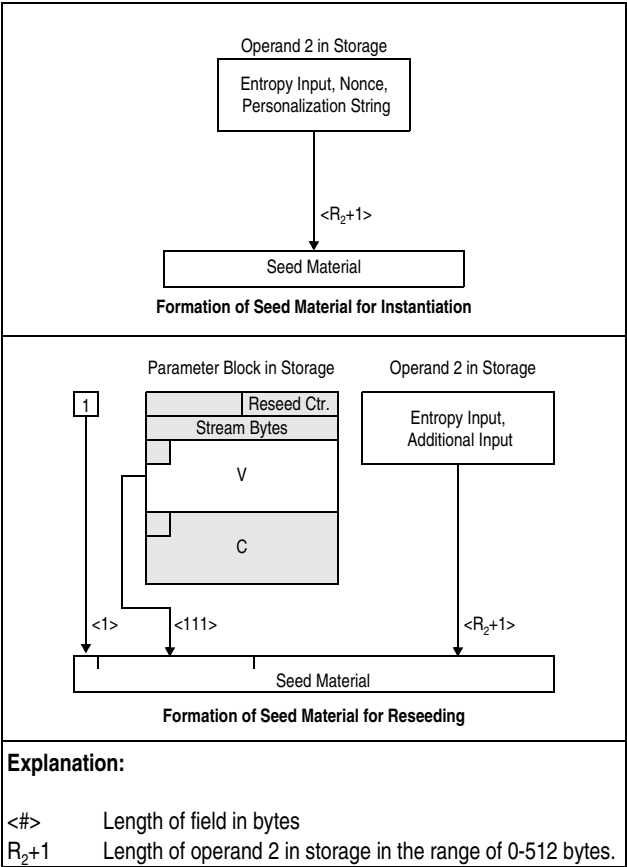
Figure 7-354. PRNO-SHA-512-DRNG Function's Seed Operation Generation of Seed Material
