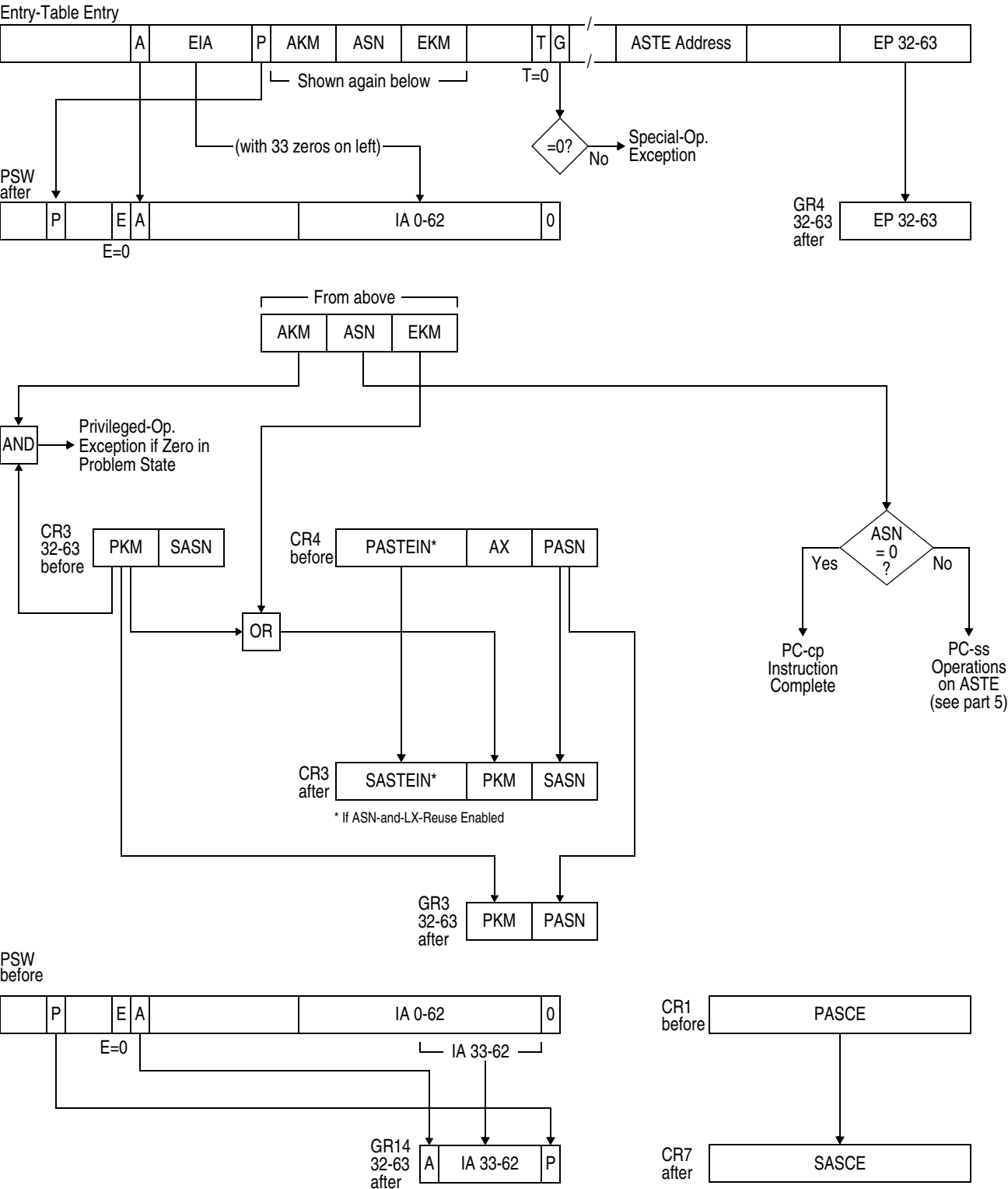
Figure 10-74. Execution of PROGRAM CALL (Part 1 of 5).
