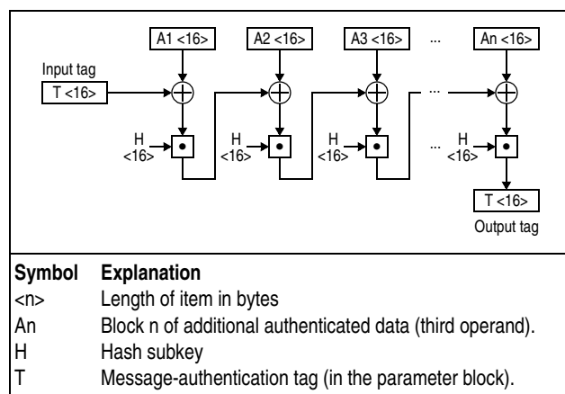
Figure 7-84. GHASH Processing of Full Blocks.
