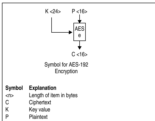
Figure 7-270. Symbols for AES-192 Encryption
