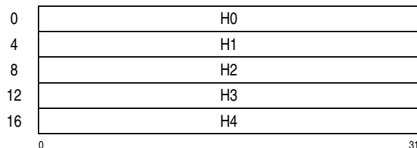
Figure 7-214. Parameter Block for KIMD-SHA-1
