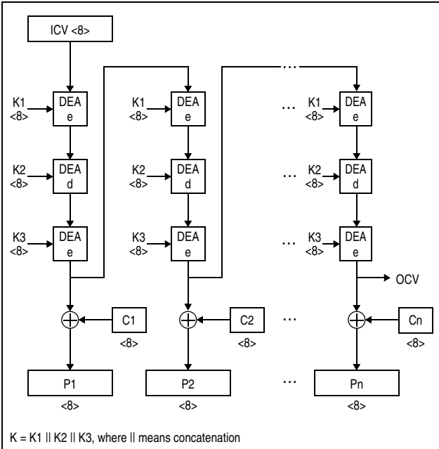
Figure 7-177. KMO-TDEA-192 Decipher Operation
