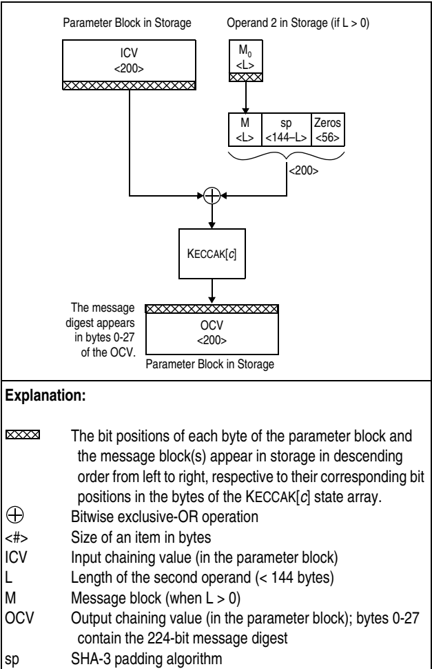
Figure 7-252. KLMD-SHA3-224 Processing (L < 144)
