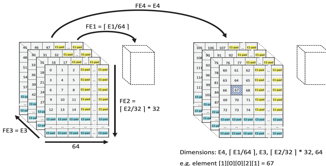
Figure 26-51. Example of a transformed 4D-tensor in data-layout-format 0
