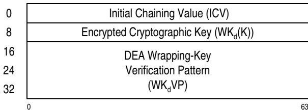
Figure 7-274. Parameter Block for KMAC-Encrypted-DEA
