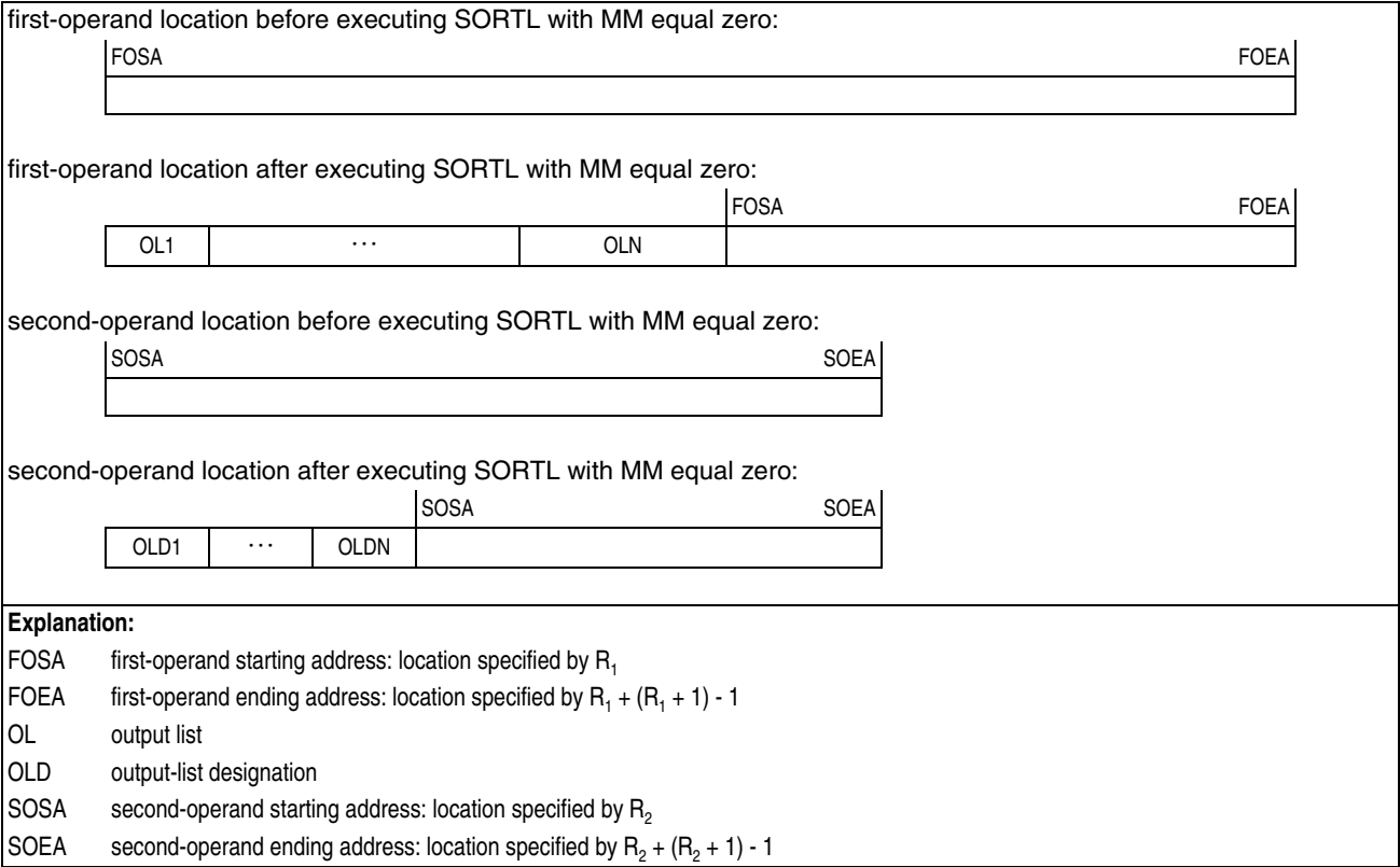
Figure 26-82. First and second operands before and after executing SORTL with MM equal zero
