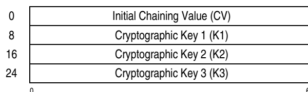
Figure 7-279. Parameter Block for KMAC-TDEA-192
