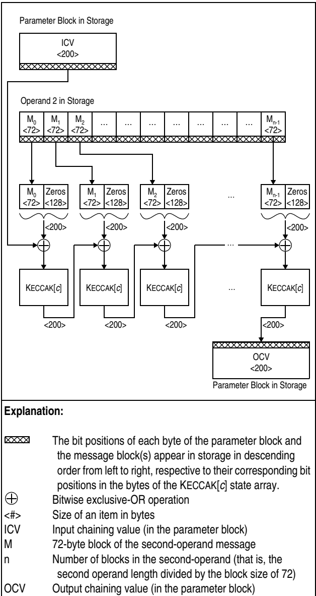
Figure 7-227. KIMD-SHA3-512 Processing
