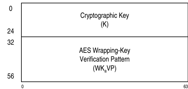
Figure 10-49. Parameter Block for PCKMO-Encrypt-ECC-P256-Key
