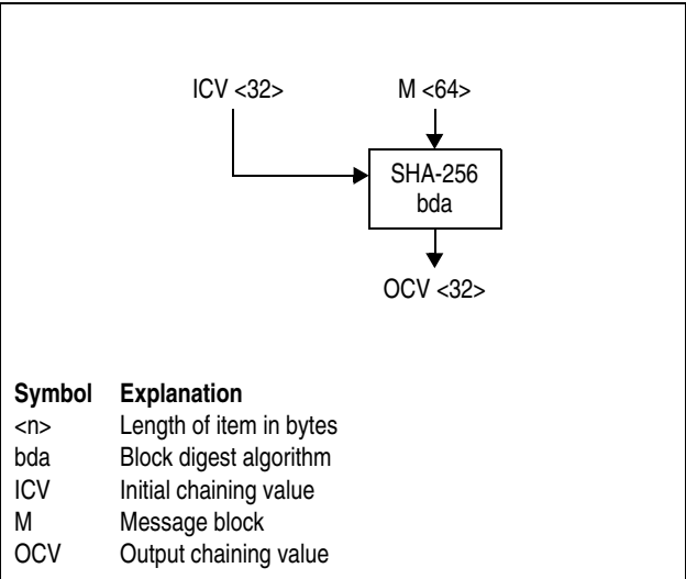
Figure 7-210. Symbol for SHA-256 Block Digest Algorithm
