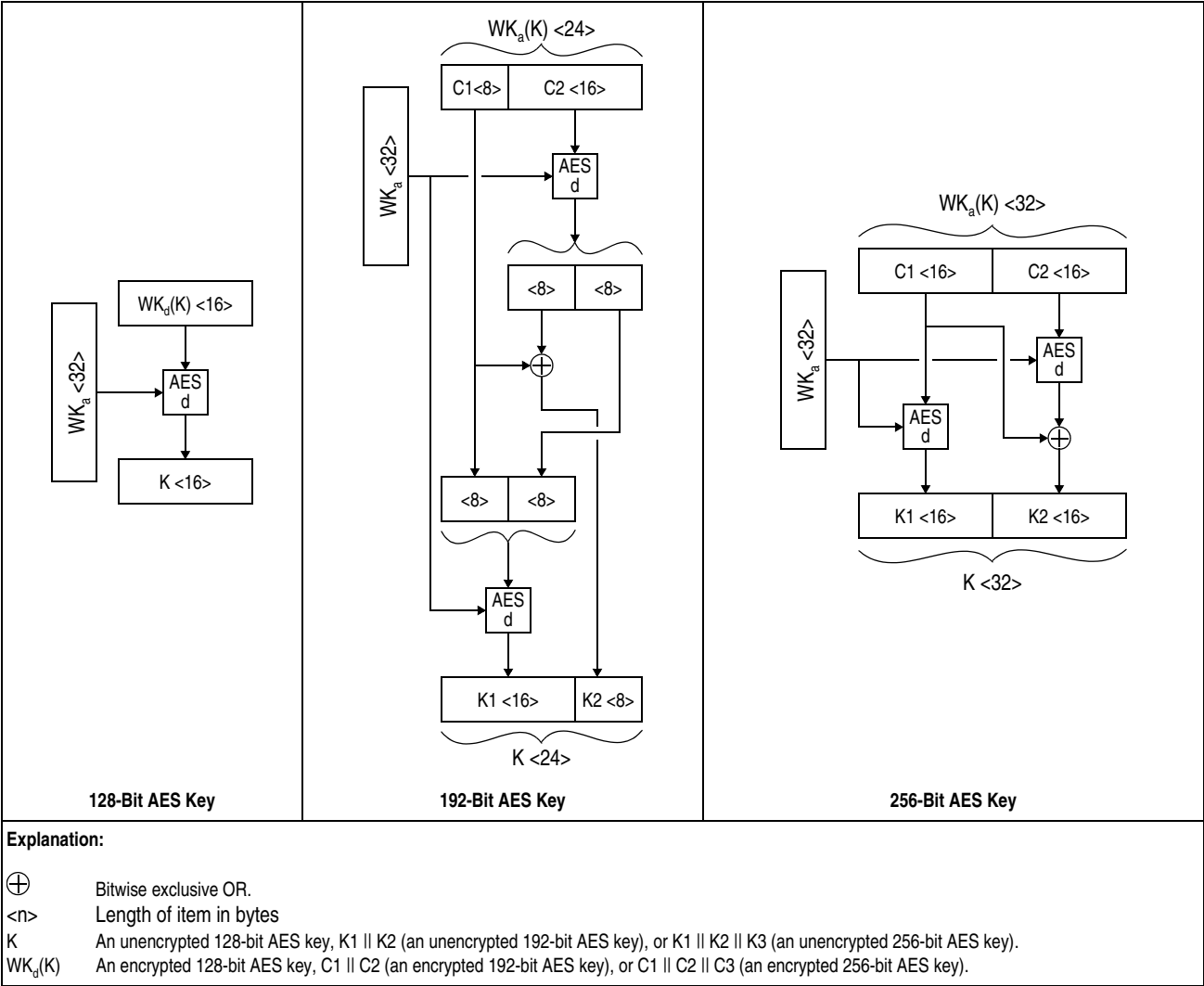
Figure 7-376. Decryption of AES Keys Using WK d
