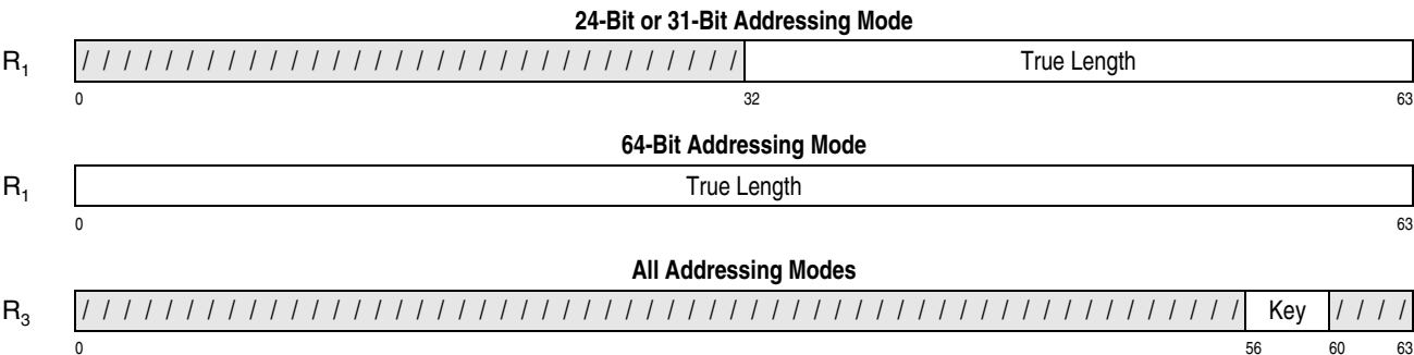
Figure 10-34. Register Contents of MOVE WITH KEY
