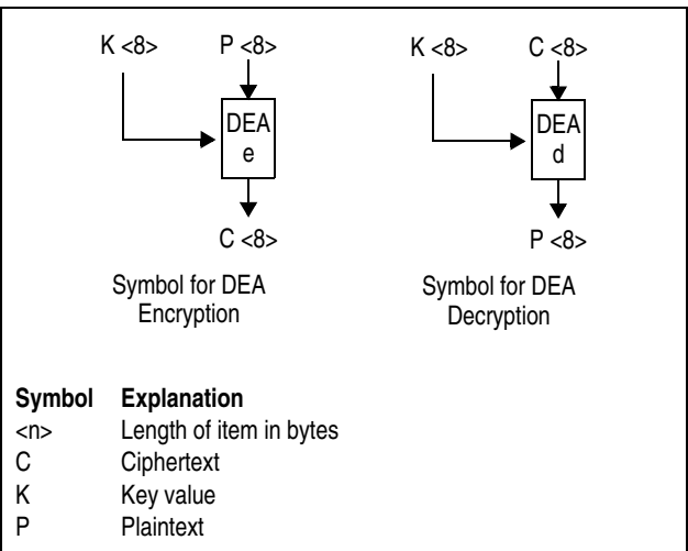
Figure 7-161. Symbols for DEA Encryption and Decryption
