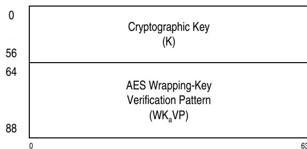
Figure 10-53. Parameter Block for PCKMO-Encrypt-ECC-Ed448-Key
