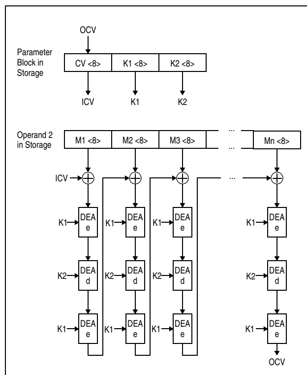
Figure 7-278. MAC Computation Using 128-bit TDEA Key
