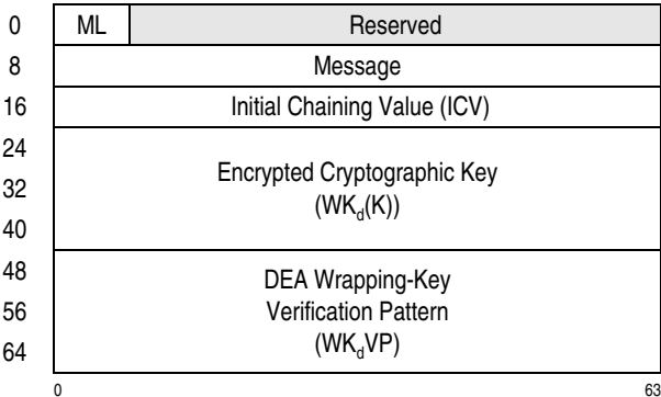
Figure 7-320. Parameter Block for PCC-Compute-Last-Block-CMAC-Using-Encrypted-TDEA-192
