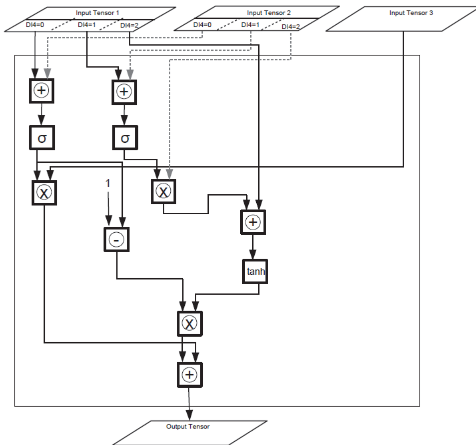
Figure 26-67. NNPA-GRUACT operation
