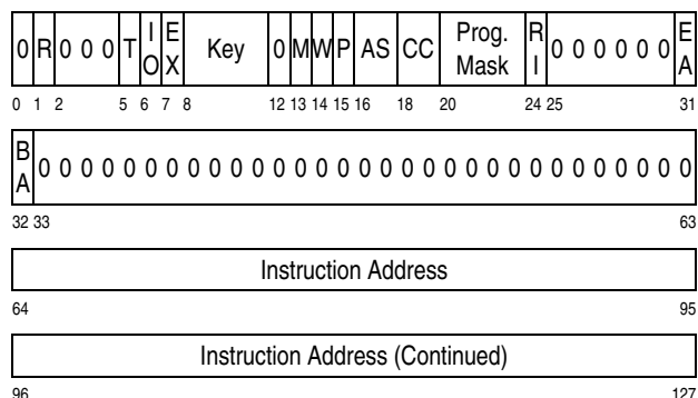
Figure 4-2. PSW Format
