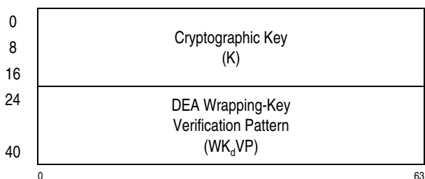
Figure 10-45. Parameter Block for PCKMO-Encrypt-TDEA-192-Key
