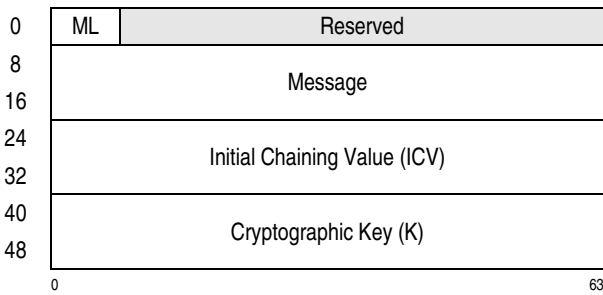
Figure 7-322. Parameter Block for PCC-Compute-Last-Block-CMAC-Using-AES-128
