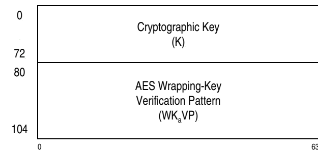
Figure 10-51. Parameter Block for PCKMO-Encrypt-ECC-P521-Key
