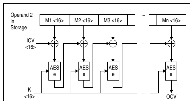
Figure 7-284. KMAC-AES-128
