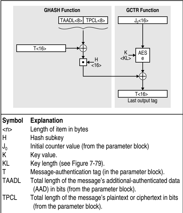
Figure 7-89. Hashing and Encrypting the Last Tag
