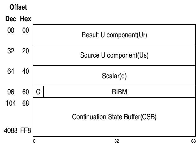
Figure 7-341. Parameter Block for PCC-Scalar-Multiply-X25519 Function
