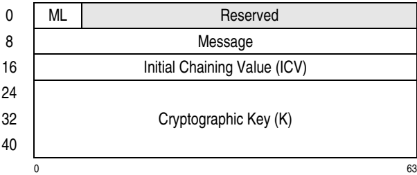
Figure 7-319. Parameter Block for PCC-Compute-Last-Block-CMAC-Using-TDEA-192
