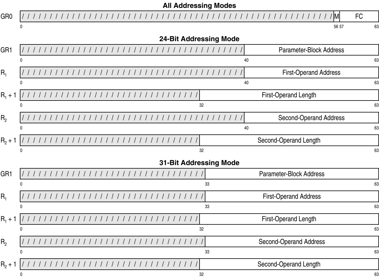
Figure 7-350. General Register Assignment for PERFORM RANDOM NUMBER OPERATION (Part 1 of 2)
