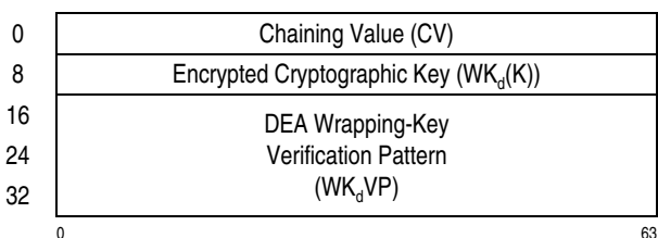
Figure 7-167. Parameter Block for KMO-Encrypted-DEA
