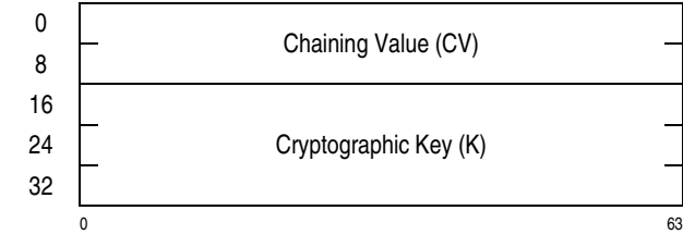
Figure 7-116. Parameter Block for KMF-AES-192
