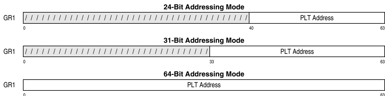
Figure 7-345. General Register Assignment for PLO (Part 2 of 2)
