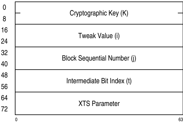
Figure 7-331. Parameter Block for PCC-Compute-XTS-Parameter-Using-AES-128
