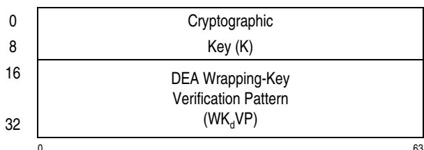
Figure 10-44. Parameter Block for PCKMO-Encrypt-TDEA-128-Key
