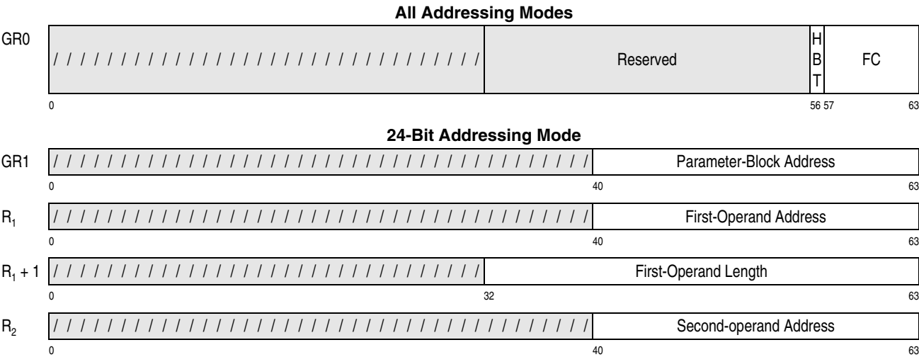
Figure 26-24. General Register Assignment for DFLTCC (Part 1 of 2)
