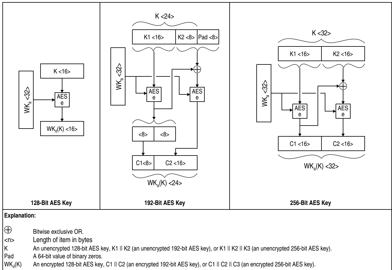
Figure 7-375. Encryption of AES Keys Using WK_d
