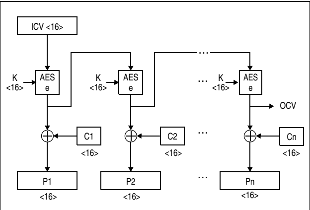
Figure 7-181. KMO-AES-128 Decipher Operation
