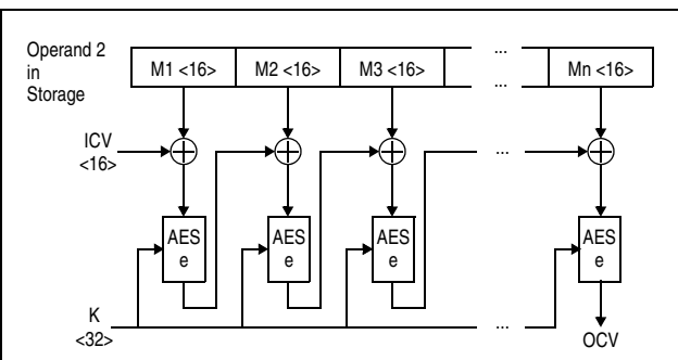
Figure 7-290. KMAC-AES-256
