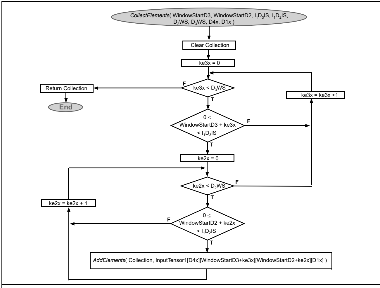
Figure 26-65. NNPA-MAXPOOL2D/AVGPOOL2D (Part 2 of 2)
