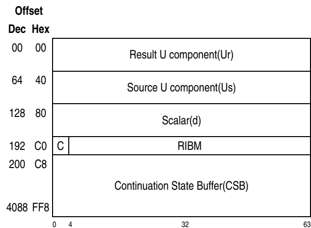
Figure 7-342. Parameter Block for PCC-Scalar-Multiply-X448 Function
