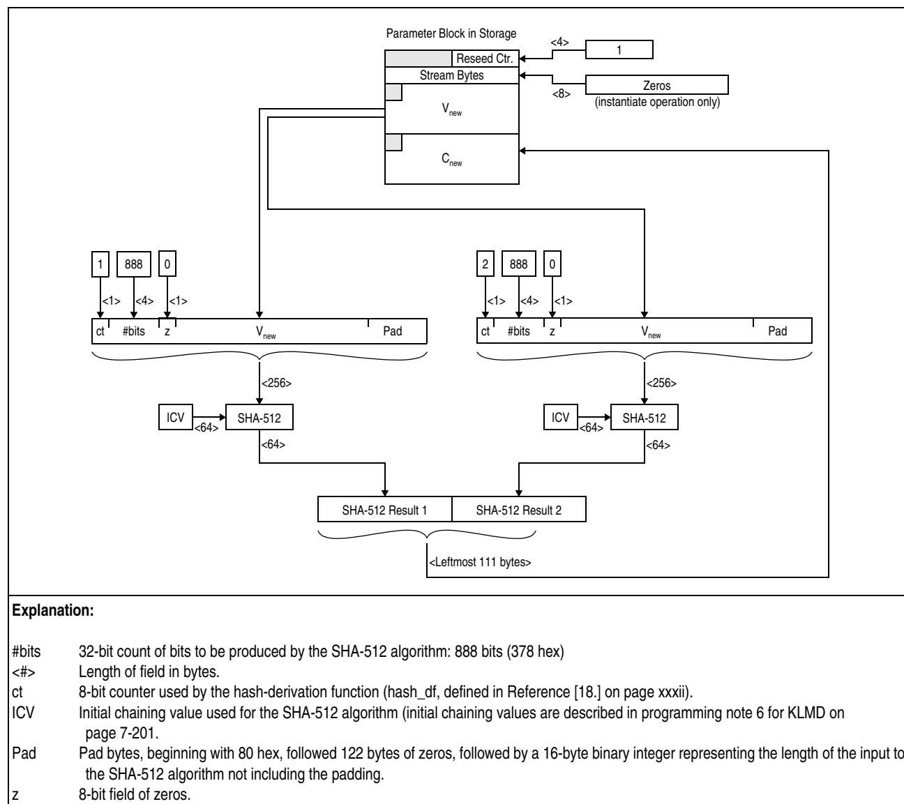
Figure 7-356. PRNO-SHA-512-DRNG Function's Seed Operation Formation of New Constant ( C_{new} ) and Initialization of the Reseed-Counter and Stream-Bytes Fields
