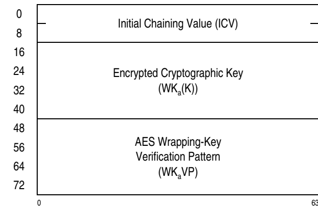
Figure 7-289. Parameter Block for KMAC-Encrypted-AES-256
