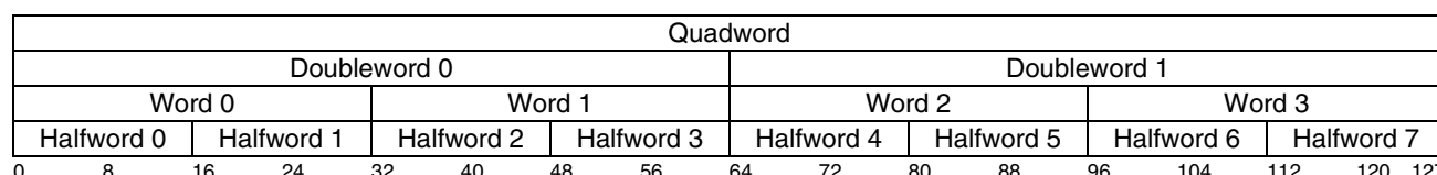
Figure 21-1. Vector Register Element Representations
