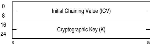
Figure 7-282. Parameter Block for KMAC-AES-128
