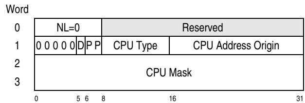
Figure 10-99. CPU-Type Topology-List Entry
