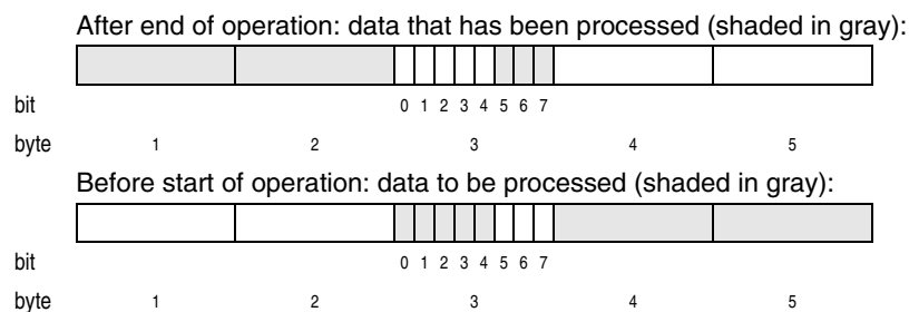
Figure 26-28. Sub-byte Boundary (SBB) Example
