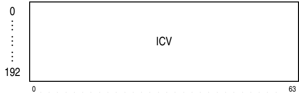
Figure 7-261. Parameter Block for KLMD-SHAKE-256
