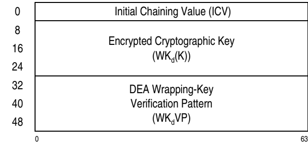
Figure 7-280. Parameter Block for KMAC-Encrypted-TDEA-192
