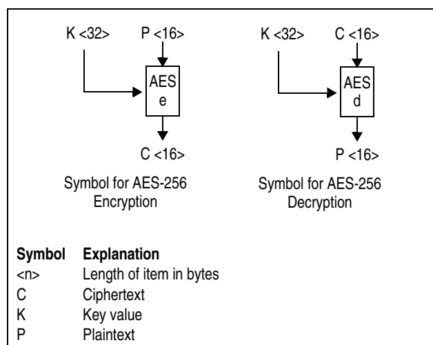
Figure 7-311. Symbols for AES-256 Encryption and Decryption
