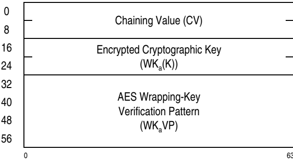
Figure 7-113. Parameter Block for KMF-Encrypted-AES-128
