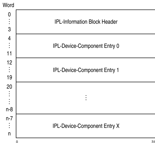
Figure 17-9. IPL-Information Block for IPL-Device-Component List
