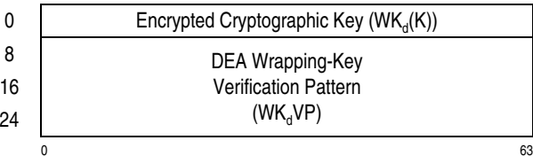
Figure 7-16. Parameter Block for KM-Encrypted-DEA
