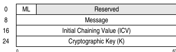
Figure 7-313. Parameter Block for PCC-Compute-Last-Block-CMAC-Using-DEA
