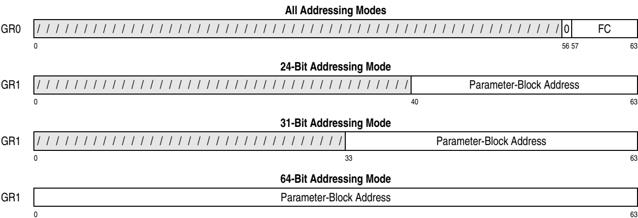
Figure 10-41. General Register Assignment for PCKMO
