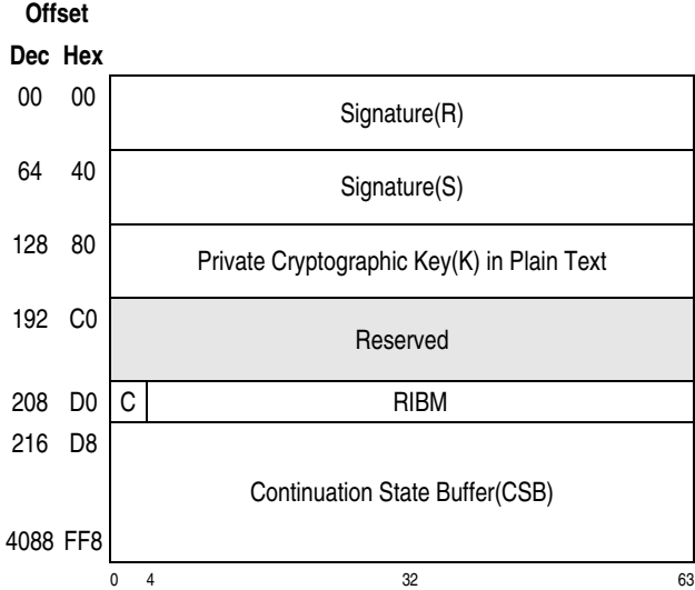
Figure 26-17. Parameter Block for KDSA-EdDSA-Sign-Ed448 Function
