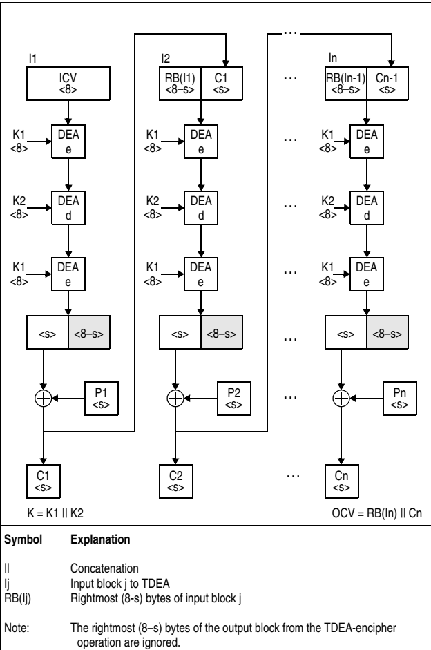
Figure 7-106. KMF-TDEA-128 Encipher Operation
