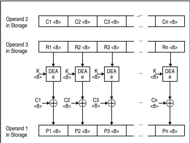
Figure 7-136. KMCTR DEA Decipher Operation Using 64-Bit Key
