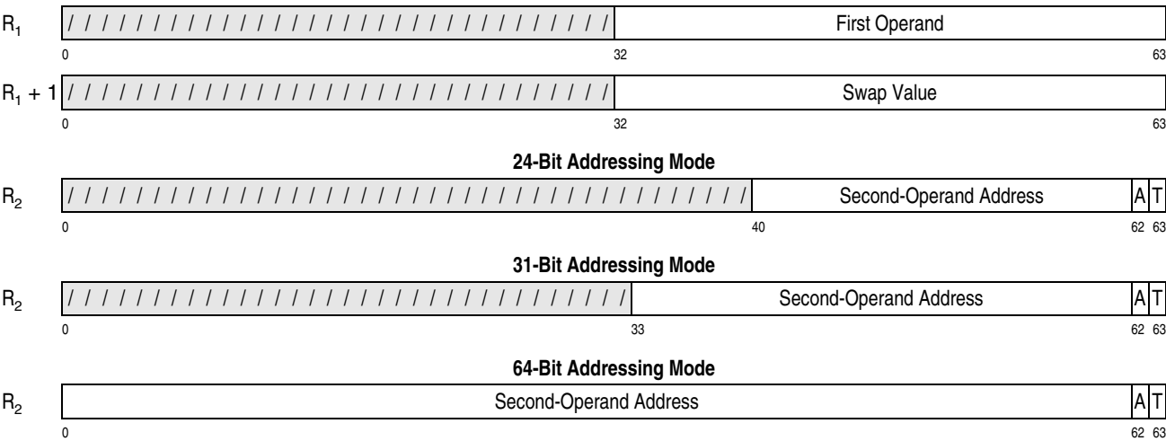
Figure 10-6. Register Contents for COMPARE AND SWAP AND PURGE (CSP)
