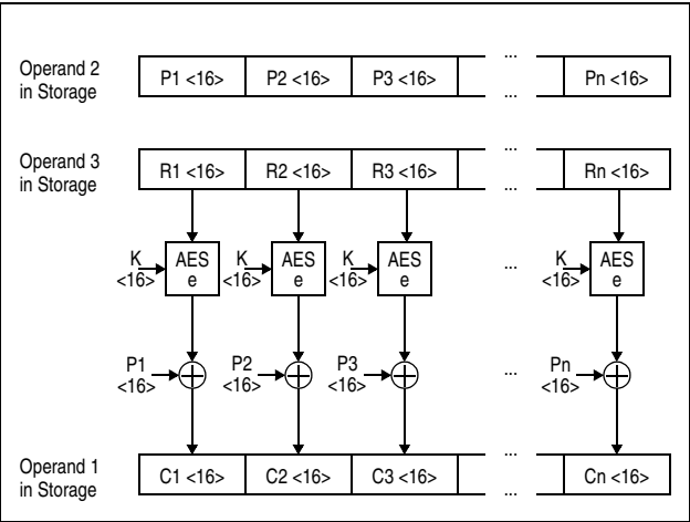
Figure 7-147. KMCTR AES Encipher Operation Using 128-Bit Key
