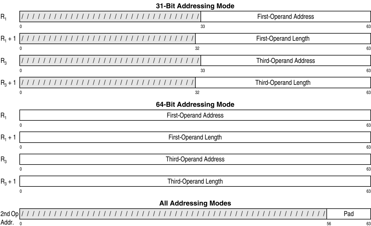
Figure 7-301. Register Contents and Second-Operand Address for MOVE LONG EXTENDED (Part 2 of 2)
