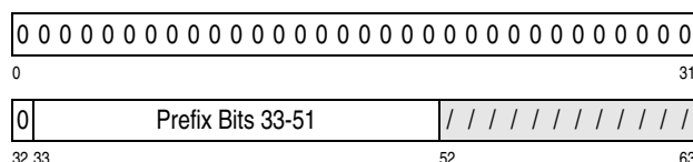
Figure 3-11. ESA/390-Compatibility Mode Prefix Register
