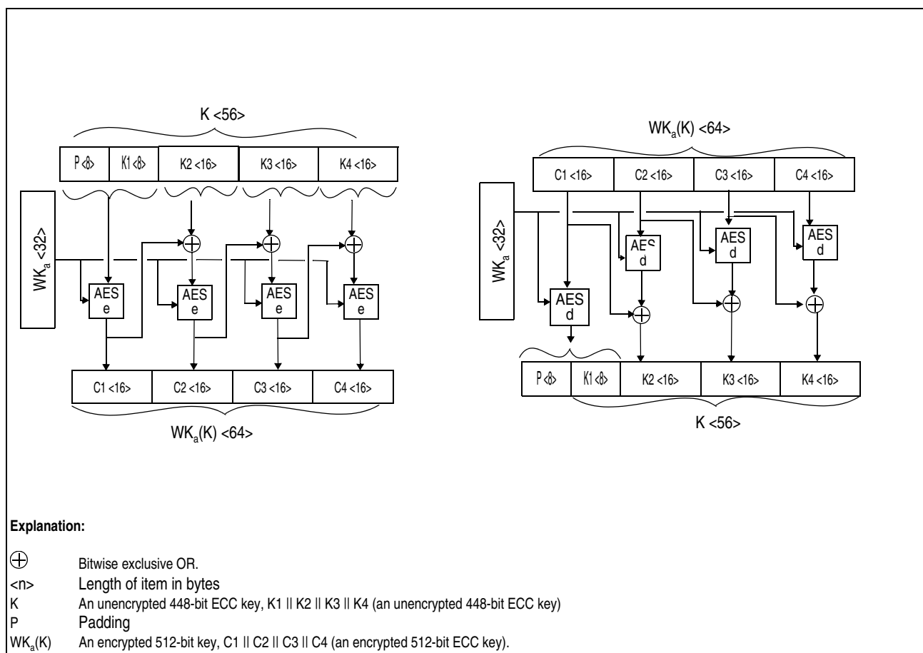
Figure 7-379. Encryption and Decryption of ECC Keys for Ed448 Using WK_a
