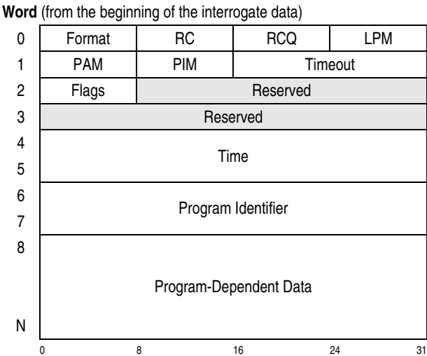
Figure 15-19. Interrogate Data
