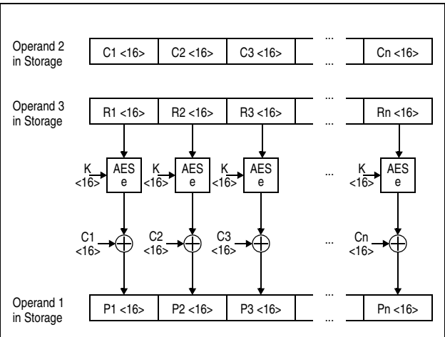
Figure 7-148. KMCTR AES Decipher Operation Using 128-Bit Key
