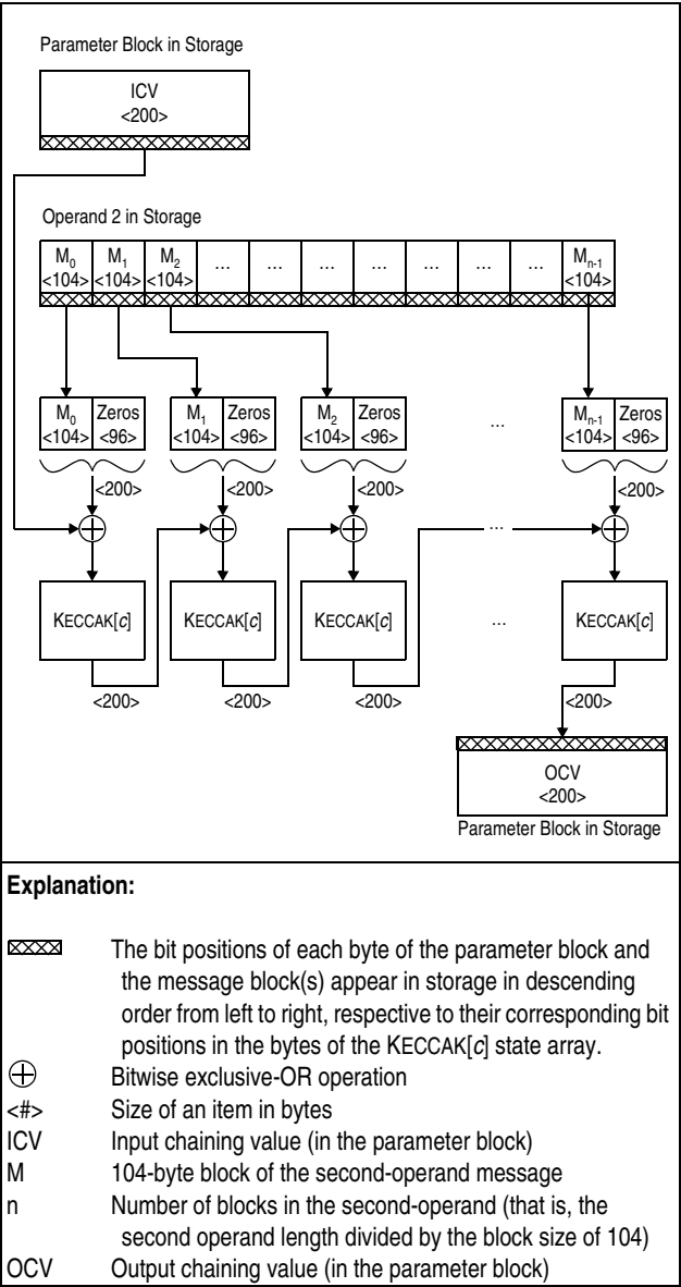
Figure 7-225. KIMD-SHA3-384 Processing
