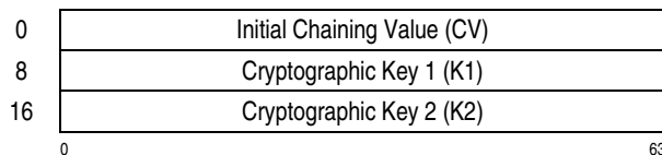
Figure 7-276. Parameter Block for KMAC-TDEA-128
