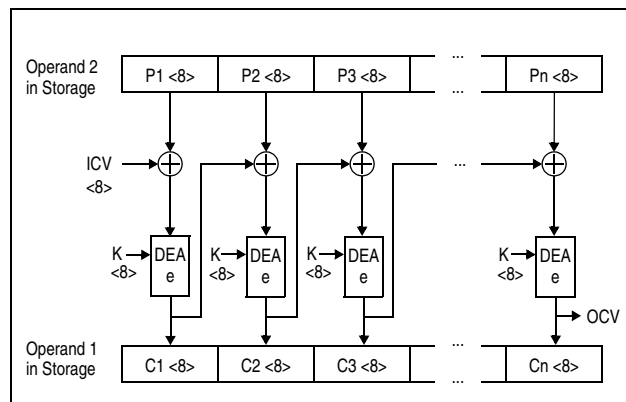
Figure 7-50. KMC DEA Encipher Operation Using 64-Bit Key
