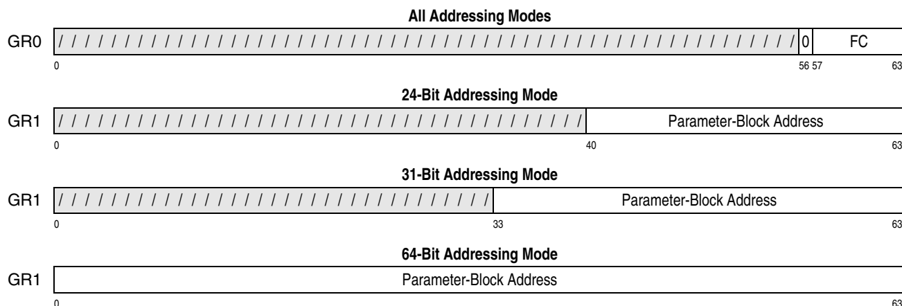
Figure 10-55. General Register Assignment for PERFORM TIMING FACILITY FUNCTION
