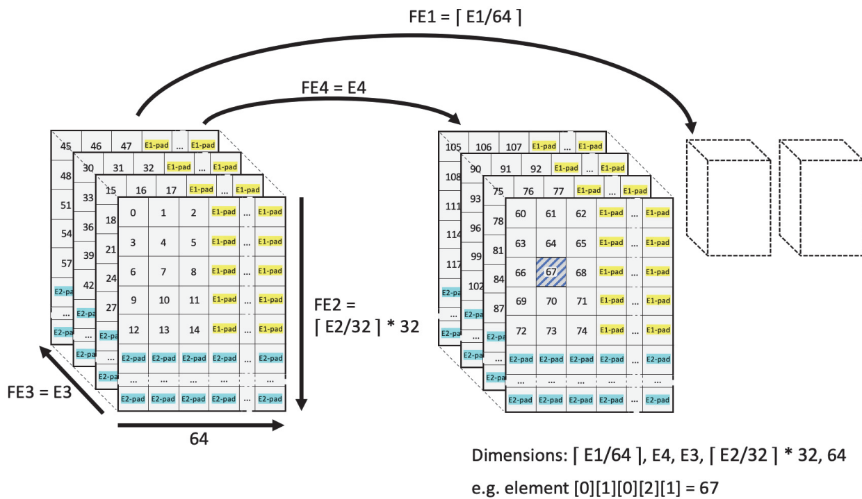
Figure 26-52. Example of a transformed 4D-tensor in data-layout-format 1
