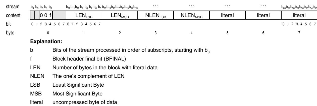
Figure 26-30. Block Type 00 (no compression) Example
