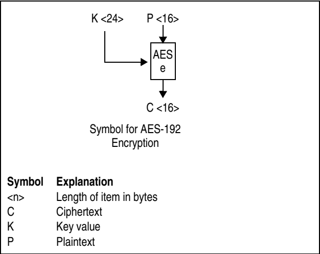
Figure 7-163. Symbols for AES-192 Encryption
