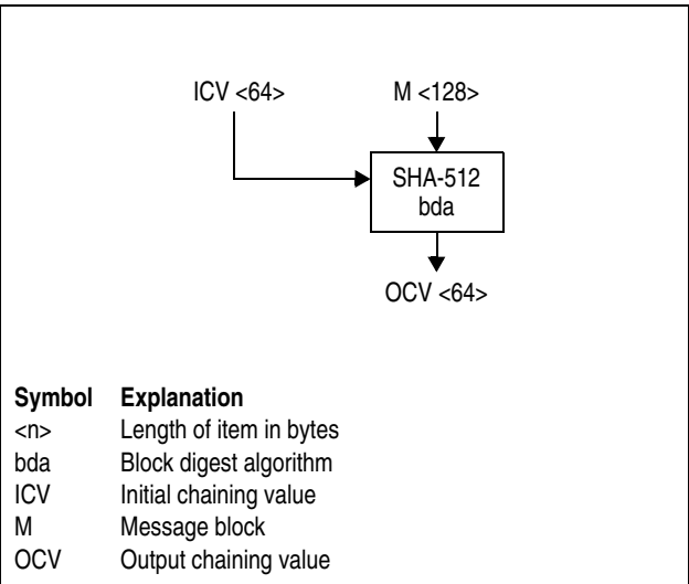
Figure 7-211. Symbol for SHA-512 Block Digest Algorithm
