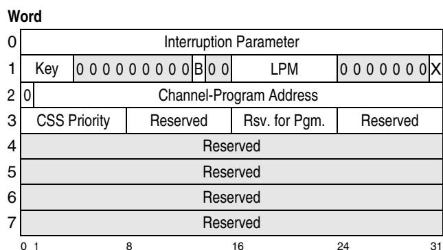
Figure 15-6. Transport-Mode Operation-Request Block
