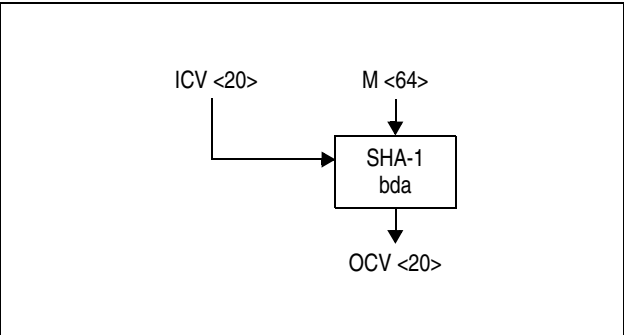
Figure 7-209. Symbol for SHA-1 Block Digest Algorithm
