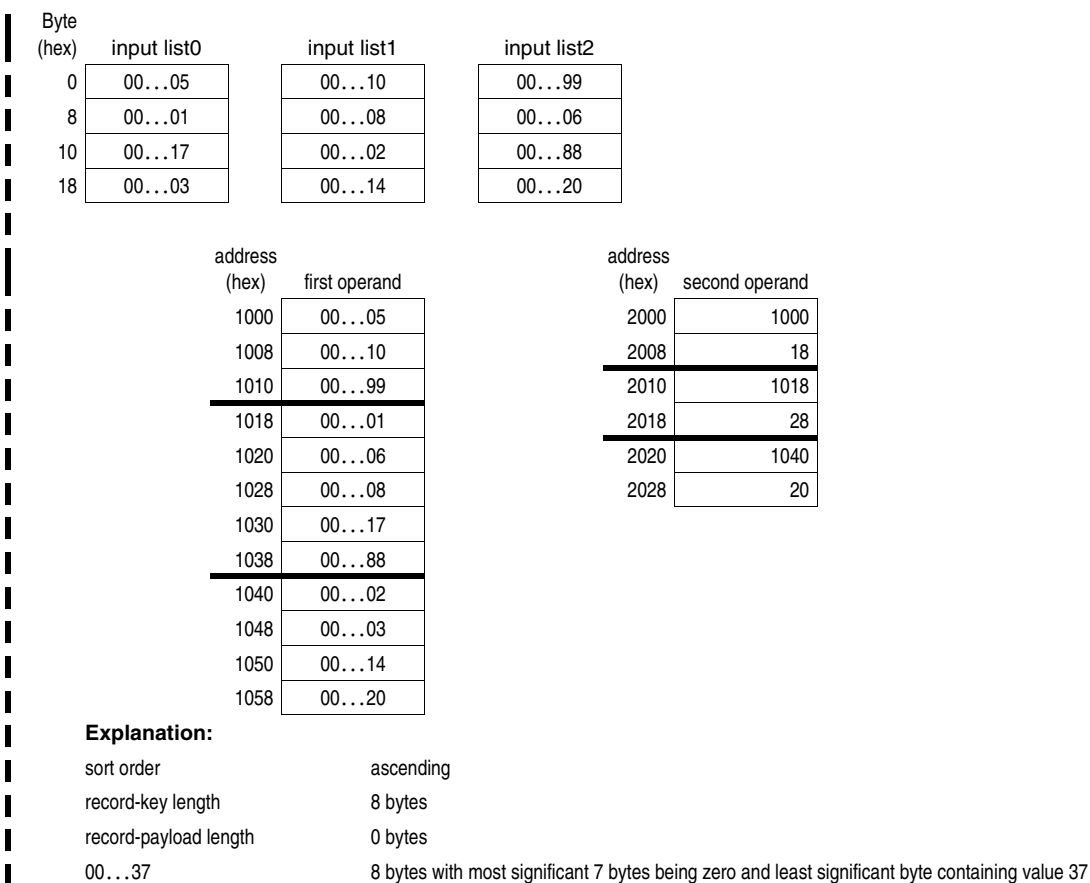
Figure 26-86. SORTL-SFLR Example with 3 input lists
