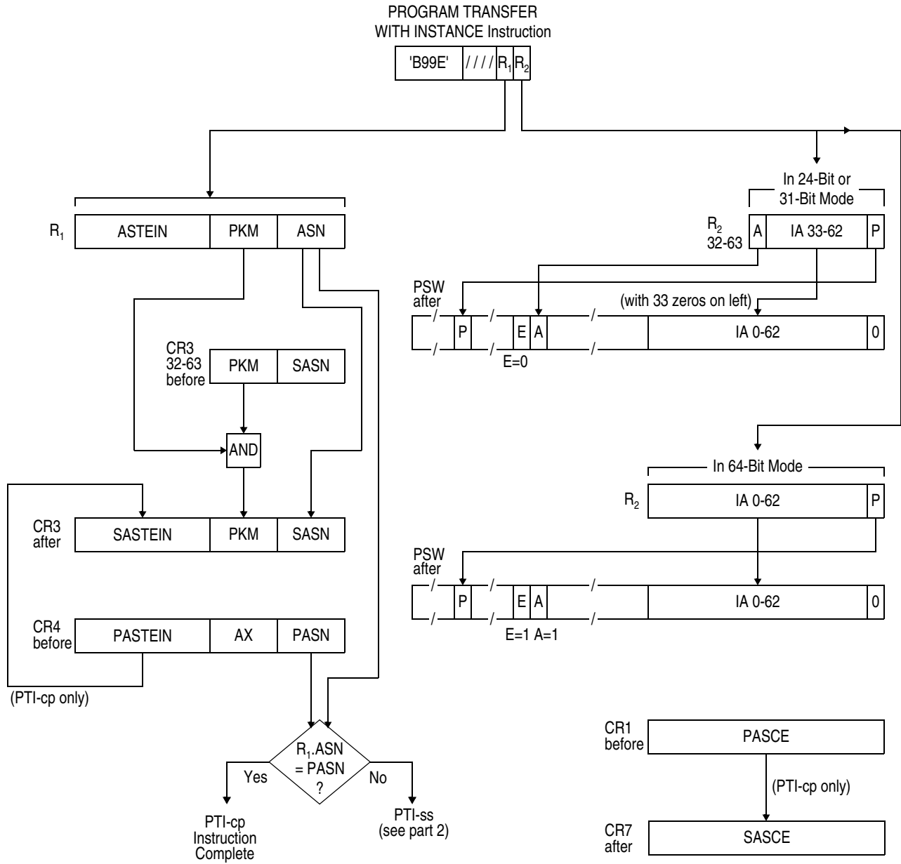
Figure 10-79. Execution of PROGRAM TRANSFER WITH INSTANCE (Part 1 of 2).
