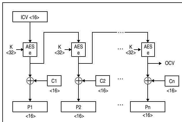
Figure 7-189. KMO-AES-256 Decipher Operation
