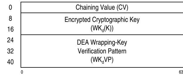
Figure 7-171. Parameter Block for KMO-Encrypted-TDEA-128
