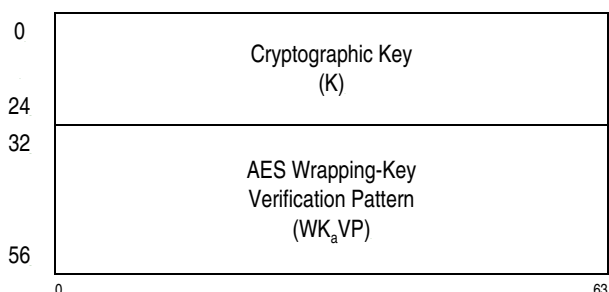
Figure 10-52. Parameter Block for PCKMO-Encrypt-ECC-Ed25519-Key
