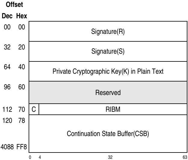
Figure 26-16. Parameter Block for KDSA-EdDSA-Sign-Ed25519 Functions
