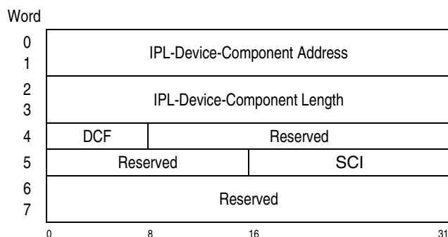
Figure 17-10. IPL-Device-Component Entry
