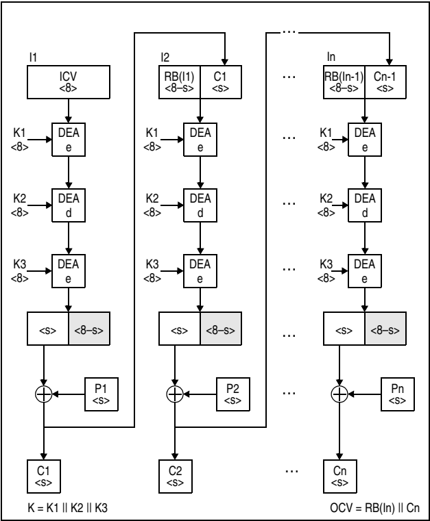
Figure 7-110. KMF-TDEA-192 Encipher Operation
