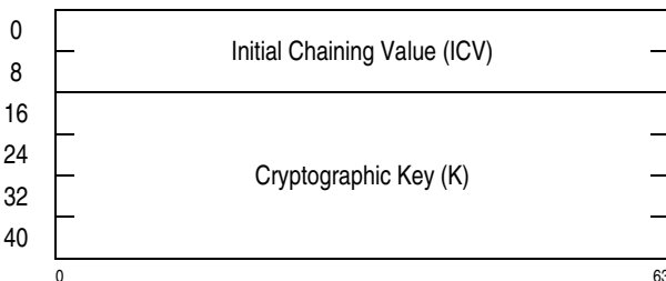
Figure 7-288. Parameter Block for KMAC-AES-256
