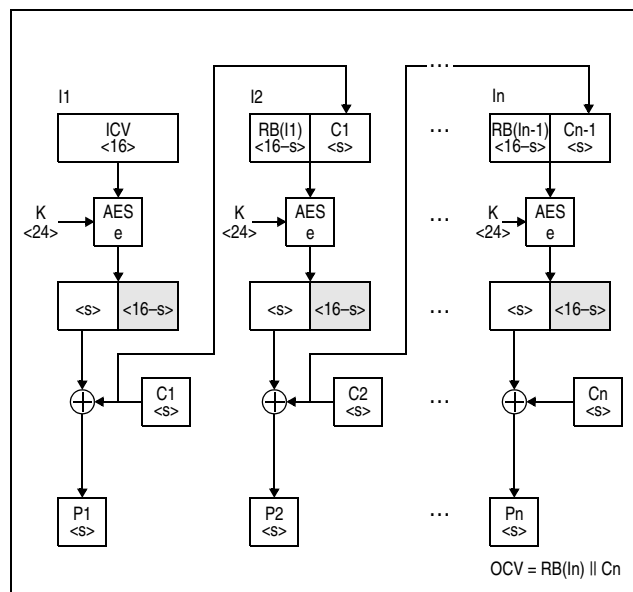
Figure 7-119. KMF-AES-192 Decipher Operation
