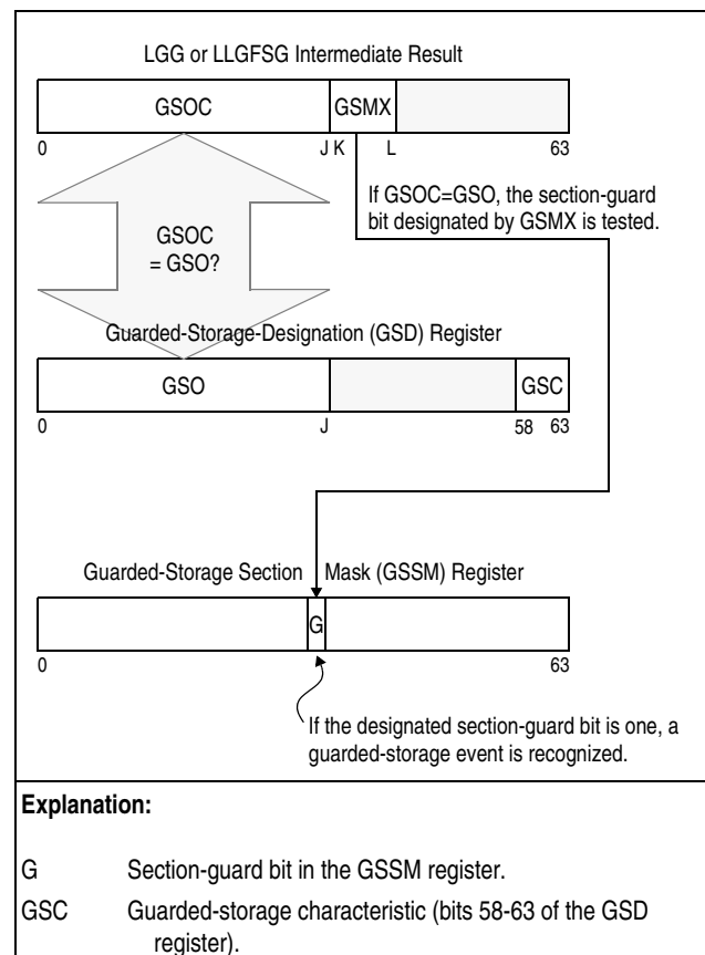
Figure 4-21. Guarded-Storage-Event Detection
