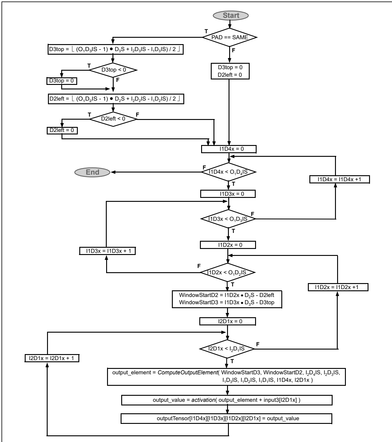
Figure 26-73. NNPA-CONVOLUTION (Part 1 of 2)
