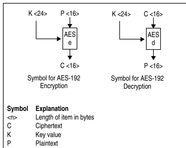
Figure 7-310. Symbols for AES-192 Encryption and Decryption
