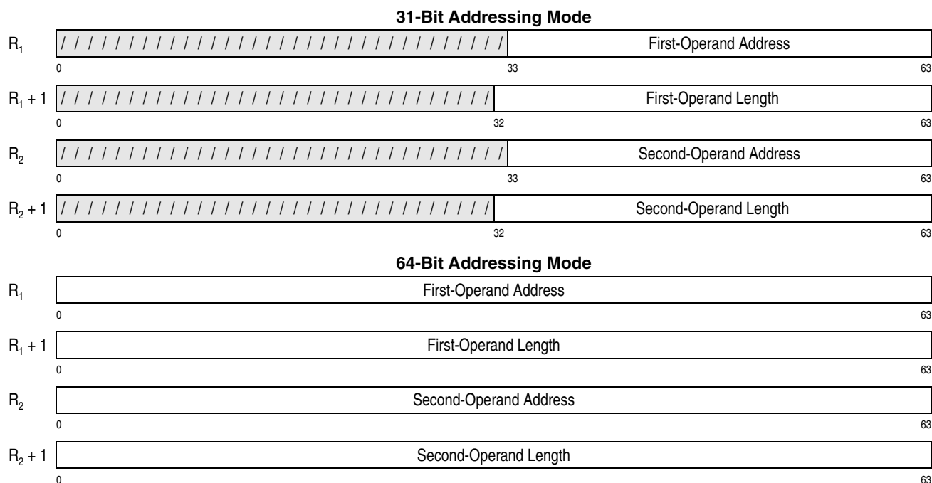
Figure 7-292. Register Contents for CONVERT UTF-16 TO UTF-32 (Part 2 of 2)
