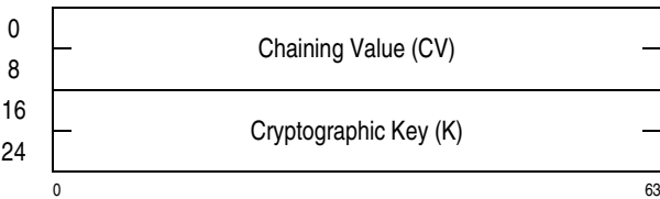
Figure 7-112. Parameter Block for KMF-AES-128
