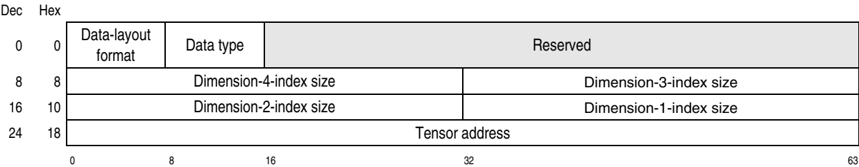
Figure 26-55. Tensor Descriptor for Format 0 Parameter Block
