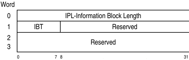
Figure 17-6. IPL-Information Block Header
