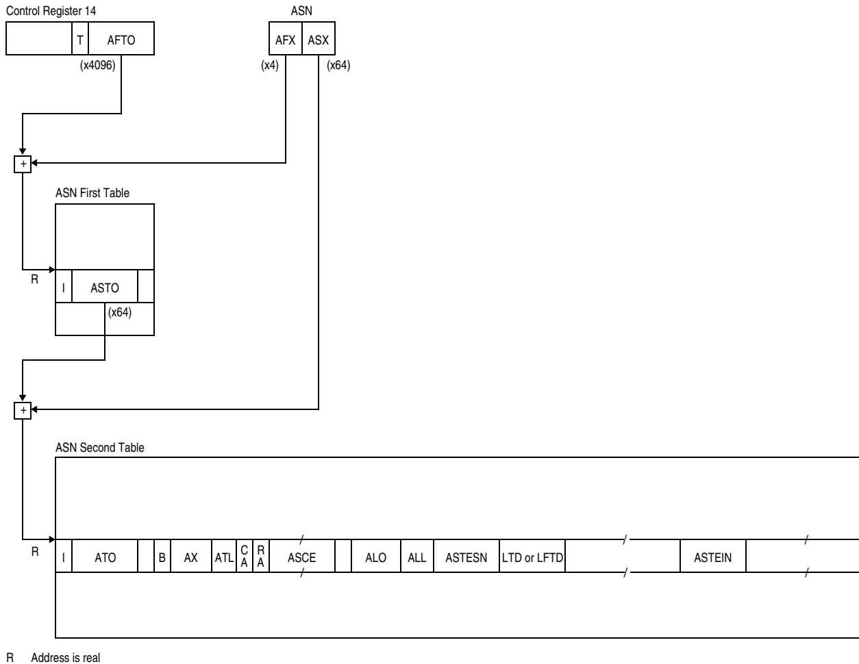
Figure 3-13. ASN Translation
