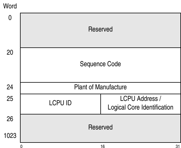
Figure 10-92. Format of the SYSIB 2.2.1
