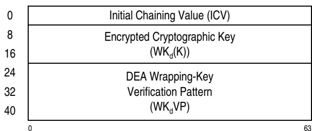
Figure 7-277. Parameter Block for KMAC-Encrypted-TDEA-128
