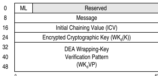
Figure 7-314. Parameter Block for PCC-Compute-Last-Block-CMAC-Using-Encrypted-DEA
