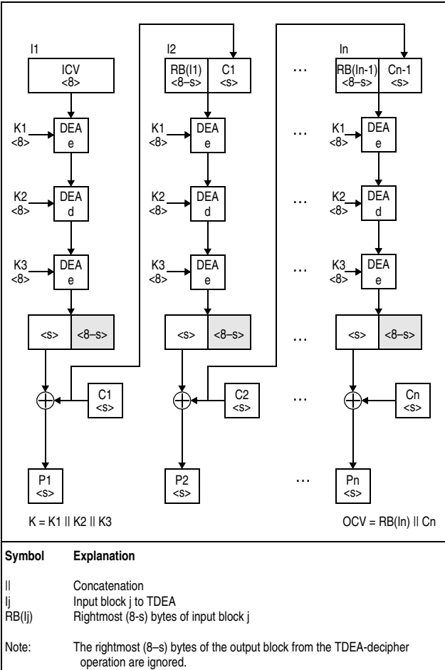
Figure 7-111. KMF-TDEA-192 Decipher Operation
