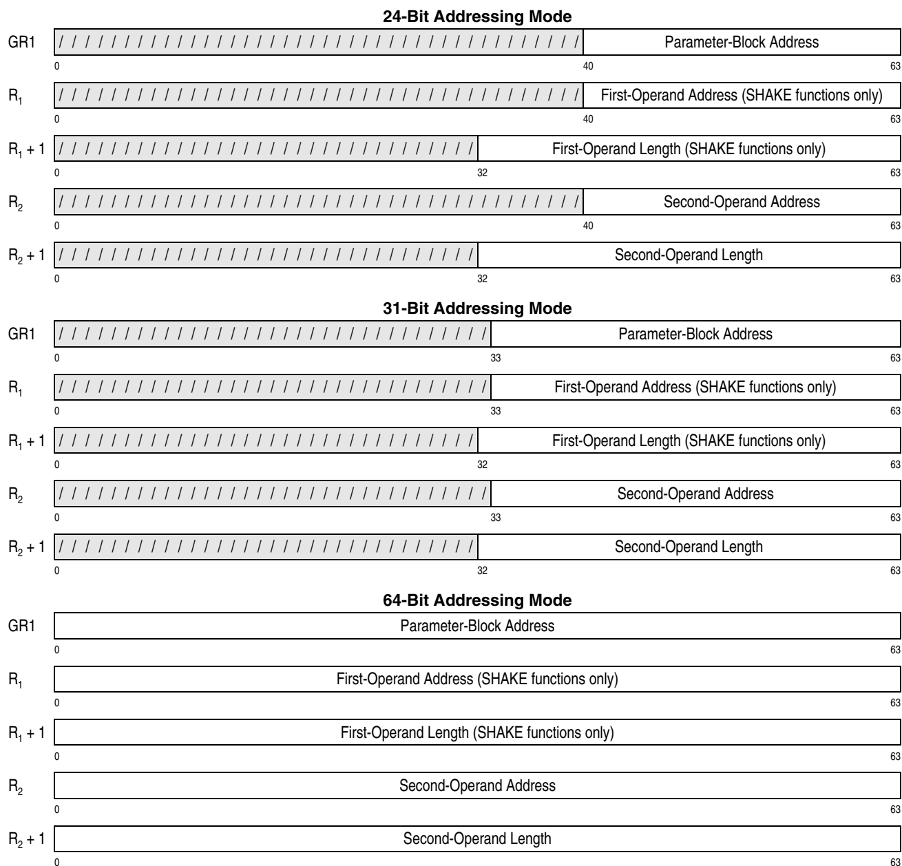
Figure 7-234. General Register Assignment for KLMD (Part 2 of 2)
