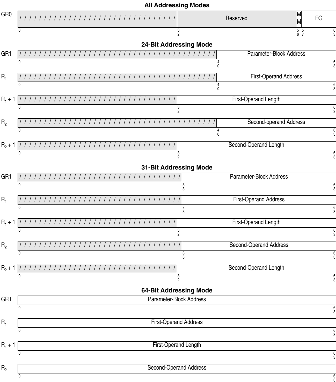
Figure 26-77. General Register Assignments for SORTL (Part 1 of 2)
