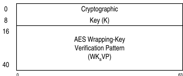
Figure 10-46. Parameter Block for PCKMO-Encrypt-AES-128-Key
