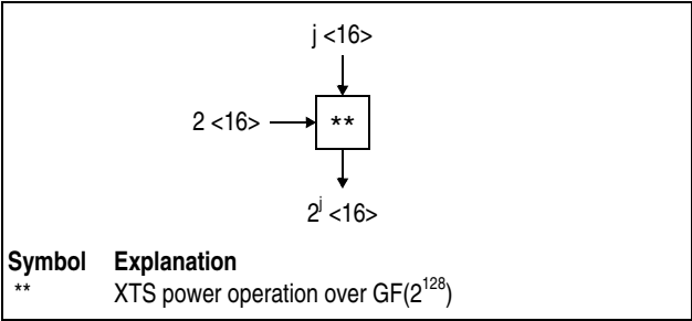
Figure 7-307. Symbol For XTS Power Operation Over GF(2^{128})
