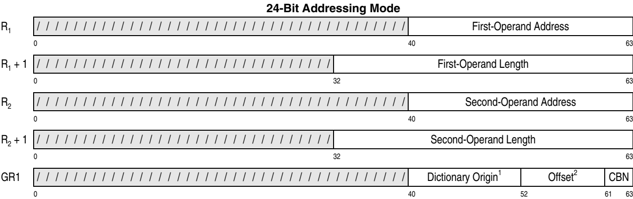
Figure 7-200. Register Contents for COMPRESSION CALL (Part 1 of 2)
