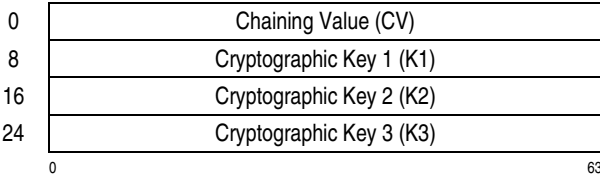
Figure 7-108. Parameter Block for KMF-TDEA-192
