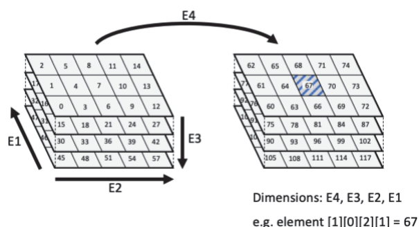
Figure 26-50. Example of a generic 4D-tensor with dimensions 2,4,3,5
