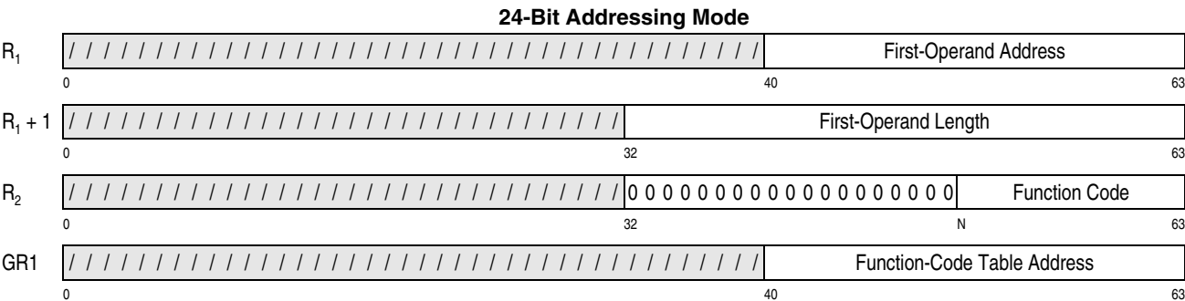
Figure 7-366. Register Contents for TRANSLATE AND TEST EXTENDED and TRANSLATE AND TEST REVERSE EXTENDED (Part 1 of 2)
