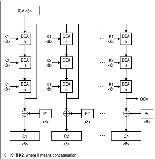
Figure 7-172. KMO-TDEA-128 Encipher Operation
