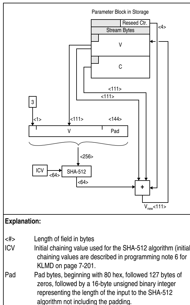
Figure 7-358. PRNO-SHA-512-DRNG Function's Generate Operation Normal Completion
