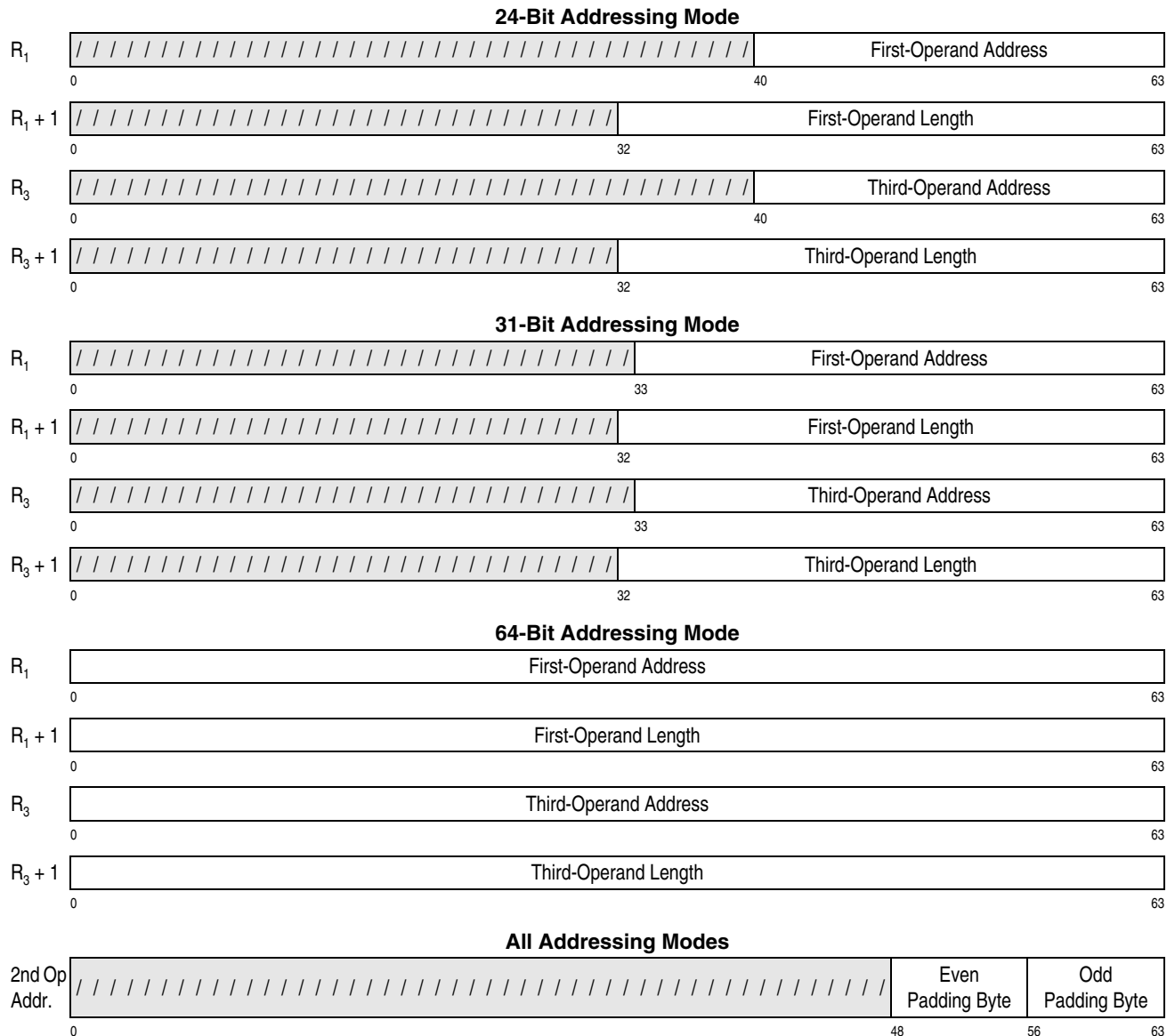
Figure 7-302. Register Contents and Second-Operand Address for MOVE LONG UNICODE
