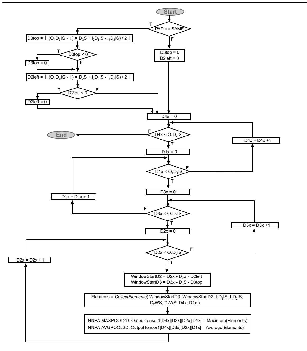
Figure 26-65. NNPA-MAXPOOL2D/AVGPOOL2D (Part 1 of 2)
