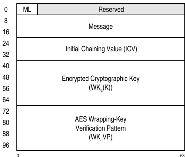
Figure 7-329. Parameter Block for PCC-Compute-Last-Block-CMAC-Using-Encrypted-AES-256
