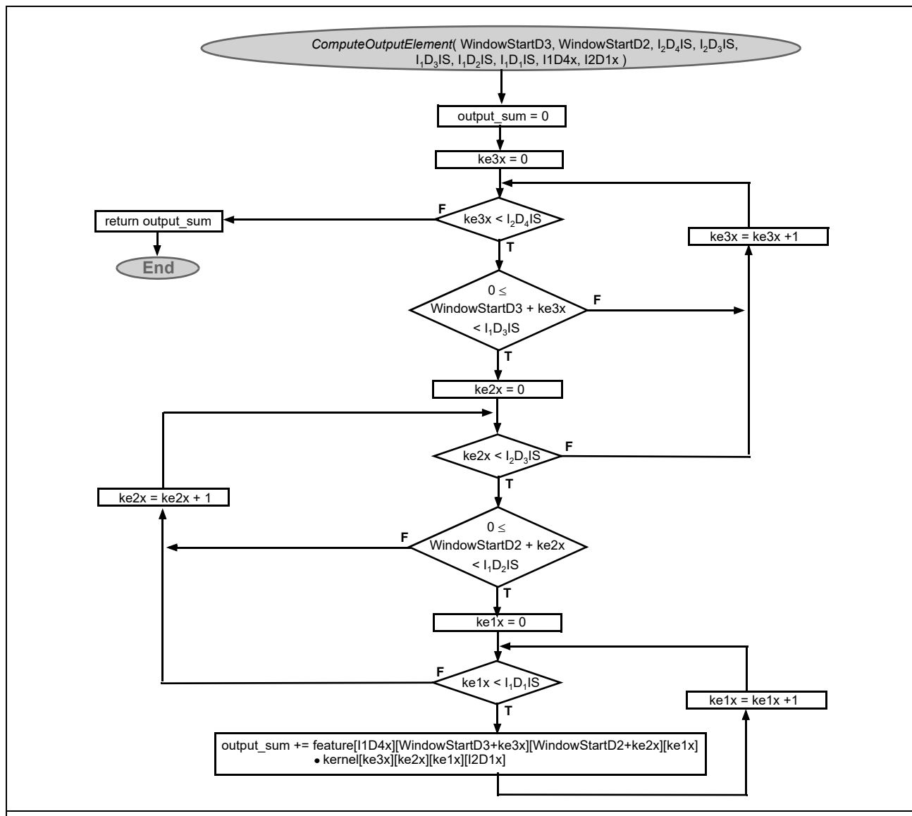
Figure 26-73. NNPA-CONVOLUTION (Part 2 of 2)
