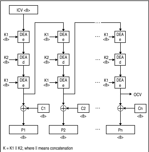
Figure 7-173. KMO-TDEA-128 Decipher Operation
