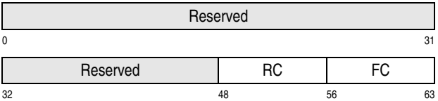
Figure 10-72. General-Register R 1 Format
