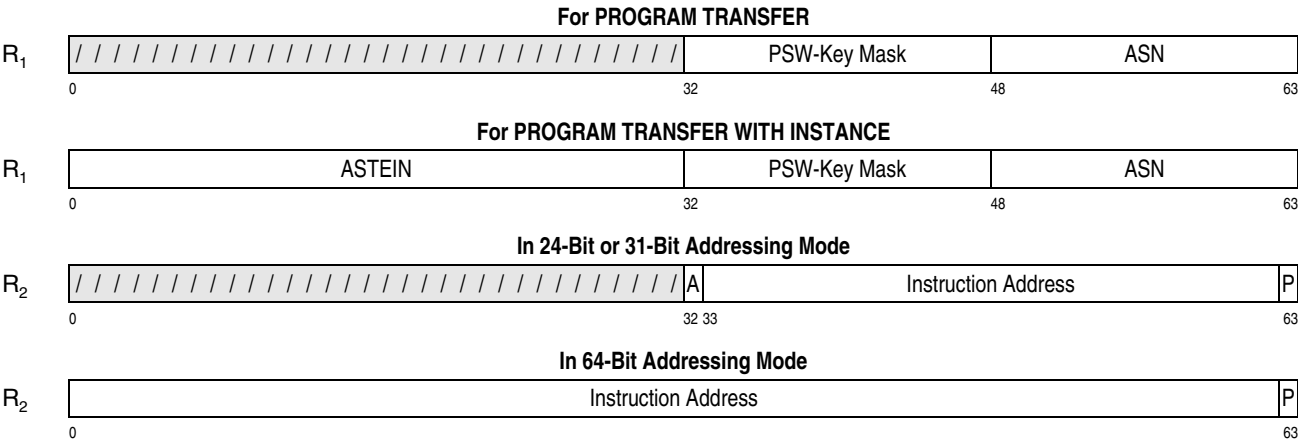
Figure 10-76. Register Contents for PROGRAM TRANSFER (WITH INSTANCE)
