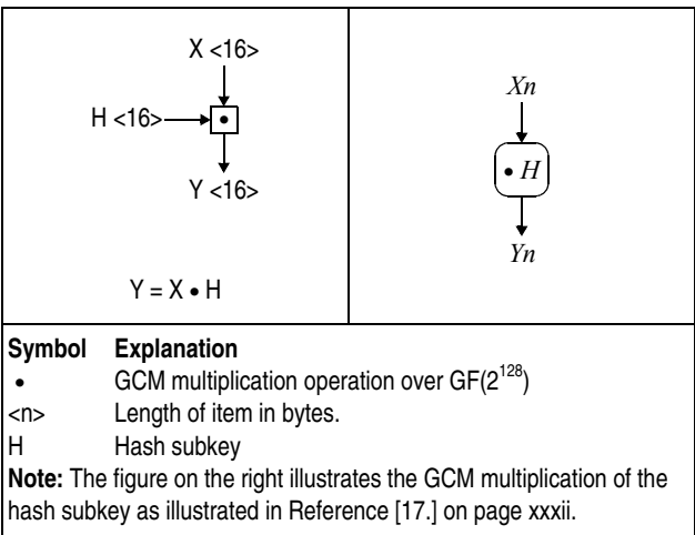
Figure 7-81. Symbols For GCM Multiplication Operation Over GF(2^{128})
