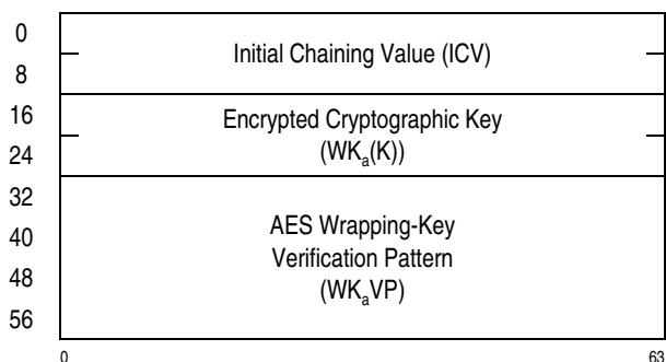
Figure 7-283. Parameter Block for KMAC-Encrypted-AES-128
