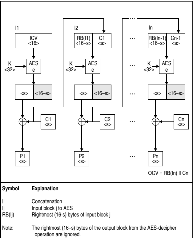
Figure 7-123. KMF-AES-256 Decipher Operation
