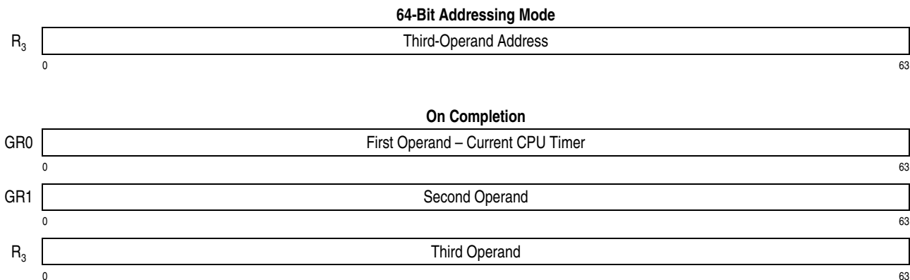
Figure 7-298. General Register Assignment for EXTRACT CPU TIME (Part 2 of 2)
