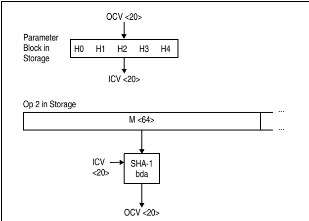
Figure 7-237. KLMD-SHA-1 Full Block (L ≥ 64)
