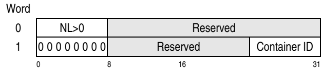
Figure 10-98. Container-Type Topology-List Entry
