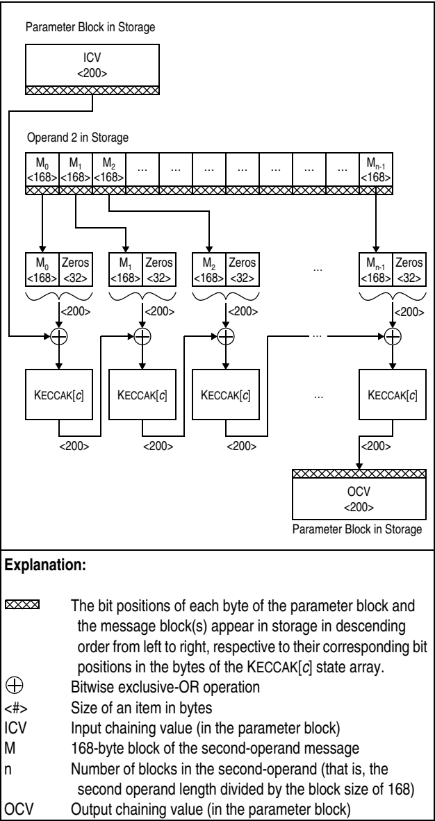
Figure 7-229. KIMD-SHAKE-128 Processing
