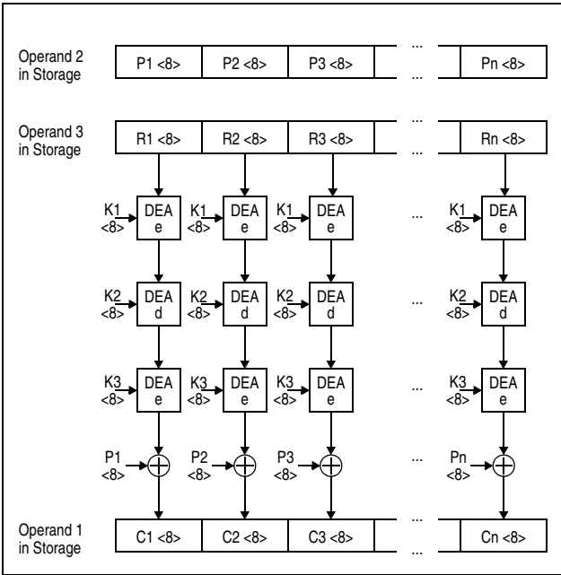
Figure 7-143. KMCTR TDEA Encipher Operation Using 192-Bit Key
