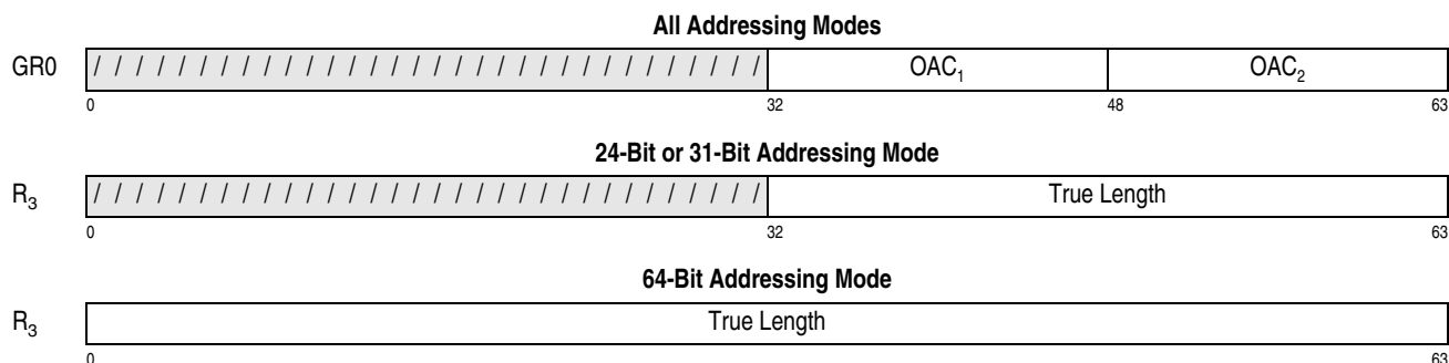
Figure 10-36. Register Contents for MOVE WITH OPTIONAL SPECIFICATIONS
