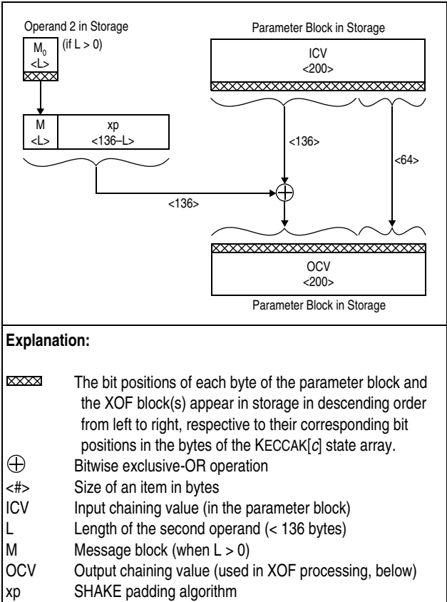
Figure 7-262. KLMD-SHAKE-256 Padding (L < 136)
