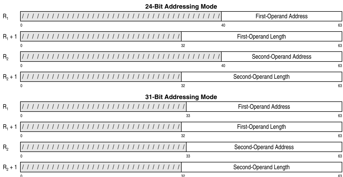
Figure 7-294. Register Contents for CONVERT UTF-32 TO UTF-16 (Part 1 of 2)
