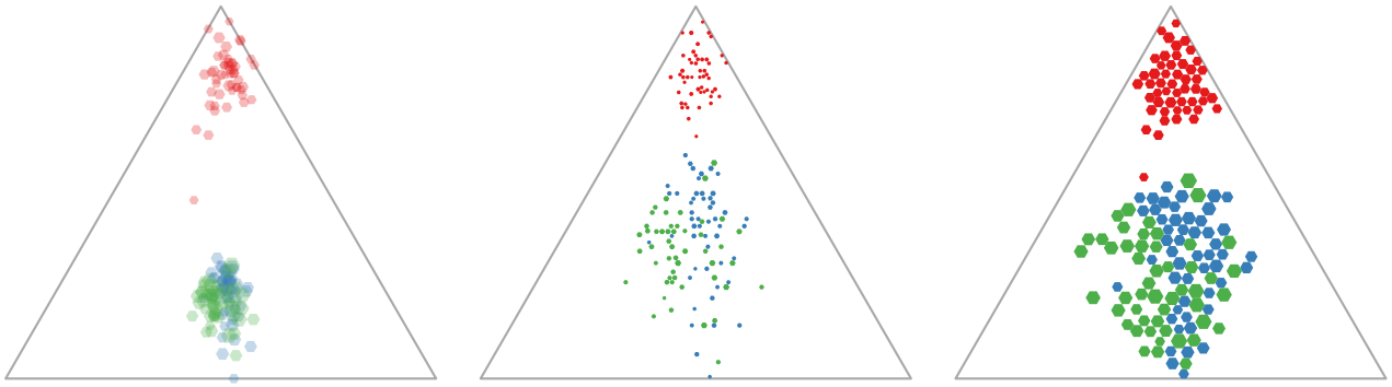
Figure 11: Left: Iris data in barycentric coordinates, each of the attributes normalized to [0, 1] . Middle: minimal displacement for hexagonal symbols and order constraints, using a regular 6-gon as \delta . Right: minimal displacement with weak order constraints.
