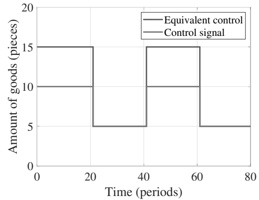
Fig. 6. Equivalent control u_{\beta eq}(k) and control signal u_\beta(k) .
