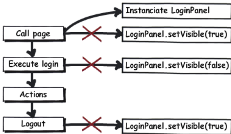
Listing 7:
