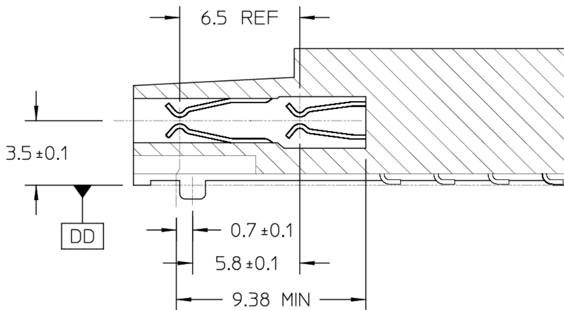
SECTION Z-Z
