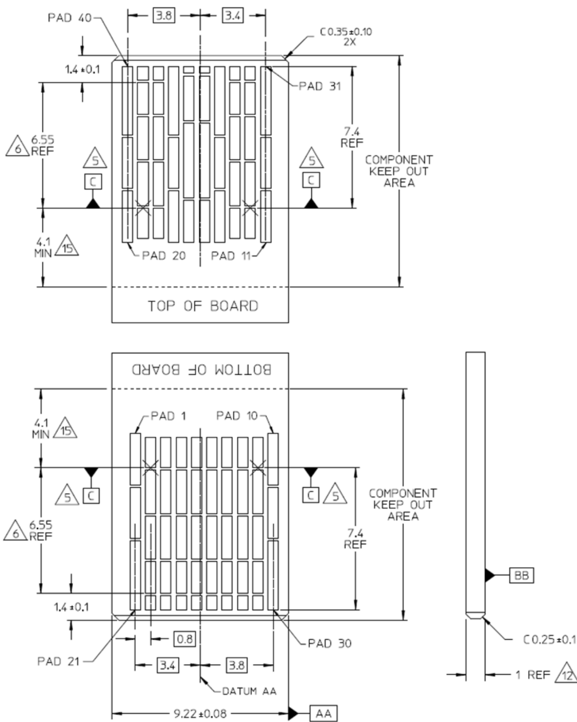
Figure 40: Module paddle card dimensions
