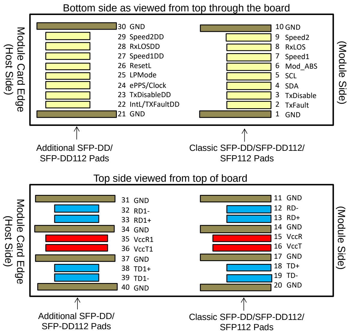
Figure 3: SFP-DD/SFP-DD112 module pad layout
