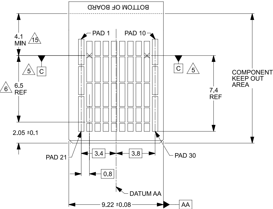
Figure 50: Improved module paddle card dimensions
