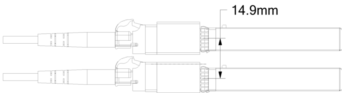
7 Figure 32: Minimum vertical port pitch
