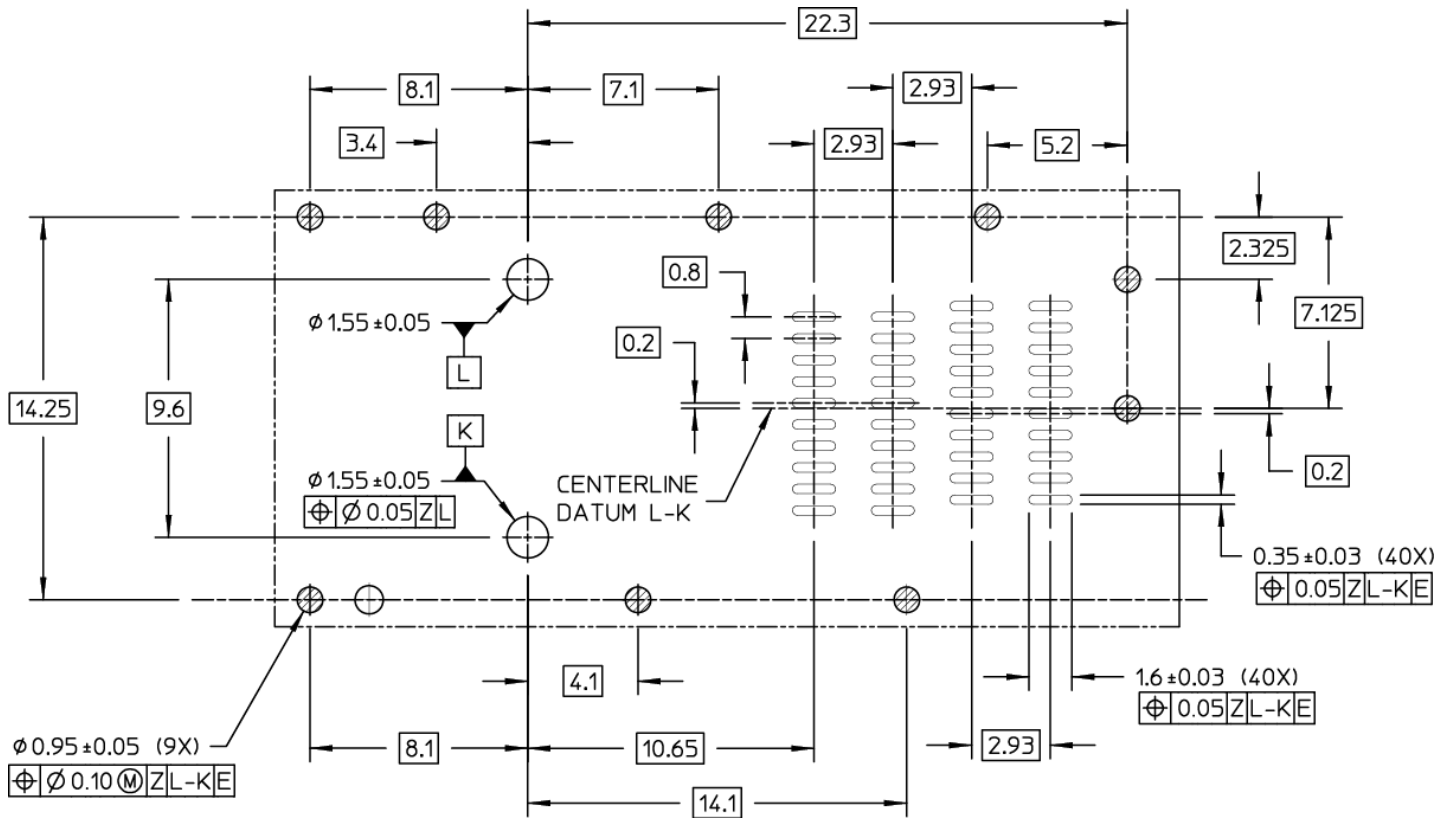
DETAIL 1
