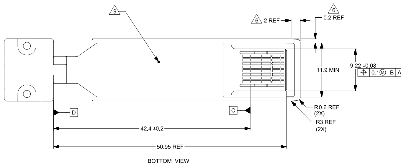
Figure 49: SFP-DD112 Module Bottom View Details
