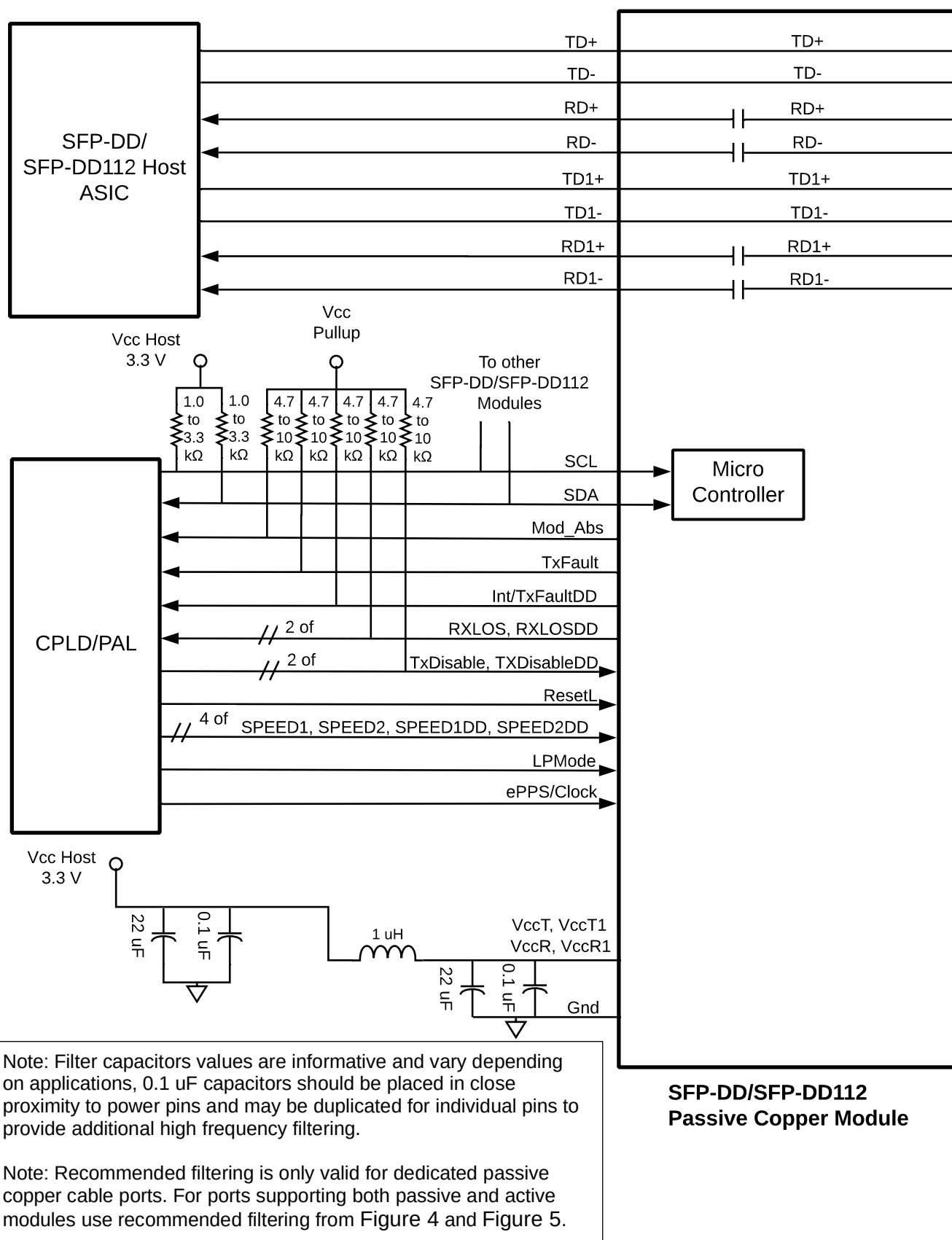
Figure 6: Example SFP-DD/SFP-DD112 Host Board Schematic for passive copper cables
