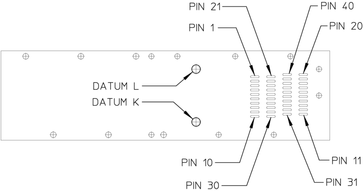
Figure 48: Host PCB Mechanical Layout
