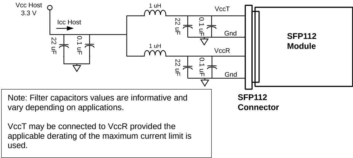
4 Figure 24: SFP112 Recommended Host Board Power Supply Filtering 5 6 7
