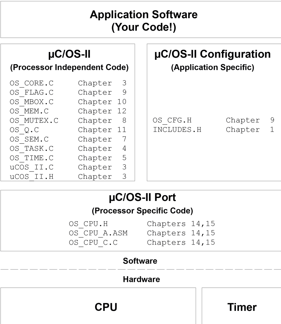
Figure - Figure 3.1 μC/OS-II File Structure
