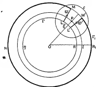
The contribution of \sum j_{p,q}^{\gamma} .
