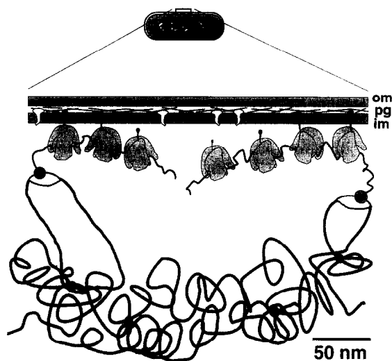
Fig. 2. Schematic representation of co-transcriptional translocation of membrane proteins along a 300-nm stretch of the cell envelope. Dimensions of cell envelope, ribosomes and RNA polymerase were taken from Woldring and Nanninga [34]. Transmembrane proteins (white), involved in the synthesis of the peptidoglycan layer (pg) between the outer membrane (om) and the cytoplasmic membrane (im), may hinder lateral diffusion of proteins (grey) that are being translocated. These exert a pulling force on supercoiled DNA, held in a solenoidal conformation by DNA binding proteins (black circles). If all envelope proteins would be co-transcriptionally translocated, a rough estimate (see text) shows that a cell would need the continuous action of 1 translocation site per 40 \times 40 nm surface to double its mass.
