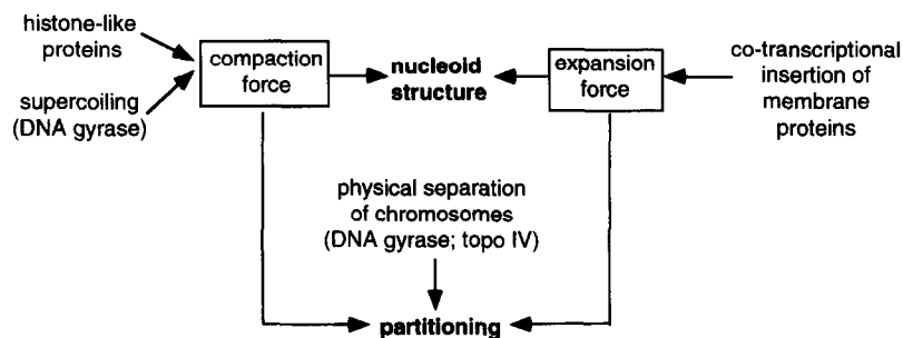
Fig. 3. Diagram illustrating the two forces proposed to determine the structure of the nucleoid and to influence nucleoid partitioning.
