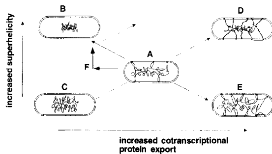
Fig. 4. The wild-type situation (A) and four theoretical states of nucleoid structure as determined by supercoiling and co-translational protein export. Horizontally and vertically, the two relevant driving forces are indicated, i.e., as resulting from coupled transcription translation translocation and from DNA supercoiling respectively. Arrows A → B and A → E indicate the resultant (in the vectorial sense) balanced forces that compact or expand, respectively. The resultant in the direction C-A-D (dashed arrow) indicates improved partitioning. (F) represents a rescue experiment (see text).
